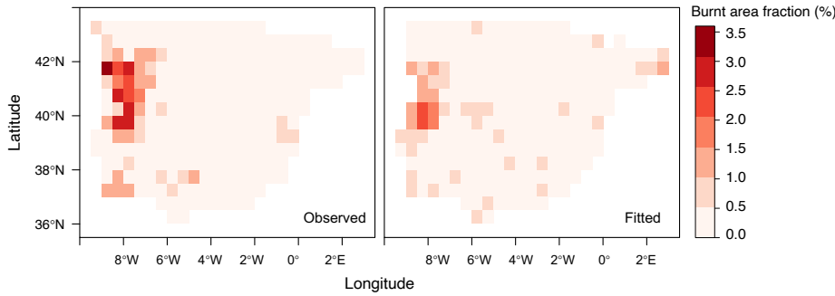
Figure 3. Mean (over 16 years) of observed (left) and fitted (right) values of burnt area fraction.
