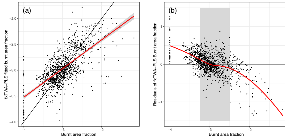
Figure 4. The fitted plot and residual plot of TWA-PLS method, with fx correction. Panel (a) is the reconstructed burnt area using the last significant number of components, here is 4. The x-axis is the burnt area fraction derived from charcoal data; the y-axis is the burnt area fraction reconstructed from pollen data using TWA-PLS with fx correction. The 1: 1 line is shown in black; the linear regression line is shown in red, to show the degree of overall compression. Panel (b) shows the residuals of reconstructed burnt area fraction using the last significant number of components. The x-axis is the burnt area fraction derived from charcoal data; the y-axis is the residual of burnt area reconstruction using TWA-PLS with fx correction. The zero line is shown in black; the locally estimated scatterplot smoothing is shown in red, to show the degree of local compression; the low compression zone is shown in grey shading.
