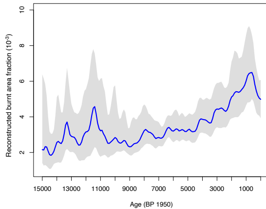
Figure 6. Composite curve of reconstructed burnt area using fxTWA-PLS, using the lofit() function with half-width = 300, number of bootstrap samples = 1000. The locally estimated scatterplot smoothing is shown in blue. The upper and lower 95th-percentile confidence intervals are shown in grey.
