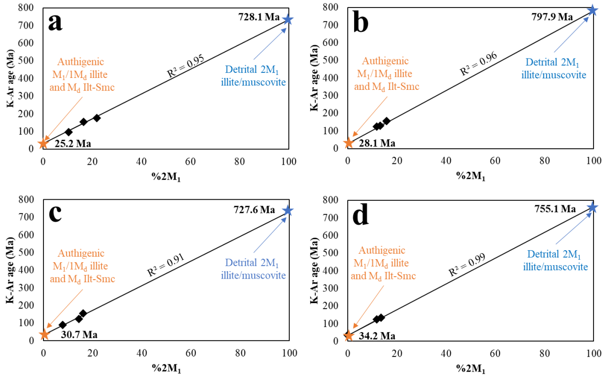
Figure 5: Crystallization ages of detrital 2M 1 illite/muscovite and of authigenic 1M d /1M illite and illite-smectite (Ilt-Smc) from the Valley of Lakes, calculated for sediments collected from (a) TAT section (~90.5 m), (b) TGR-C section (~78.0 m), (c) SHG-D section (~55.5 m) and (d) TGR-AB section (~35.0 m) using illite polytype quantification and K-Ar age systematics of different grain size sub-fractions (from left to right: < 1 μm, 1-2 μm and 2-10 μm).
