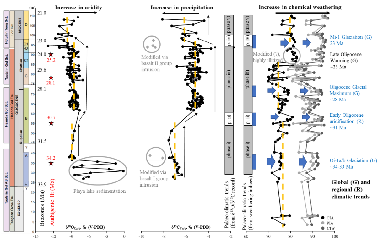
Figure 8: Lithostratigraphic framework of the sediments from the Valley of Lakes (Mongolia, Central Asia) showing the biozonation (modified after Harzhauser et al., 2017) and formation ages of authigenic illitic (Ilt) phases obtained in this study (red asterisks), as well as soil carbonate \delta^{18}\text{O} and \delta^{13}\text{C} isotope profiles and shifts in the silicate mineral-derived chemical weathering indicators. Note that these hydroclimate proxies are inversely correlated and follow long-term trends (indicated by orange dashed lines) in aridification or gain of humidity in this region (indicated by black arrows). Increased chemical weathering degrees (highlighted with blue bars and blue arrows) coincide with glaciation events documented in time-equivalent marine deep-sea deposits (Zachos et al., 2001; Gallagher et al., 2020). Samples and intervals outlined with grey circles are most likely modified due to the flows of the basalt I and II groups or local strong illitization, and are therefore excluded from the palaeo-climatic interpretation.
