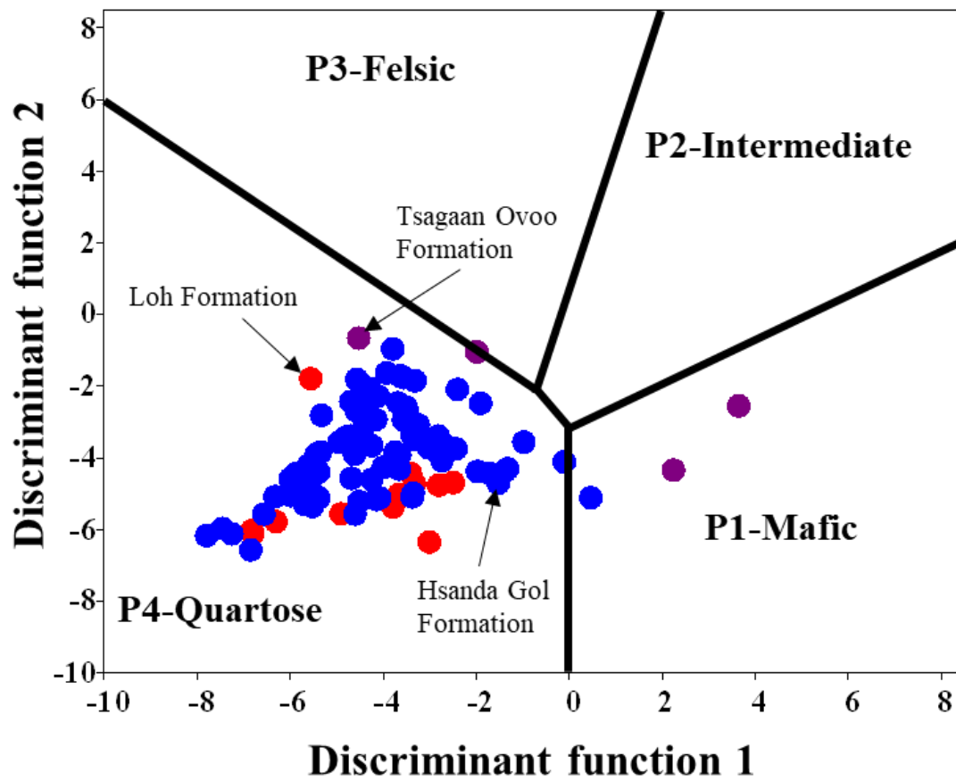
1000 Figure 7: Discrimination plot of discriminant function 1 and 2 indicating a narrow provenance 1001 range (mainly type P4-quartzose) for the sediments from the Valley of Lakes, Mongolia.
