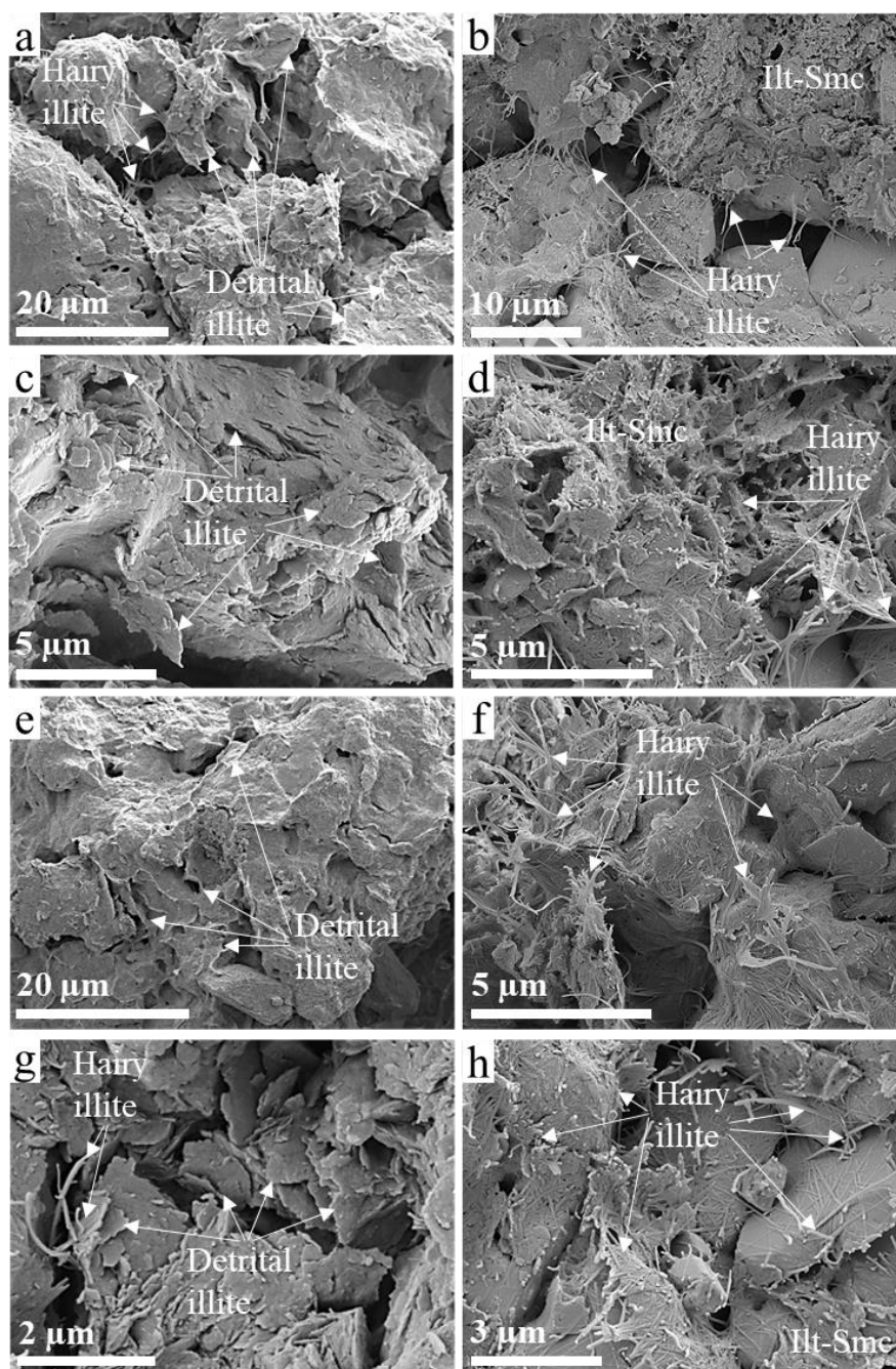
Figure 4: Secondary electron images of partly calichized and illitized silty to sandy deposits from the of the Oligocene Hsanda Gol Formation, Valley of Lakes, collected from (a-b) TAT section (~90.5 m), (c-d) TGR-C section (~78.0 m), (e-f) SHG-D section (~55.5 m) and (g-h) TGR-AB section (~35.0 m). The detrital illite/muscovite (left panel) occurs as coarse, rounded or pseudo-hexagonal platelets, whereas authigenic illite-smectite (Ill-Smc) and hairy illite (right panel) appear either as fine, flaky to irregular particles or as long, but thin laths and fibers, both covering detrital grains or growing into the open pores.
