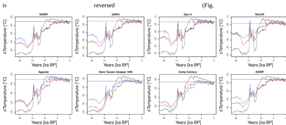
Figure 5: Comparison of temperature anomalies from current (1950-1990) for the CHELSA-TraCE21k time series data (blue), the TraCE21k data (red), and the temperature reconstructions from ice cores (black) for 8 sites across Greenland. The grey horizontal line indicates the current observed temperature during the period 1981-2010 from CHELSA V2.1. data. Temperatures are plotted as anomalies from the current temperature recorded at the respective location of the ice cores.
