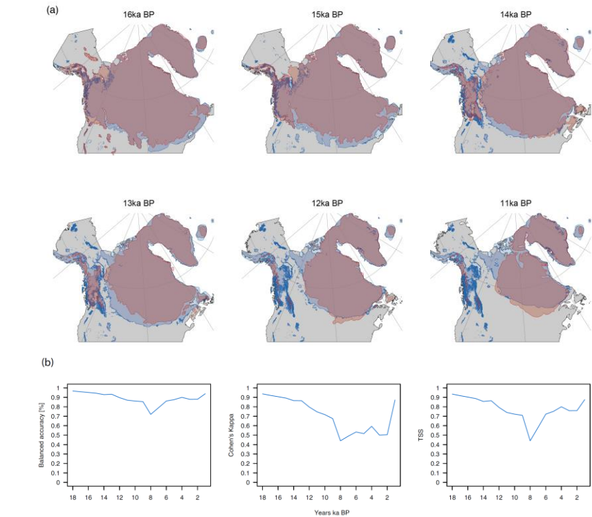
Figure 6: a.) Comparisons of estimated glacial extents of the Laurentide ice sheet from 16k BP to 11k BP. Blue delineates the interpolated ice sheet extent from CHELSA-TraCE21k, and red shows the estimated extent from (Dyke et al., 2003). While the retreat of the main Laurentide ice sheet is similar in both estimations, the Cordilleran Ice sheet covering the Rocky Mountains, retreats faster in the estimations by (Dyke et al., 2003), compared to CHELSA-TraCE21. b.) Performance comparison using three different metrics (Balanced accuracy, Cohen's Kappa, and True Skill Statistic) from a comparison of CHELSA-TraCE21k and Dyke et al. 2003.
