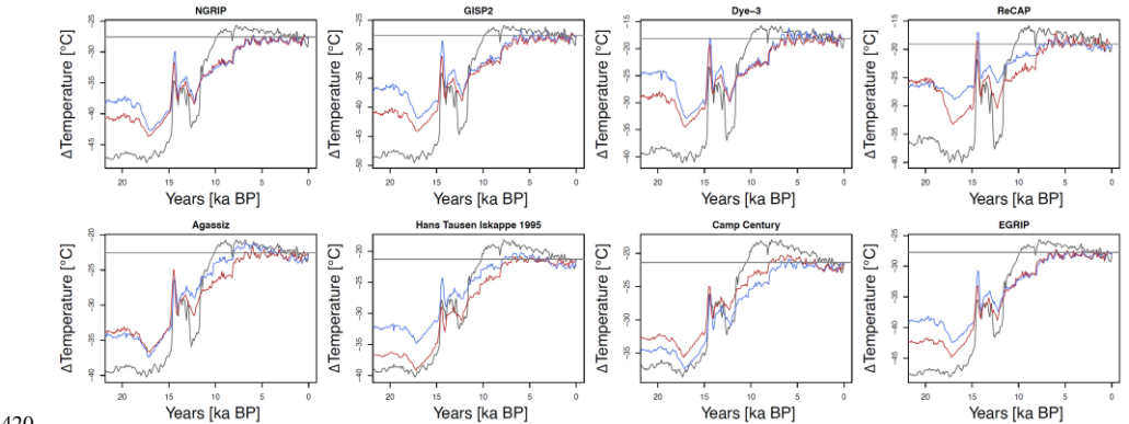
420 Figure 5: Comparison of temperature anomalies from current (1950-1990) for the CHELSA-TraCE21k time series data (blue), the TraCE21k data (red), and the temperature reconstructions from ice cores (black) for 8 sites across Greenland. The grey horizontal
