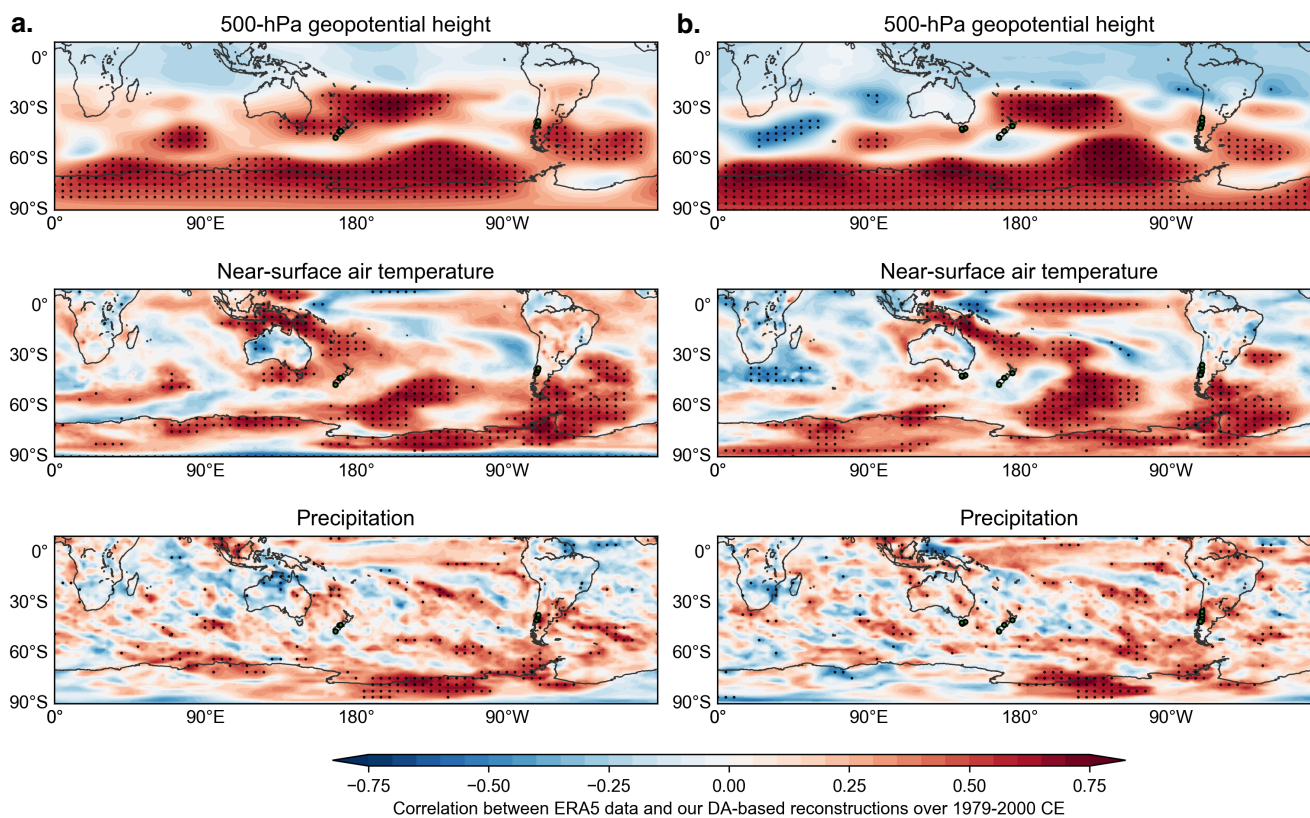
Figure 2. Pearson correlation coefficient between the reconstructed and ERA5 geopotential height at 500 hPa, near-surface air temperature or cumulative precipitation over 1979–2000 CE for the TIC-MDN (a) and TIC-reg (b) experiments (see Sect. 3 and Table 1 for details on the experiments). The green dots indicate the localization of the assimilated tree-ring width records. The black dots indicate a significant correlation coefficient at the 95% confidence level.
