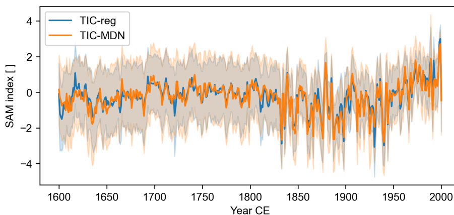
Figure 10. Z-scored (relative to 1901–2000 CE) TIC-reg (in blue) and TIC-MDN (in orange) reconstructed SAM index over 1600–2000 CE (Table 1). The uncertainty associated with each reconstruction is represented by the shaded areas.
