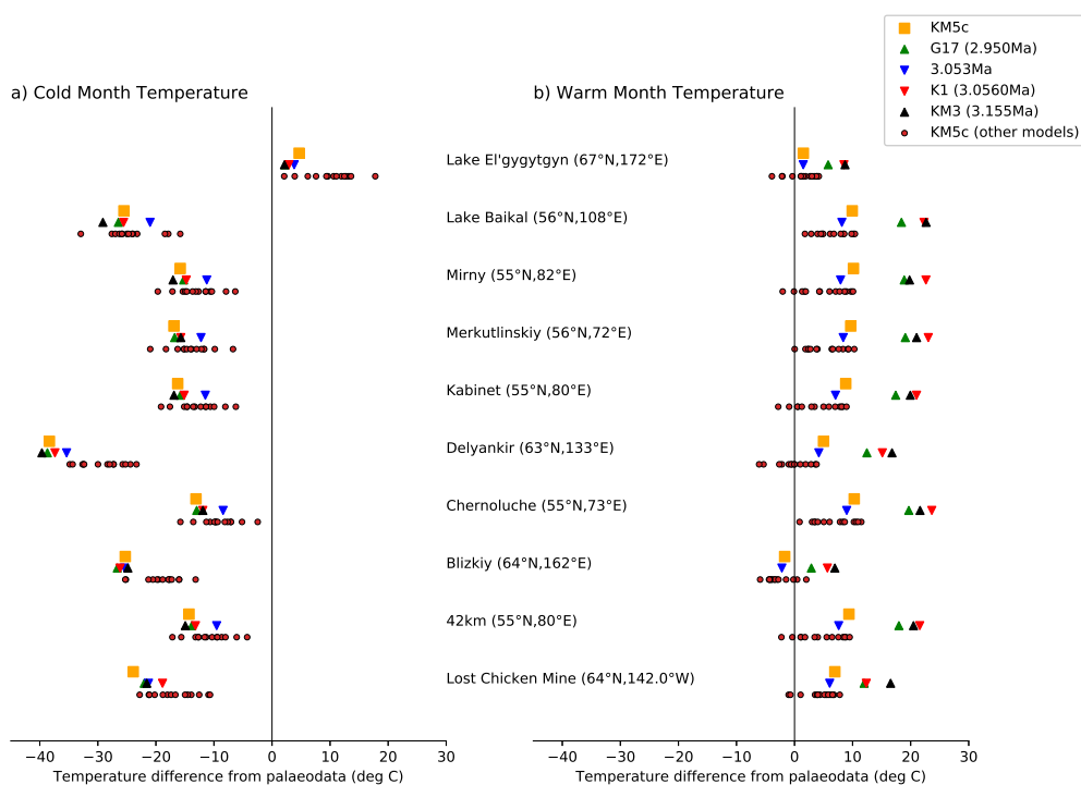
Figure 6. Shows the difference between the modelled temperature and the palaeodata at KM5c (Lake Baikal and Lake El'gygytgyn) and other late Pliocene sites. HadCM3 simulations with a range of different orbital configurations are shown by the square and triangles. The KM5c simulation for other models is shown by the circles.
