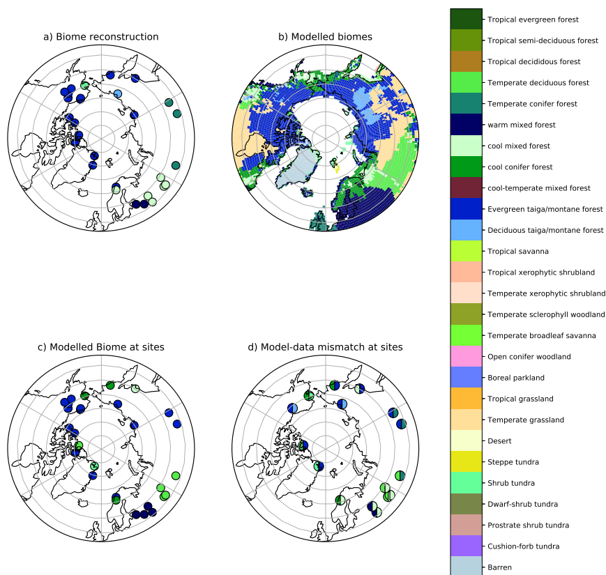
Figure 5. a) The reconstructed biomes from Salzmann et al. (2008). b) the modelled biomes, obtained by using the PlioMIP2 MMM to drive the BIOME4 model. c) The modelled biomes in (b), at the locations where data is available. d) locations where the reconstructed biomes do not match the modelled biome. The modelled biome is the left of the semicircle, the reconstructed biome is the right of the semicircle.
