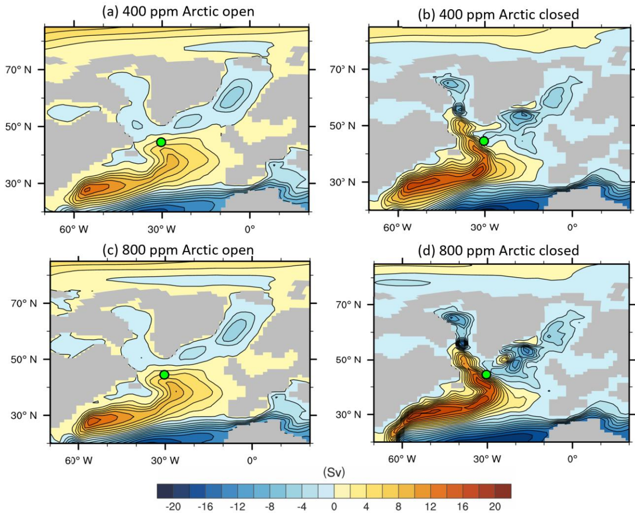
910 Figure 8: Barotropic streamfunctions illustrating the horizontal circulation (positive = clockwise) for the Arctic open (a, c) and the Arctic closed run (b, d) for atmospheric CO 2 concentrations of 400 ppm (a,b) and 800 ppm (c,d). The contour interval is 2 Sv. Note the modified and intensified subtropical and subpolar gyre systems in the Arctic closed experiment and the critical position of Site 647 at their boundaries.
