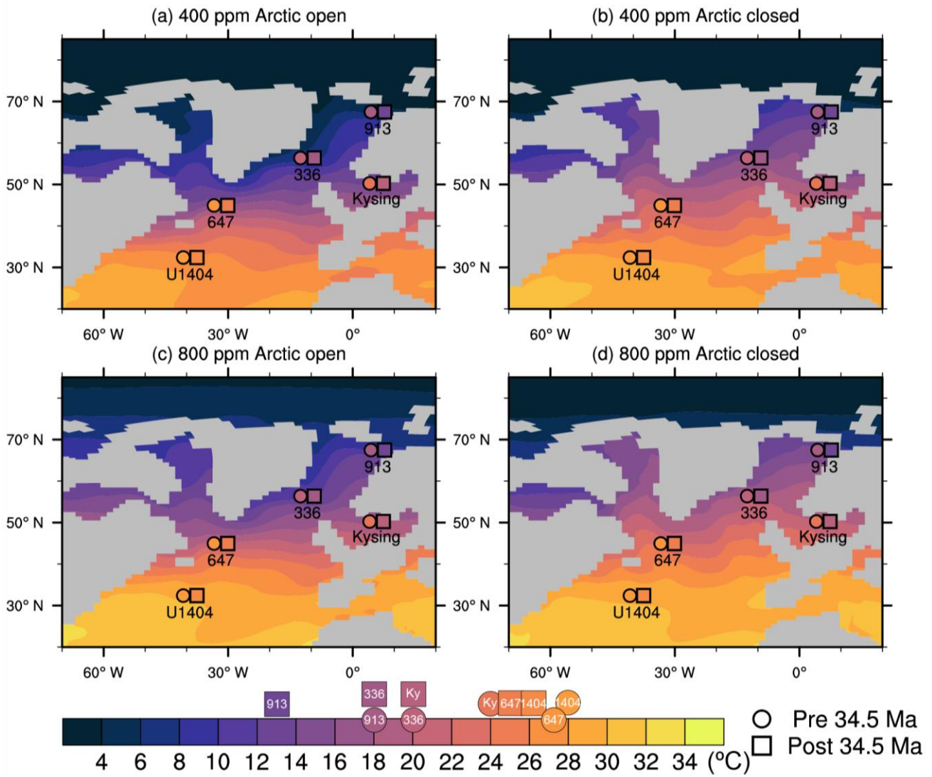
Figure 6: Comparison of model temperatures in the four simulations in the North Atlantic with late Eocene (circles; pre 34.5 Ma) and early Oligocene (squares; post 34.5 Ma) proxy data. Contours show the modelled annual mean SST for the Arctic open (a, c) and the Arctic closed run (b, d) for atmospheric CO 2 concentrations of 400 ppm (a,b) and 800 ppm (c,d). The coloured circles show the proxy data averaged between 34.5 and 37 Ma (late Eocene) and the coloured squares show the proxy data averaged between 34.5 and 32 Ma (early Oligocene).
