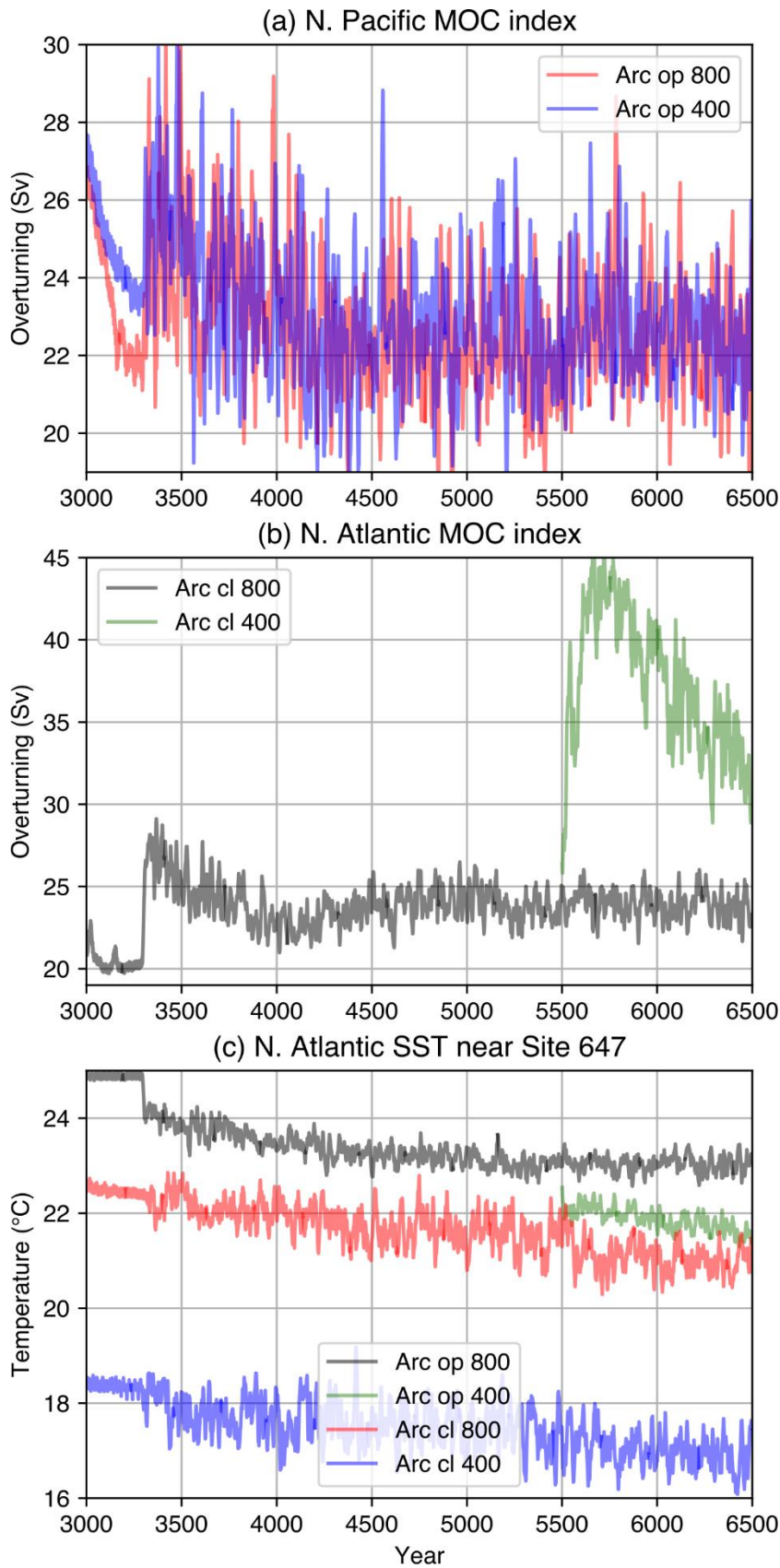
880 Figure 5: Time series of the North Pacific meridional overturning circulation (MOC) index (a), the North Atlantic MOC index (b), and the SST averaged over a 5^{\circ} \times 5^{\circ} box around core site 647 in the four model simulations.
