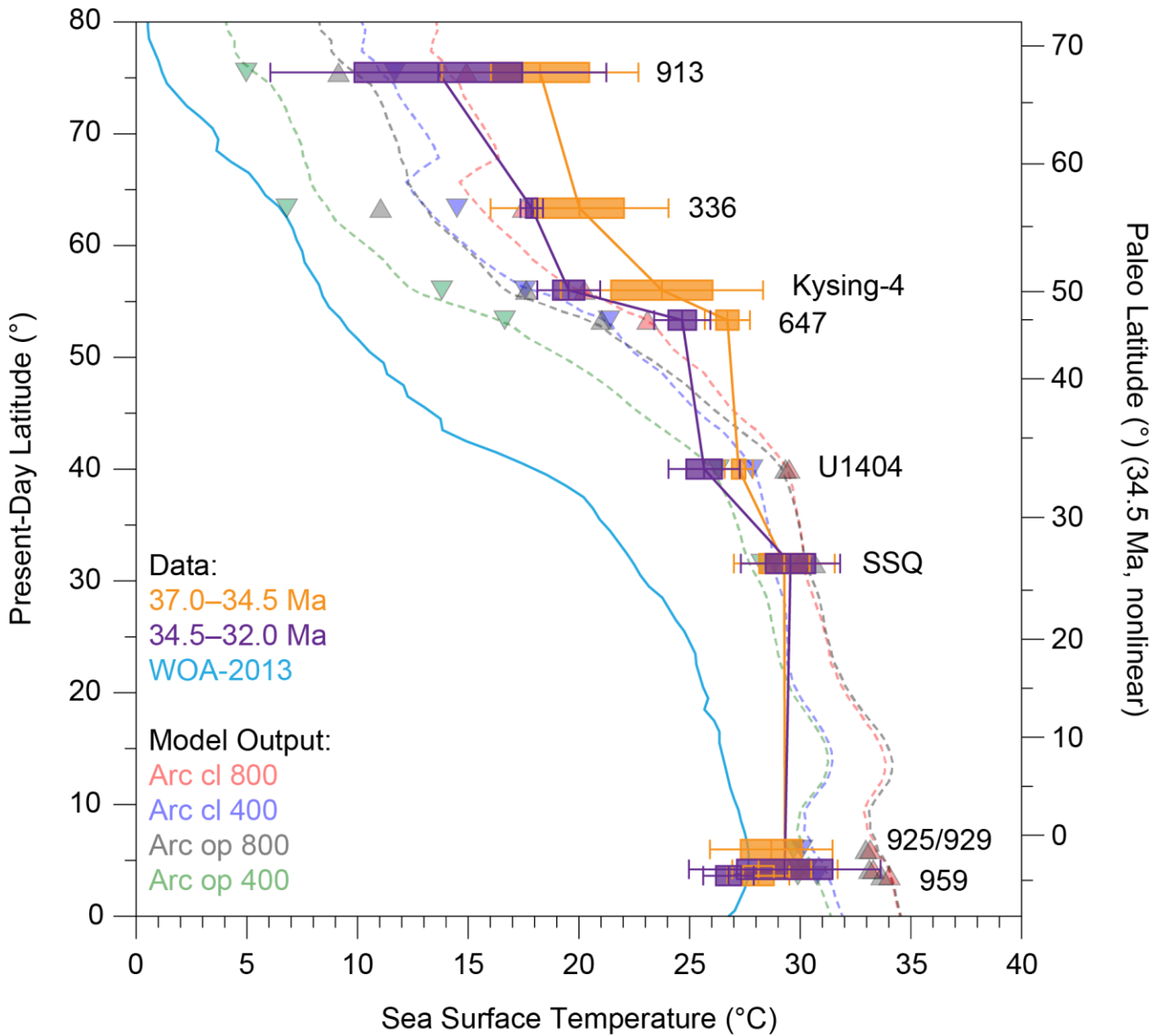
Figure 4: Data-model comparison of latitudinal SST gradients for the “Eocene” (>34.5 Ma, orange bars and solid lines) and “Oligocene” (<34.5 Ma, violet bars and solid lines) states to the four different model simulations. The dashed lines show the zonal average SSTs at that latitude and the triangles show the site specific temperatures in the simulations. The 1 and 2 sigma error bars are indicated around the data points and on the left of the figure in solid blue is the zonally average present-day Atlantic SST from the World Ocean Atlas (Boyer et al., 2013). Model paleolatitudes (right hand axis) are shifted with respect to present-day latitudes of the data (site and WOA data, left hand axis) by the average offset of -7.0^\circ (error: \pm 1.5^\circ ) for the sites considered.
