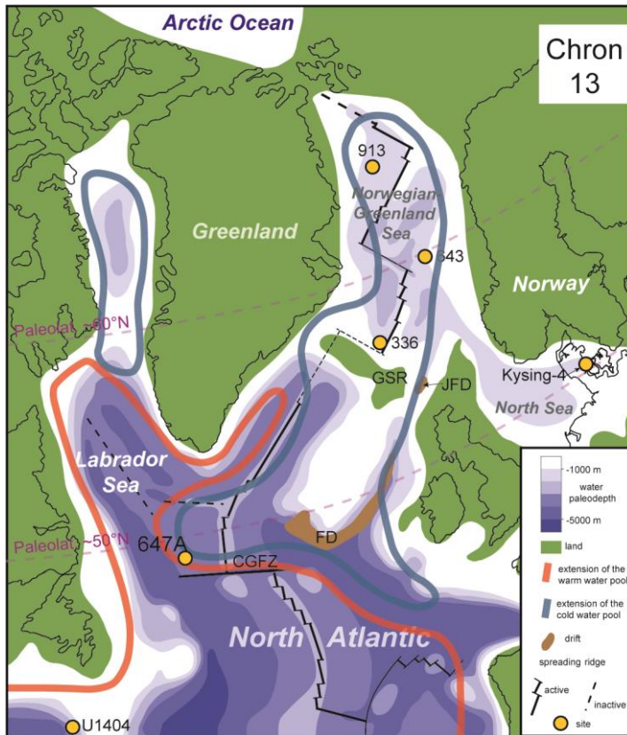
840 Figure 1: The late Eocene (magnetic polarity Chron 13; 33.705–33.157 Ma (GTS2012)) location of Site 647 (ODP Leg 105) and other sites studied for temperature proxies (pollen in ODP 913B, ODP 643, ODP 985 (Eldrett et al., 2009); alkenones in DSDP 336, ODP 913B and IODP U1404 (Liu et al., 2009, 2018); GDGTs in Kysing-4 (Śliwińska et al., 2019)) referred to in the text. The paleogeographic map is modified after Arthur et al., (1989), Piepjohn et al., (2016), Śliwińska et al., (2019) and references therein. Abbreviated oceanic features identified are: 845 the Feni Drift (FD)(Davies et al., 2001), the Judd Falls Drift (JFD) (Hohbein et al., 2012), Greenland–Scotland Ridge (GSR), and Charlie-Gibbs Fracture Zone (CGFZ).
