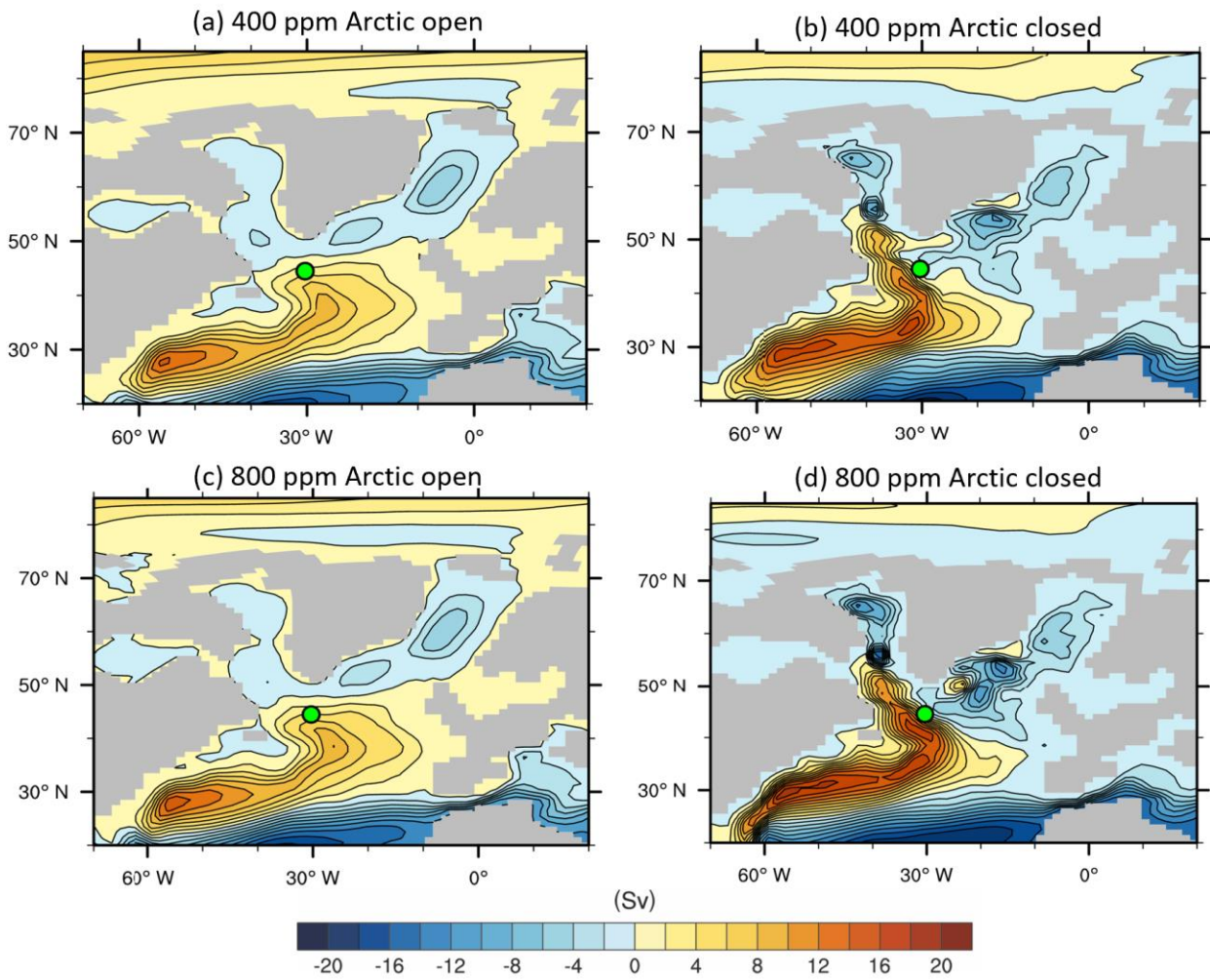
ϕ20 Figure 78: Barotropic streamfunctions illustrating the horizontal circulation (positive = clockwise) for the Arctic open (a, c) and the Arctic closed run (b, d) for atmospheric CO 2 concentrations of 400 ppm (a,b) and 800 ppm (c,d). The contour interval is 2 Sv.
