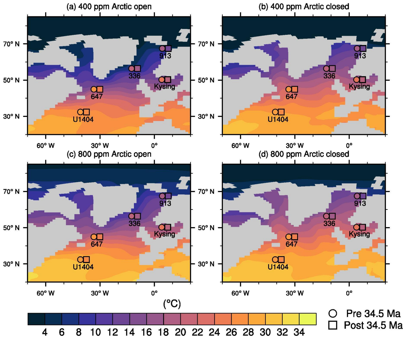
Figure 56: Comparison of model temperatures in the four simulations in the North Atlantic with Late Eocene (circles) and Early Oligocene (squares) proxy data. Contours show the modelled annual mean SST for the Arctic open (a, c) and the Arctic closed run (b, d) for atmospheric CO 2 concentrations of 400 ppm (a,b) and 800 ppm (c,d). The colored circles show the proxy data averaged between 34.5 and 37 Ma (a, b) and between 34.5 and 32 Ma (c, d).
