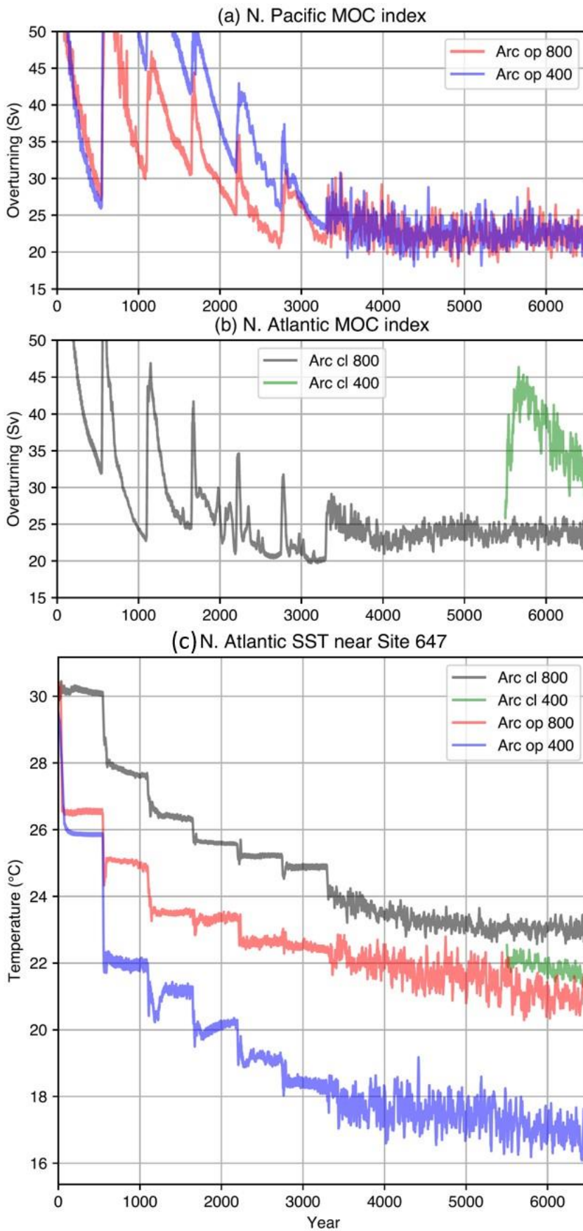
Figure 5: Time series of the North Pacific meridional overturning circulation (MOC) index (a), the North Atlantic MOC index (b), and the SST averaged over a 5°x5° box around core site 647 in the four model simulations.
