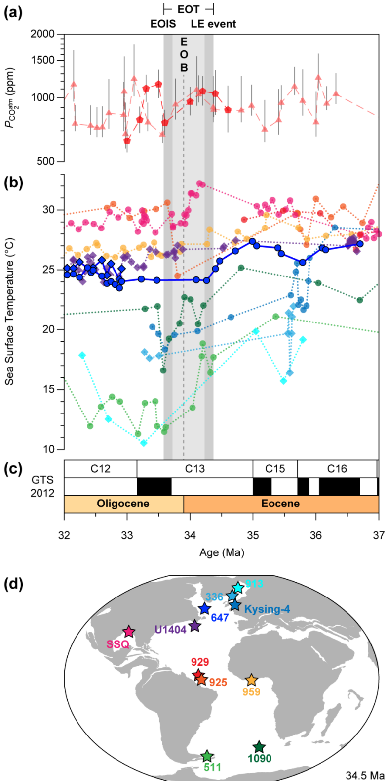
875 Figure 3: SST evolution across the EOT in the Atlantic Ocean. a) Reconstructed P_{\text{CO}_2^{\text{atm}}} based on planktonic foraminiferal \delta^{11}\text{B} (pentagons) (Pearson et al., 2009) and phytoplankton alkenone \delta^{13}\text{C} (triangles) (Pagani et al., 2011; Zhang et al., 2013). The effect of P_{\text{CO}_2^{\text{atm}}} on radiative forcing scales logarithmically. b) Newly generated and published (Cramwinckel et al., 2018; Houben et al., 2019; Inglis et al., 2015; Liu et al., 2018, 2009; Śliwińska et al., 2019; Wade et al., 2012) reconstructed SSTs based on U_{37}^{kl} (diamonds) and \text{TEX}_{86}^{\text{H}} (circles). All 880 ages are converted into the GTS2012 (Vandenberghe et al., 2012). c) Magneto- and chronostratigraphy based on the GTS2012 (Vandenberghe et al., 2012). d) Paleogeography at 34.5 Ma ( https://www.odsn.de/ ) with color- coded site locations of the SST records shown in panel B. SSQ stands for St. Stephen's Quarry.
