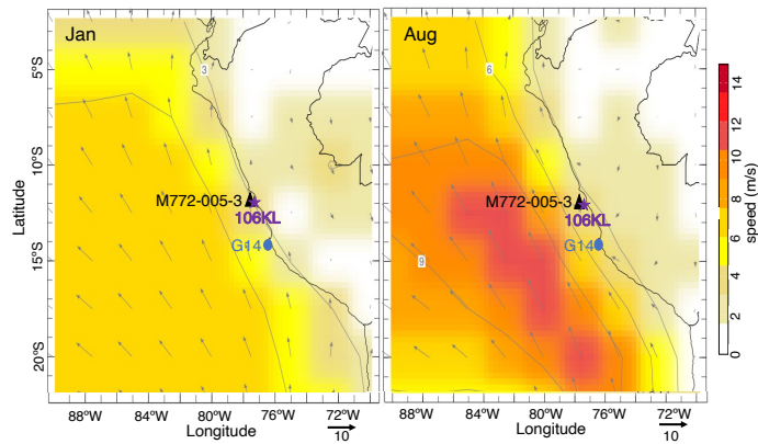
179 180 Figure 1. (A) Location of the sampling of the sediment cores M772-005-3, 106KL and G14 core. Average wind speed (m/s) at 1000 181 hPa in January and August ( http://iridl.ldeo.columbia.edu ).
