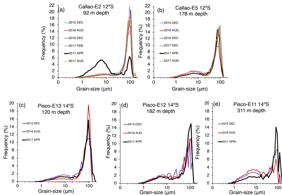
247 248 Figure 2. Grain-size distribution of surface sediments at the Callao (a, b) and Pisco stations (c, d, e).
