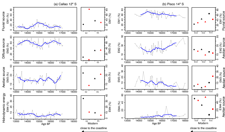
367 Figure 6. Variations in the contribution of the grain size end-members from marine cores and surface sediments in Callao (a) and 368 Pisco (b). The modern period is represented by the mean end-member contribution of surface sediments collected during normal 369 conditions (black symbols) and Coastal El Niño April 2017 event (red symbols).
