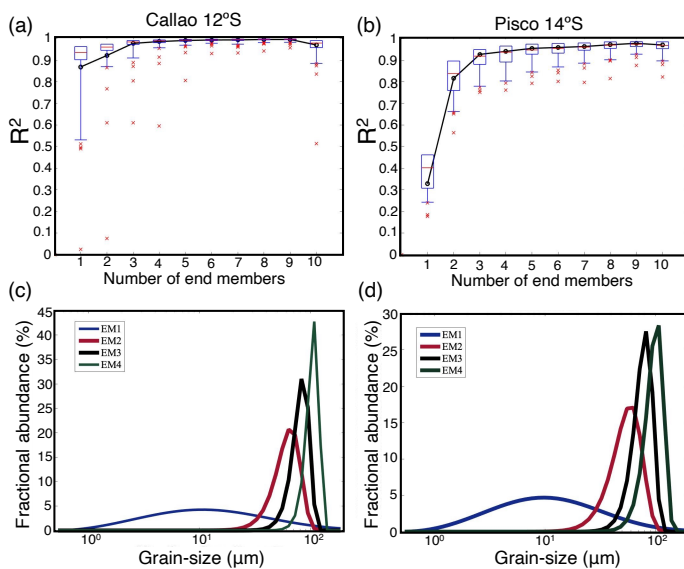
268 269 Figure 4. Coefficient of determination ( r^2 ) as a function of the number of end members chosen to model the observed grain-size 270 distribution in Callao (a) and Pisco (b). Grain size distribution of the four end-members in Callao (c) and Pisco (d).
