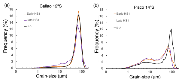
255 256 Figure 3. Mean grain-size distribution by climatic period in Callao (a) and Pisco (b).
