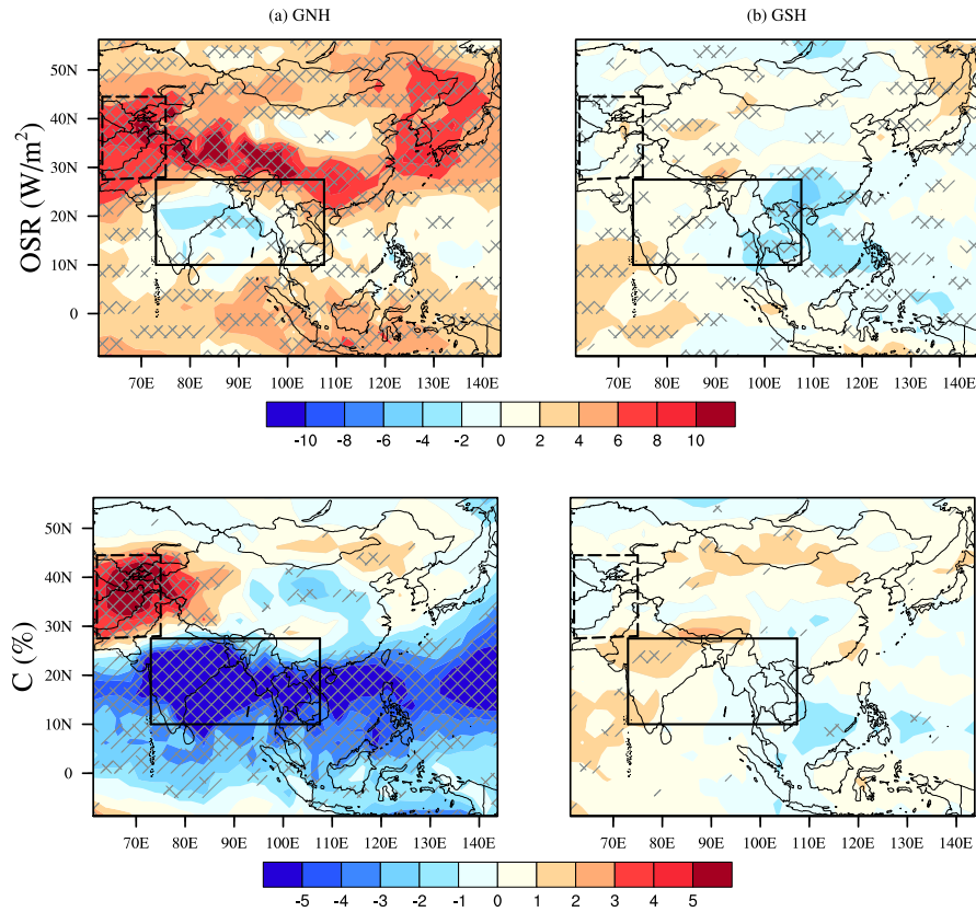
Figure 10. Spatial distribution of top of the atmosphere outgoing shortwave radiation (TOA OSR, \text{W m}^{-2} , top) in full sky and cloud area fraction ( C , %, bottom) anomalies in the eruption year with respect to the mean of five years before the eruption. The solid and dashed black box indicates the relatively wettest area (RWA) and relatively driest area (RDA), respectively. The gray slashes and cross signs indicate the significant results at the 95% and 99% confidence level.
