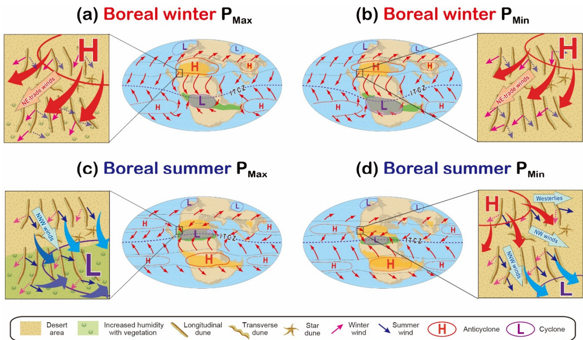
Figure 4: Schematic illustrations of orbital and seasonal changes in Pangaeian atmospheric pressure pattern and inferred dune alignments in western US during the eccentricity-modulated precession maximum (P Max ; a, c) and minimum (P Min ; b, d). Orbital-scale changes in pressure pattern are based on climatic model results (Winguth and Winguth, 2013). Seasonal changes in wind regimes are indicated as pink (boreal winter) and blue (boreal summer) arrows. During the eccentricity-modulated precession maximum, the continental low-pressure system in the boreal summer was likely reduced by a few hPa relative to the eccentricity-modulated precession minimum in response to the increase in surface temperature (Winguth and Winguth, 2013). Increased moisture and vegetation cover likely 285 290
