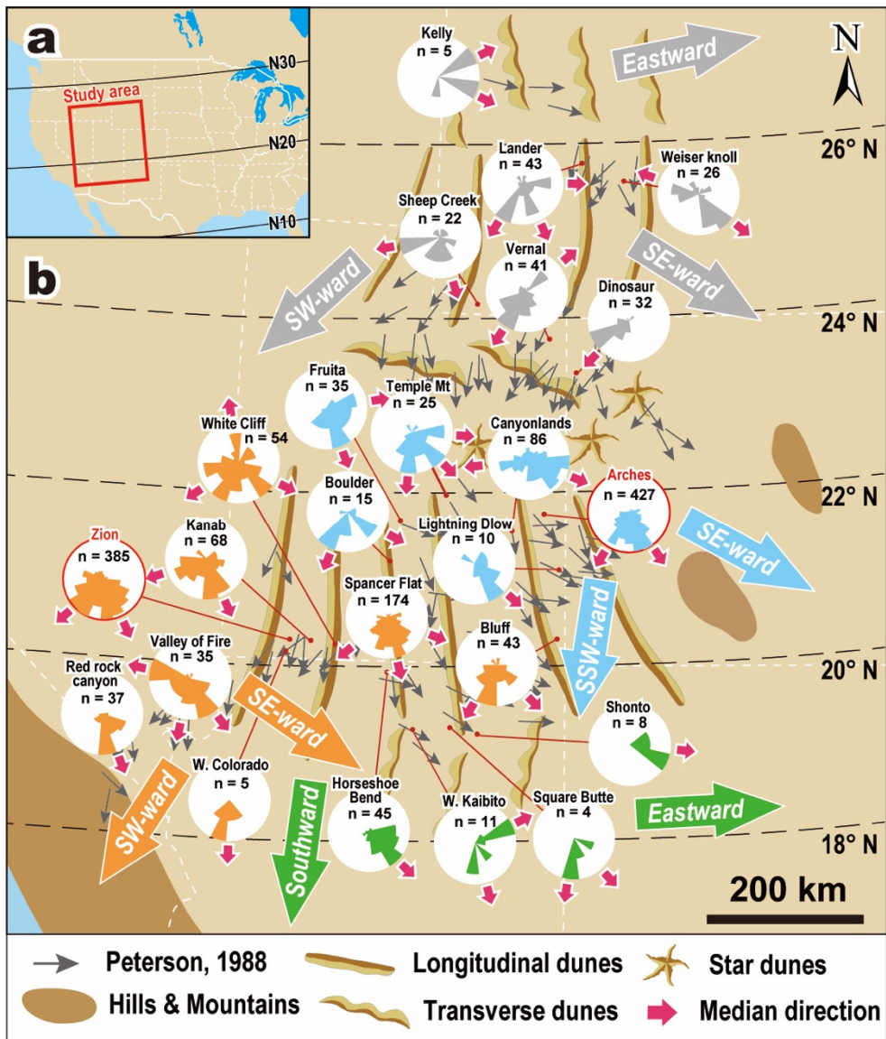
140 Figure 1: Reconstructed palaeo-wind patterns in the western US during the Early Jurassic. (a) Location of the study area in the western US. (b) Spatial distributions of dune slip-face azimuths measured in this study (shown on rose diagrams) and inferred dune morphologies, plotted on the Early Jurassic palaeogeographic map of Peterson (1988) with palaeolatitudes based on Dickinson (2018). The colours of the rose diagrams indicate the area: northern (grey), central (light blue), southwestern (orange), and southern (green) parts of the study area. Large arrows in (b) indicate the reconstructed prevailing surface wind directions in each area. The pink arrows around the outside of each rose diagrams indicate the median direction of separated components in the slip-face azimuth data provided in Table 1.
