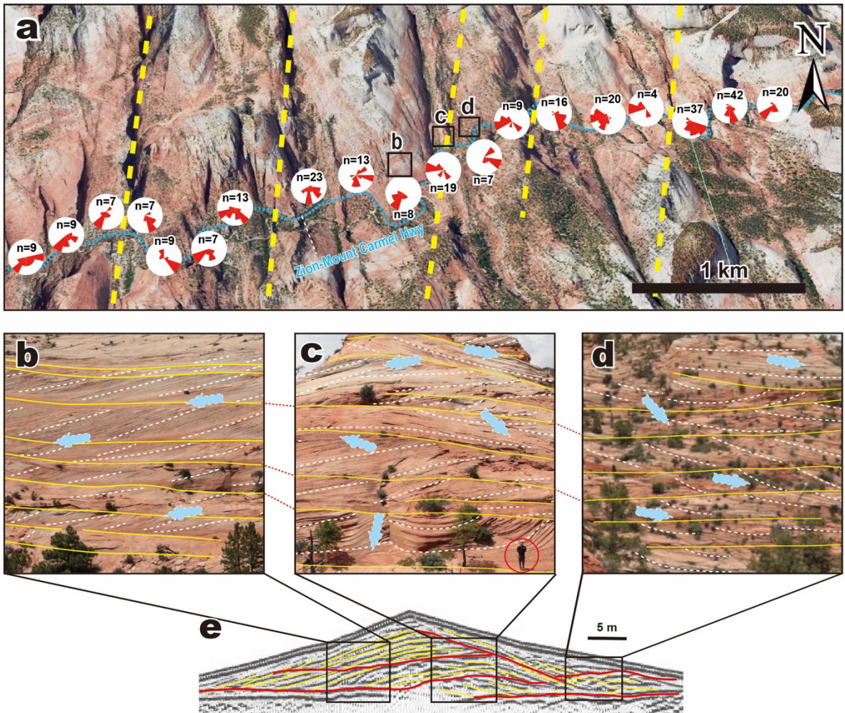
180 Figure 2: Spatial pattern of dune slip-face azimuths and outcrop photographs of the Navajo Sandstone in the Zion National Park, and comparison with the internal structure of a modern longitudinal dune. (a) Spatial distribution of 185 palaeo-wind data along the Zion–Mount Carmel Highway. Yellow dotted lines are the inferred locations of the central crests of longitudinal dunes, which are spaced at horizontal intervals of ~1 km intervals. (b–d) Outcrop photographs of cross-stratification in the Navajo Sandstone. Yellow solid lines and white dashed lines indicate the bounding surfaces of aeolian dune strata and slip-face cross-stratifications, respectively. All photographs were taken facing north. Red circle in (c) indicates a person for scale (ca. 1.7 m tall). (e) Ground-penetrating radar (GPR) profiles
