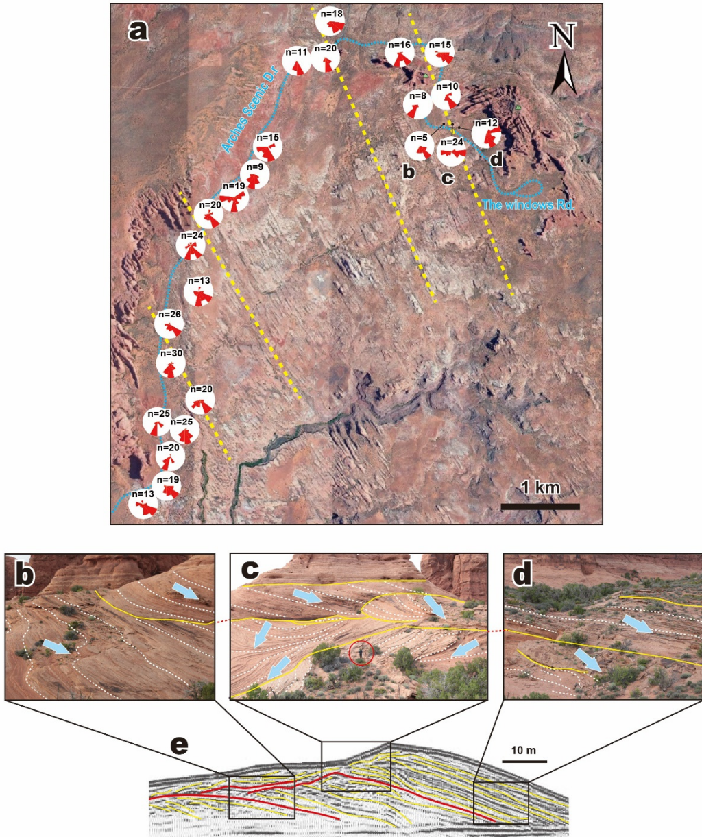
190 Figure 3: Spatial pattern of dune slip-face azimuths and outcrop photographs of the Navajo Sandstone in the Arches National Park, and comparison with the internal structure of a modern longitudinal dune. (a) Spatial distribution of palaeo-wind data along the Arches Scenic Drive. Yellow dotted lines are the inferred locations of the central crests of longitudinal dunes. (b–d) Outcrop photographs of cross-stratification structures in the Navajo Sandstone. Yellow solid lines and white dashed lines indicate bounding surface and slip-face cross-stratifications respectively. All photographs were taken facing north. Red circle in (c) indicates a person for scale (ca. 1.7 m tall). (e) Ground-penetrating radar (GPR) profile showing the internal structure of a modern longitudinal dune (Bristow et al., 2000). Yellow and red traces indicate slip-faces and unconformities, respectively. 195
