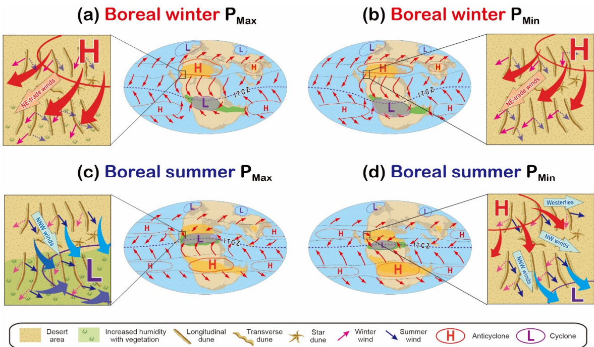
285 Figure 4: Schematic illustrations of orbital and seasonal changes in Pangaeian atmospheric pressure pattern and inferred dune alignments in western US during the eccentricity-modulated precession maximum (P Max ; a, c) and minimum (P Min ; b, d). Orbital-scale changes in pressure pattern are based on climatic model results (Winguth and Winguth, 2013). Seasonal changes in wind regimes are indicated as pink (boreal winter) and blue (boreal summer) arrows. During the eccentricity-modulated precession maximum, the continental low-pressure system in the boreal summer was likely reduced by a few hPa relative to the eccentricity-modulated precession minimum in response to 290
