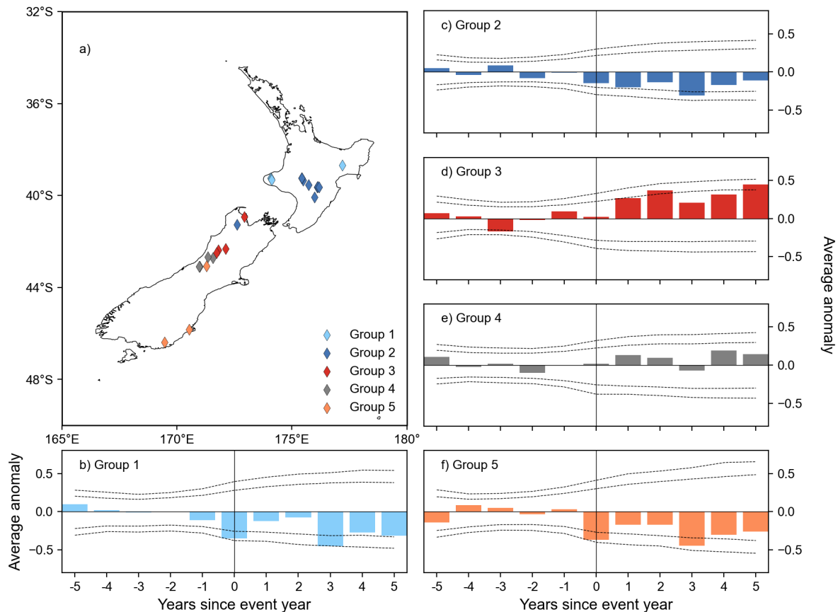
255 Figure 4 – a) Results of k-means clustering of New Zealand cedar chronologies; b) – f) mean chronology departures five years before and after eruption years (year 0), separated by cluster, and the 95th and 99th significance levels calculated by generating 10,000 random samples of non-event years from the group composite. Map part a) made with Natural Earth free vector map data available at naturalearthdata.com .
