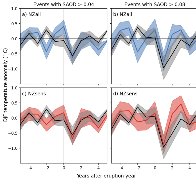
Figure 6 – Mean anomalies five years before and after 21 eruption years with SAOD > 0.04 (left column) and 13 eruption years with SAOD > 0.08 (right column), for both the NZall (blue) and NZsens (red) reconstructions. The mean response from an ensemble of seven climate models to the same set of events is shown in black. The 90th percentile bootstrap confidence intervals were constructed from 1,000 replicates of either 15 or 9 event years at random.
