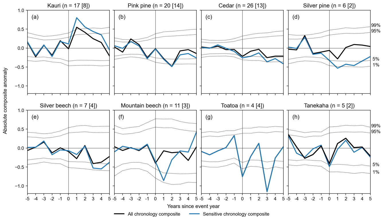
205 Figure 3 – Mean chronology departures five years before and five years after the 13 largest eruption years (year 0), separated by tree species. The chronologies contributing to the species-wide composite are shown in black, with the number of chronologies indicated in the round brackets. The sensitive chronology composite is shown in blue and the number of contributing chronologies is shown in the square brackets. Significance bands (dotted grey lines) are the 1st, 5th, 95th, and 99th percentile of 10,000 random samples of non-event years from the species-wide composite.
