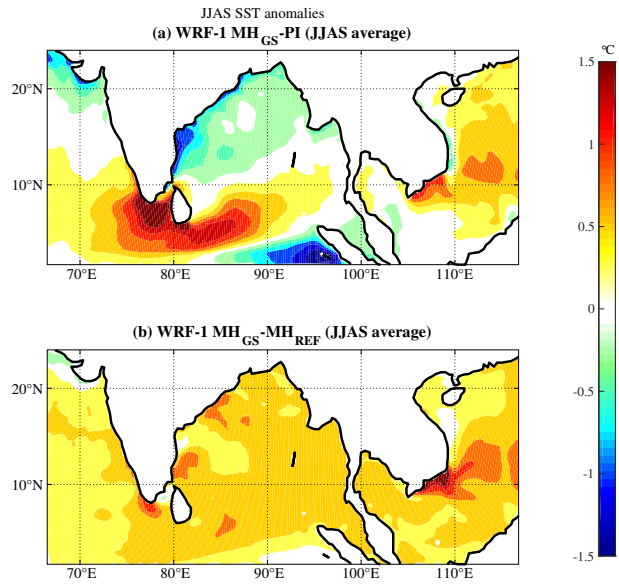
Figure S1: JJAS SST differences for the first WRF-CROCO ensemble member between a. MH_{GS} and PI , and b. MH_{GS} and MH_{REF} .
