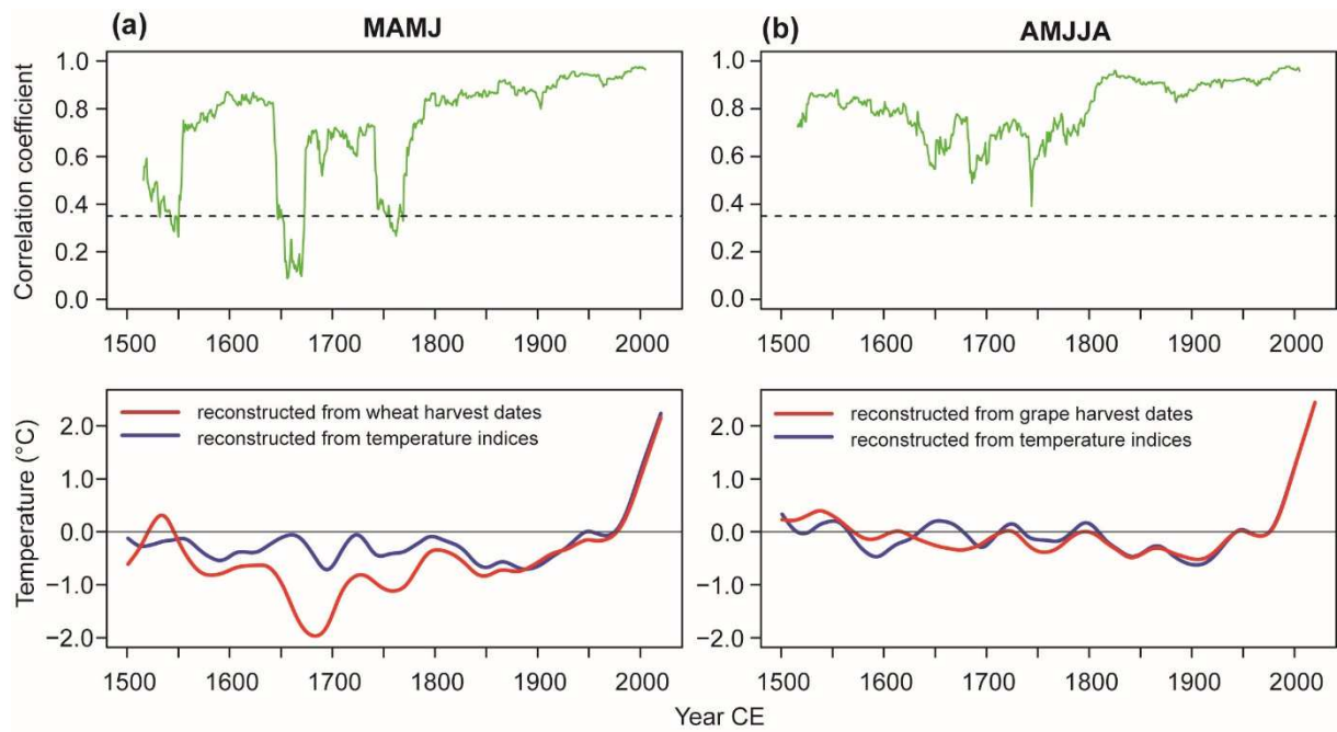
5 Figure 8. 31-year running correlations (top) and low-frequency signal expressed as smoothed series by the 60-year spline function (bottom) compared to MAMJ temperatures reconstructed from the wheat harvest dates (Možný et al., 2012) and those reconstructed from temperature indices (a); (b) the same as (a) but for AMJJA temperatures reconstructed from the grape harvest dates (Možný et al., 2016a).
