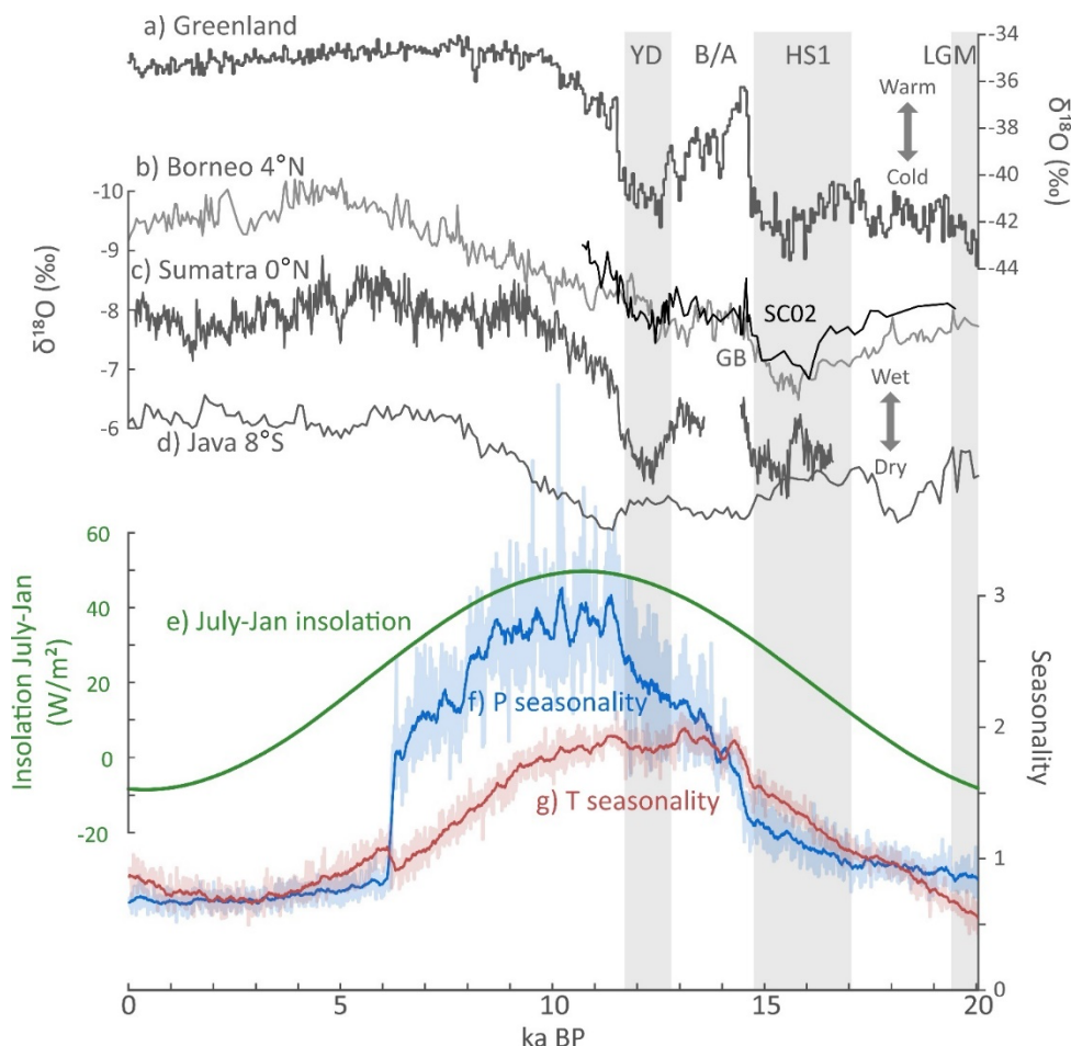
Figure 2: Long-term transient changes in temperature and hydroclimate based on proxy evidence in comparison to seasonality changes in terms of orbital forcing ( 2^\circ N ) and simulated precipitation (P) and temperature (T). a) Greenland (NGRIP) ice core \delta^{18}O indicative of
