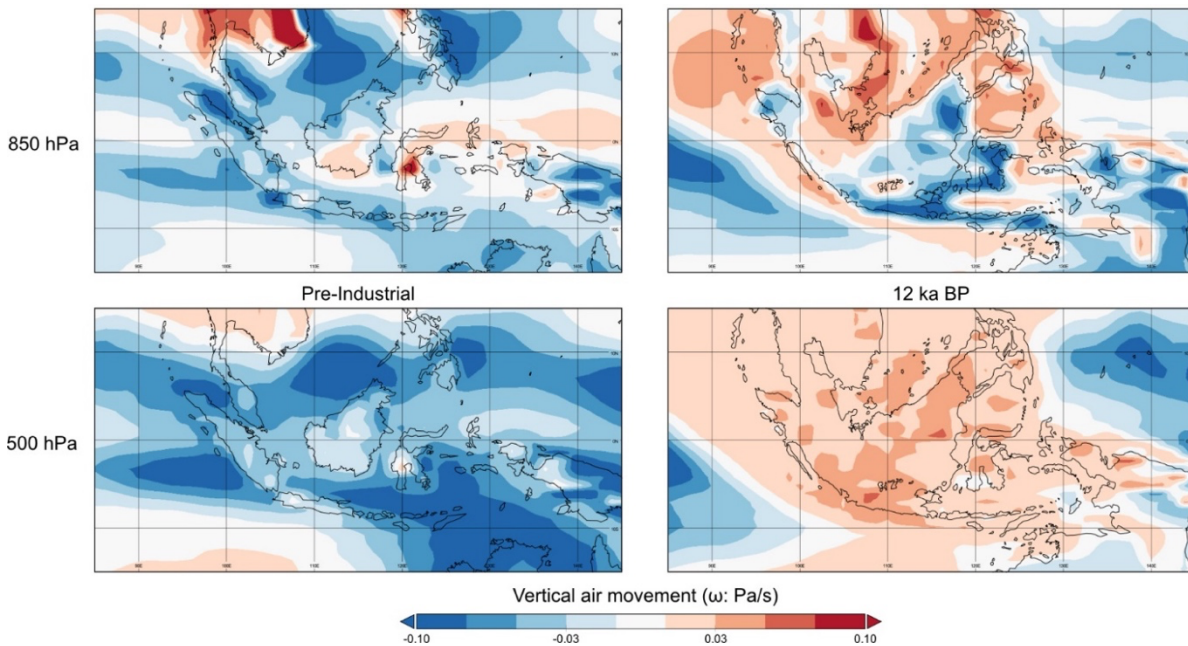
455 Figure 6. Comparison of near-surface convection/subsidence (850 hPa level) with (no) deep convection (>500 hPa level) over ISEA during January for PI (left) and 12k (right). As in Fig. 5, negative values (blue) indicate rising air/convection and positive values (red) indicate subsidence/breakdown of convection. Note that near-surface convection due to orography around Borneo at 12 ka BP keeps all months humid (>60 mm) while the overall deep convection of the PI is completely shut down over the whole IPWP region causing at least 460 seasonal aridity.
