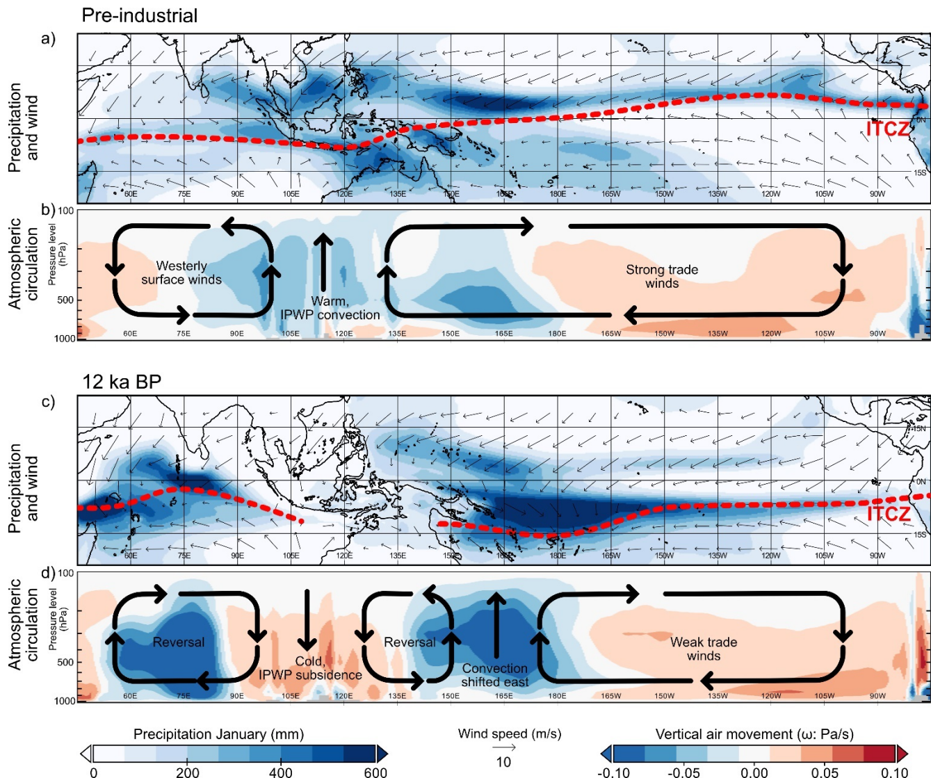
355 Figure 5. Simplified mechanistic explanation for January precipitation patterns during the pre-industrial (top) and 12 ka BP (bottom) in 360 terms of horizontal and vertical wind patterns. a) and c) show mean total precipitation (mm/month) and surface wind vectors (m/s) for January; b) and d) Omega parameter ( \omega : Pa/s) representing vertical air movement ( \omega < 0 , rising in blue; \omega > 0 sinking in red) along the equator over the Indo-Pacific region. The approximate January location of the ITCZ and atmospheric Walker Circulation patterns are indicated as red lines (a, c) and black arrows (b, d), respectively. Note that the atmospheric circulation cells are inverted over the IPWP region at 12 ka BP where subsiding air masses, a breakdown of deep convection and divergent winds from land to sea cause seasonal aridity over tropical land areas. For details on the weakening and/or reversal of the zonal winds, see Fig. S7.
