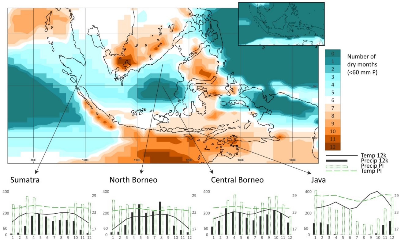
320 Figure 4: Number of simulated dry months per year at 12 ka BP and comparison of the regional annual temperature and precipitation cycles for 12 ka BP and PI. The inset shows the number of dry months (<60 mm P/month) per year for PI. Climate diagrams show the monthly average temperature and precipitation from PI (green) and 12 ka BP (black) based on CESM1 simulations. Sumatra, Java and North Borneo locations approximately correspond to speleothem cave locations from the reconstructions in Fig. 2.
