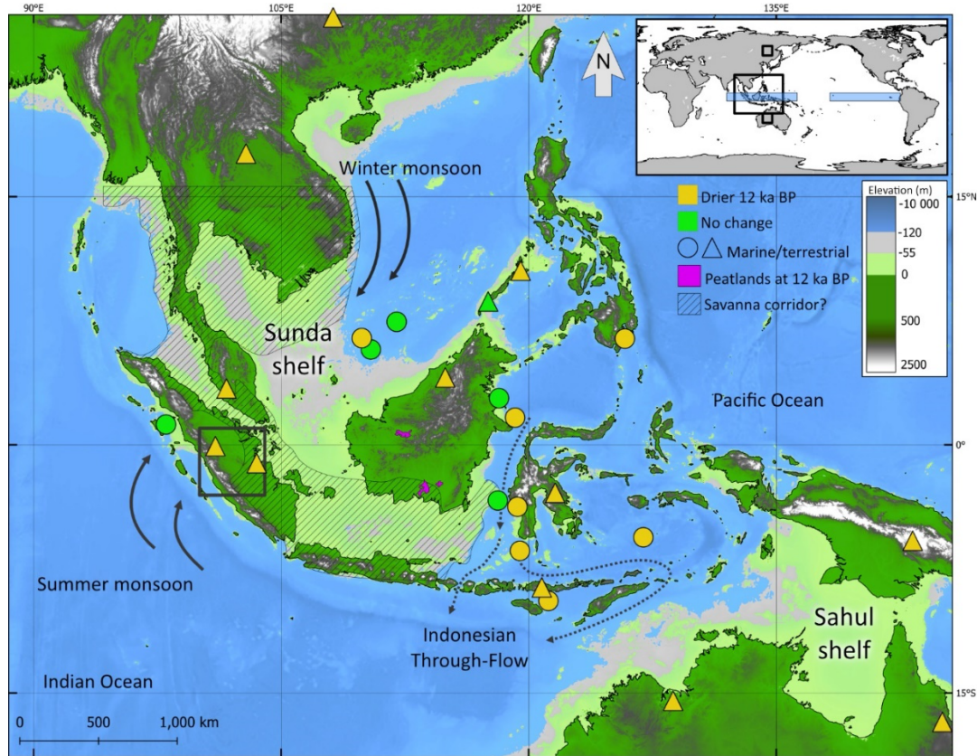
105 Figure 1: Topographic map of South-East Asia and a compilation of available climate proxy records (supplementary Table 1). Yellow markers indicate drier or more seasonal climate at 12 ka BP compared to PI, and green indicates no notable difference. Purple areas denote the peatland extent at 12 ka BP (Dommain et al., 2014). Exposed land due to lower sea level at 12 ka BP shown in light green and in light gray for the LGM. The hatched area indicates the proposed savanna/seasonal deciduous forest corridor on the Sunda shelf at the LGM (Cannon et al., 2009). Black square on the regional map indicates the area used to track long-term changes in seasonality from TRACE (Fig. 2 f, g). Small black squares in the global map inset show the areas used for estimating the thermal gradient over ISEA and blue squares are used for Walker Circulation Index calculations (Fig. 7a). 110
