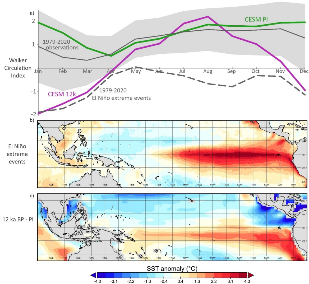
490 Figure 7. Comparison of the monthly mean Walker Circulation Index and SST anomalies for 12 ka BP and the modern states. a) Monthly mean Walker Circulation Index based on CESM1 simulations for PI (green) and 12 ka BP (purple) and ERA5 reanalysis data for 1979- 2020 (gray) with shading denoting \pm 1 standard deviation in ERA5 monthly mean data. Also shown is the composite average over three most extreme El Niño extreme events (dashed gray line) from ERA5 (1983, 1998 and 2015). b) Average SST anomalies for the same three
