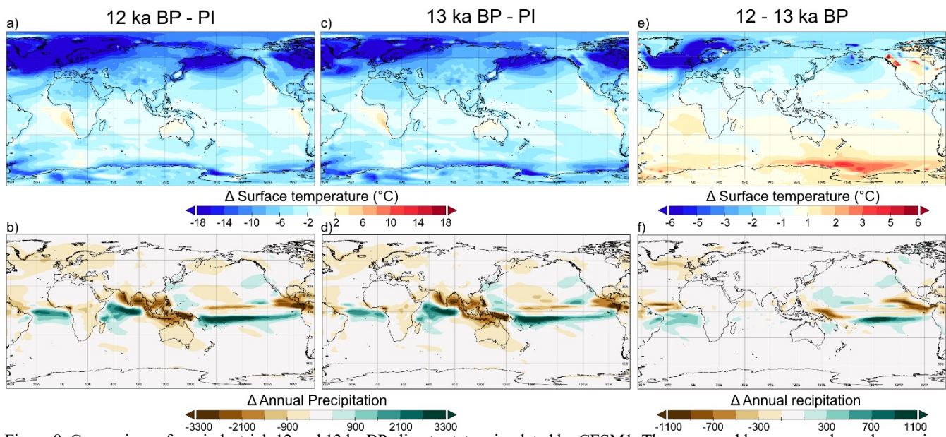
Figure 8. Comparison of pre-industrial, 12 and 13 ka BP climate states simulated by CESM1. The upper and lower rows show changes in temperature and precipitation, respectively. a-d) show that the changes between 12 and 13 ka BP relative to PI are very similar in the tropics. e and f) show changes between 12 and 13 ka BP which most notably consist of NH cooling, and SH warming, and that tropical Pacific precipitation patterns are shifted.
