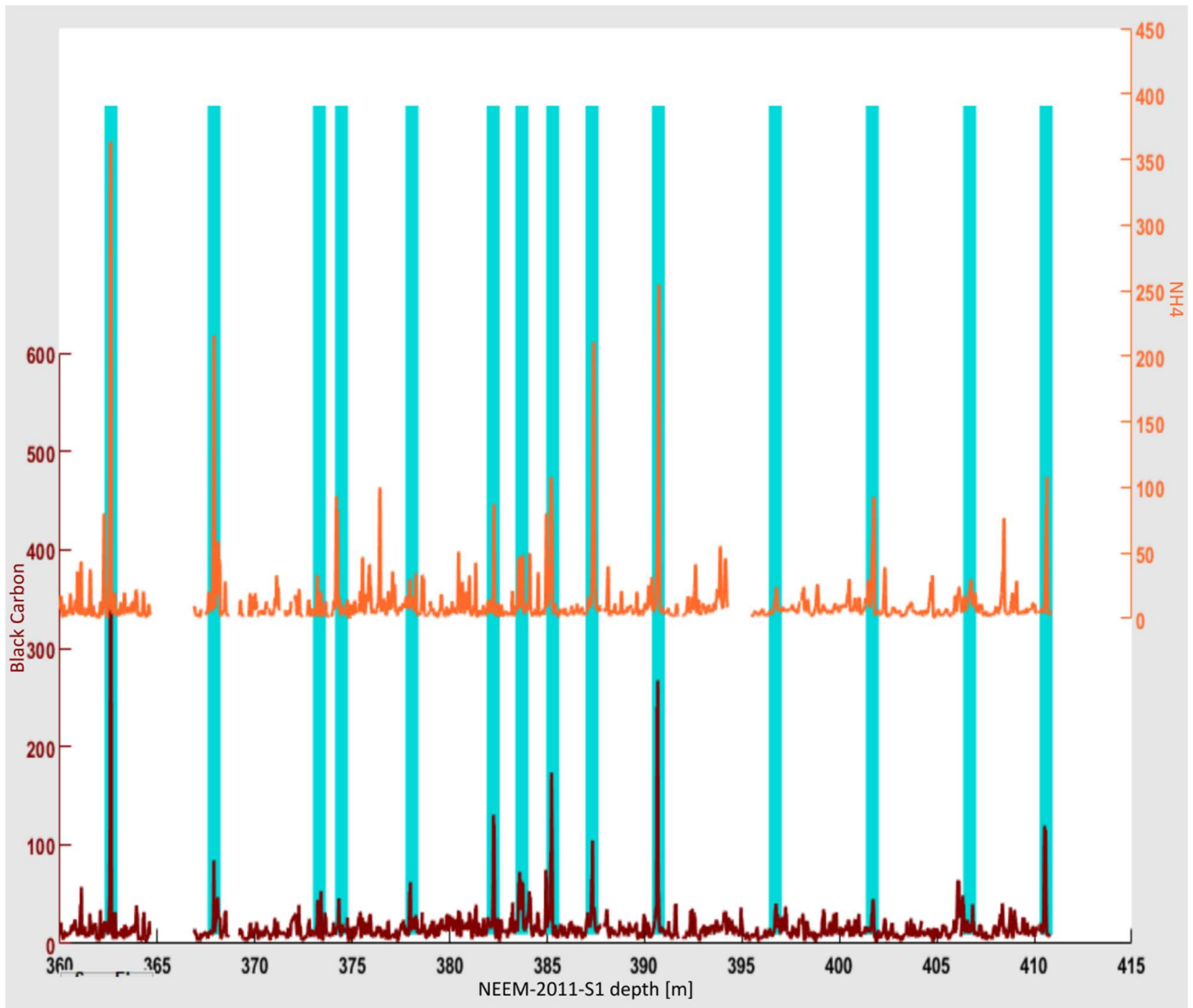
Figure 1 NEEM-2011-S1 Black Carbon and \text{NH}_4^+ comparison. The blue bars are not GICC21 tie-points but merely indicate the co-occurrence of \text{NH}_4^+ peaks with BC peaks.
