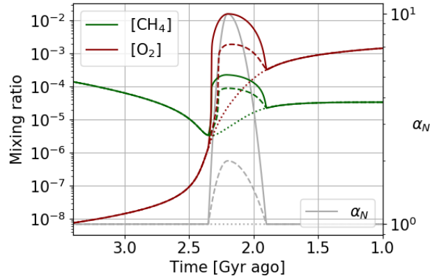
Figure 18. Oxygen and methane temporal evolution. Models \alpha_N constant equal 1, reaching a factor 2 and reaching a factor 10.
