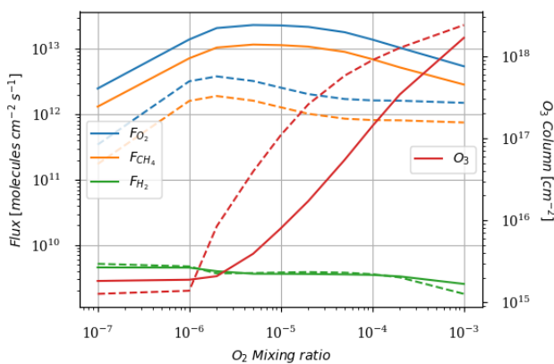
Figure 9. Surface oxygen ( F_{O_2} ) and methane ( F_{CH_4} ) fluxes, hydrogen escape ( F_{H_2} ) and O_3 column density as a function of surface O_2 for a surface CH_4 set up at 10^{-4} . Results for 1D model surface temperature 280K (solid) and 220K (dashed).
