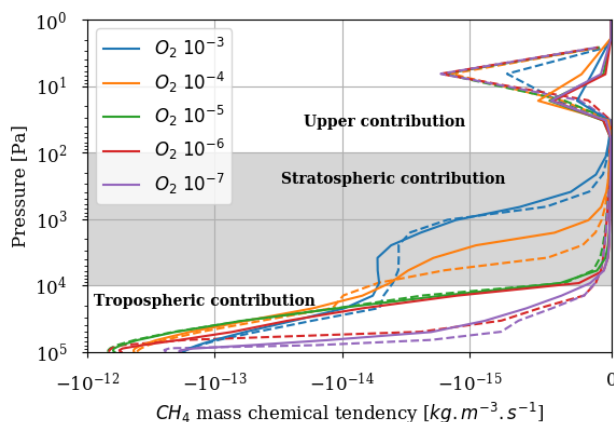
Figure 5. Methane photochemical losses as a function of altitude for several O_2 levels and a methane vmr of 10^{-4} at the surface. Solid: results of 3D model (averaged over the surface and a year). Dashed: 1D results.
