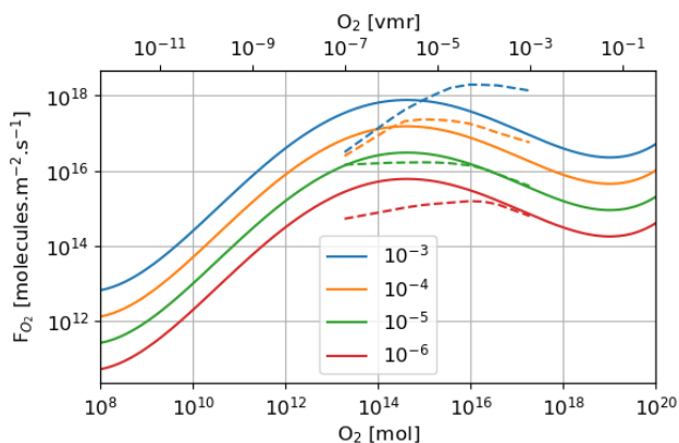
Figure 15. Oxygen atmospheric loss ( F_{\text{O}_2} ) depending on oxygen and methane (label in [vmr]). Goldblatt et al. (2006) parametrization (solid) and GCM 1D results (dash).
