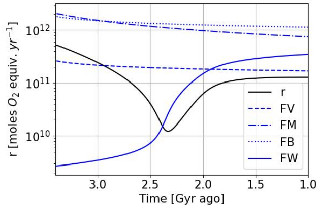
Figure 14. Temporal evolution of the reductant contributions (see Table 1) with \alpha_i = 1 and using for oxygen atmospheric loss ( F_{O_2} ) the Goldblatt et al. (2006) parametrization.
