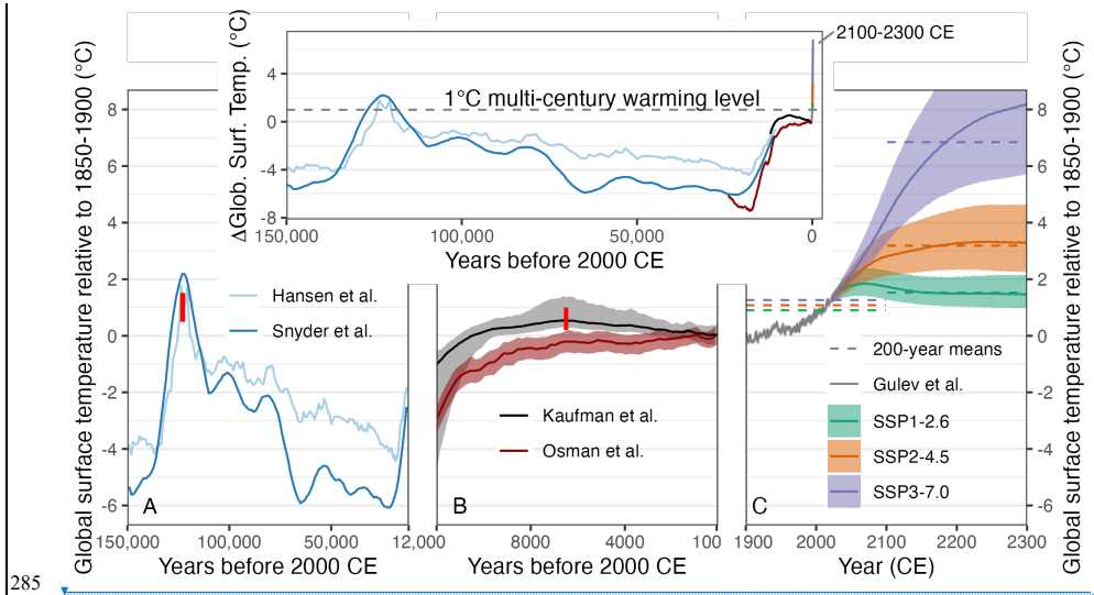
285 290 295 Figure 1: Global surface temperature (GST) over 150,000 years relative to 1850-1900. Three timescales are shown according to their published resolutions: (A) 150 to 12 ka based on marine oxygen isotopes in foraminifera (Hansen et al., 2013; Snyder, 2016). (B) 12 ka to 1900 CE based on the Temp12k multi-method, multi-proxy ensemble reconstruction (Kaufman et al., 2020b) and a post-AR6 reconstruction that blends marine proxy evidence with a climate model simulation (Osmann et al., 2021); and (C) 1900 to 2300 based on instrumental observations (gray line) (Gulev et al., 2021), and projections using three emissions scenarios (low, intermediate, and high) as assessed in AR6 (Lee et al., 2021). Horizontal dashed lines are 200-year averages (1900-2100, 2100-2300). Lines in (A) and (B) show the mean and shading in (B) shows the 5-95% range. Red vertical lines are the IPCC assessed (medium confidence; Gulev et al., 2021) temperature ranges from proxy evidence for the warmest intervals of the Last Interglacial (around 125,000 years ago, 0.5-1.5°C) and Holocene (around 6500 years ago, 0.2-1°C). These values are based on multiple studies, including the time series displayed here. Inset shows all three panels on the same time scale with 200-year resolution so that past, present and future are directly comparable.
