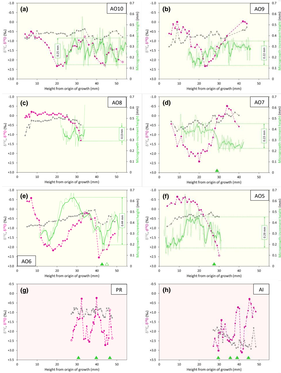
Figure 7: Isotopic, microgrowth-increment and growth-break data from Merksem-equivalent A. opercularis (a, b) and Oorderen Member (and equivalent) A. opercularis (c-f), P. rustica (g) and A. islandica (h). Format and symbols as in Fig. 6.
