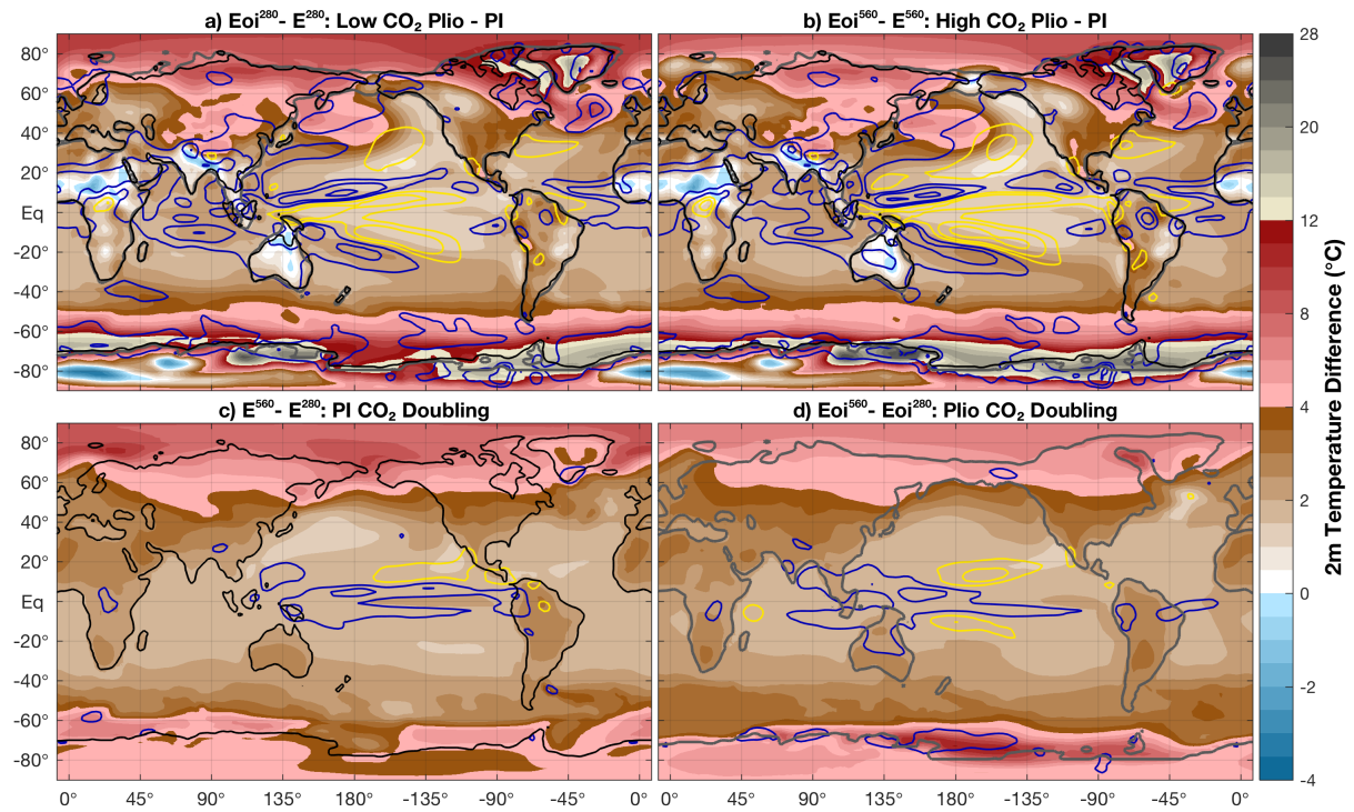
Figure C2: Altered version of Figure 10, with simplified colour scale and precipitation contours.
