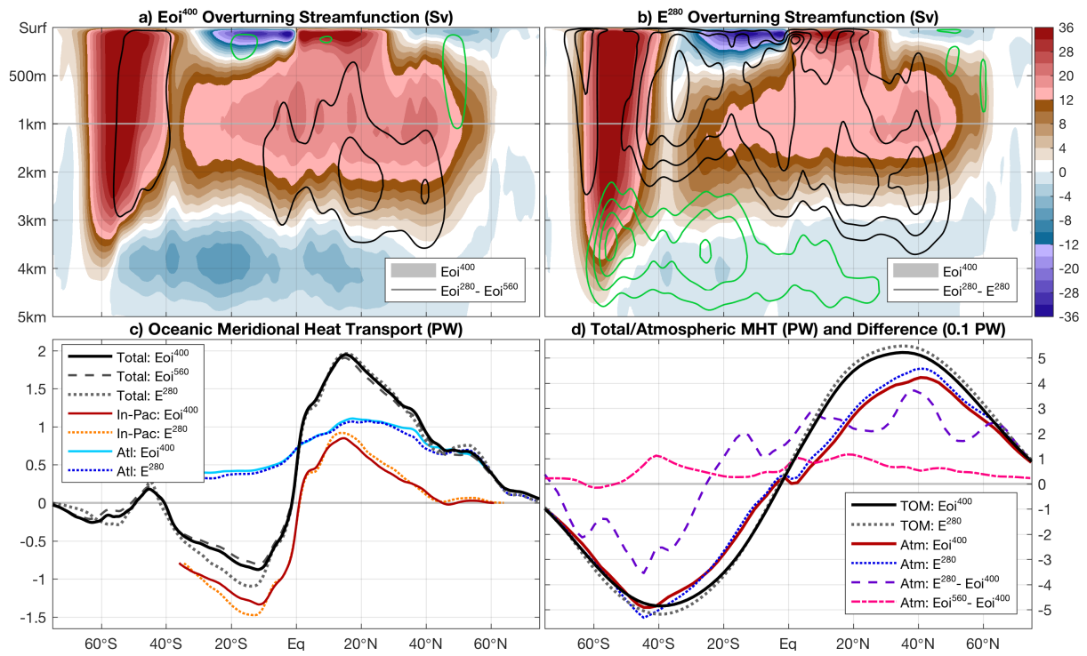
Figure C3: Updated version of Figure 7, using contours for differences only.
