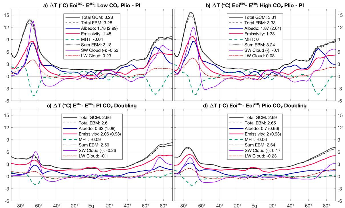
Figure C1: Energy balance analysis following Lunt et al. (2021), zonal average differences.
