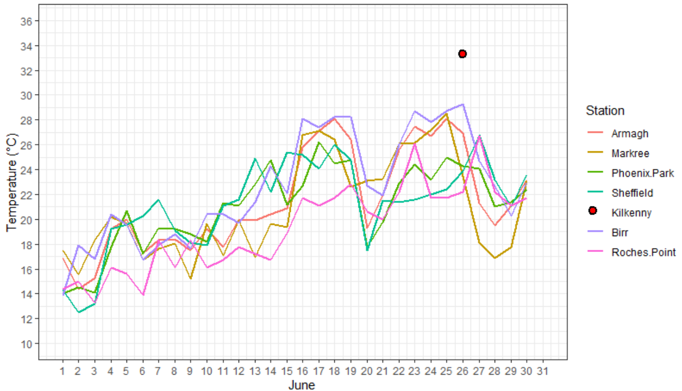
Figure 3. The maximum air surface temperatures of the six selected weather stations for the month of June 1887. The red point marker displays the maximum surface temperature recorded at Kilkenny on the 26 th June 1887.
