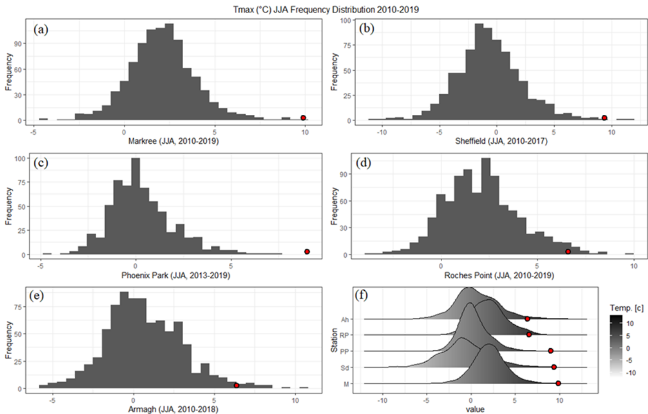
Figure 7(a-e). Modern day distribution for the JJA season differences between the maximum temperature of Kilkenny Greenshill and the five stations where the data was most available and (f) and amalgamation of all of the stations for comparison purposes. Shown in red is the difference reported on June 26th 1887 between each station and Kilkenny Castle.
