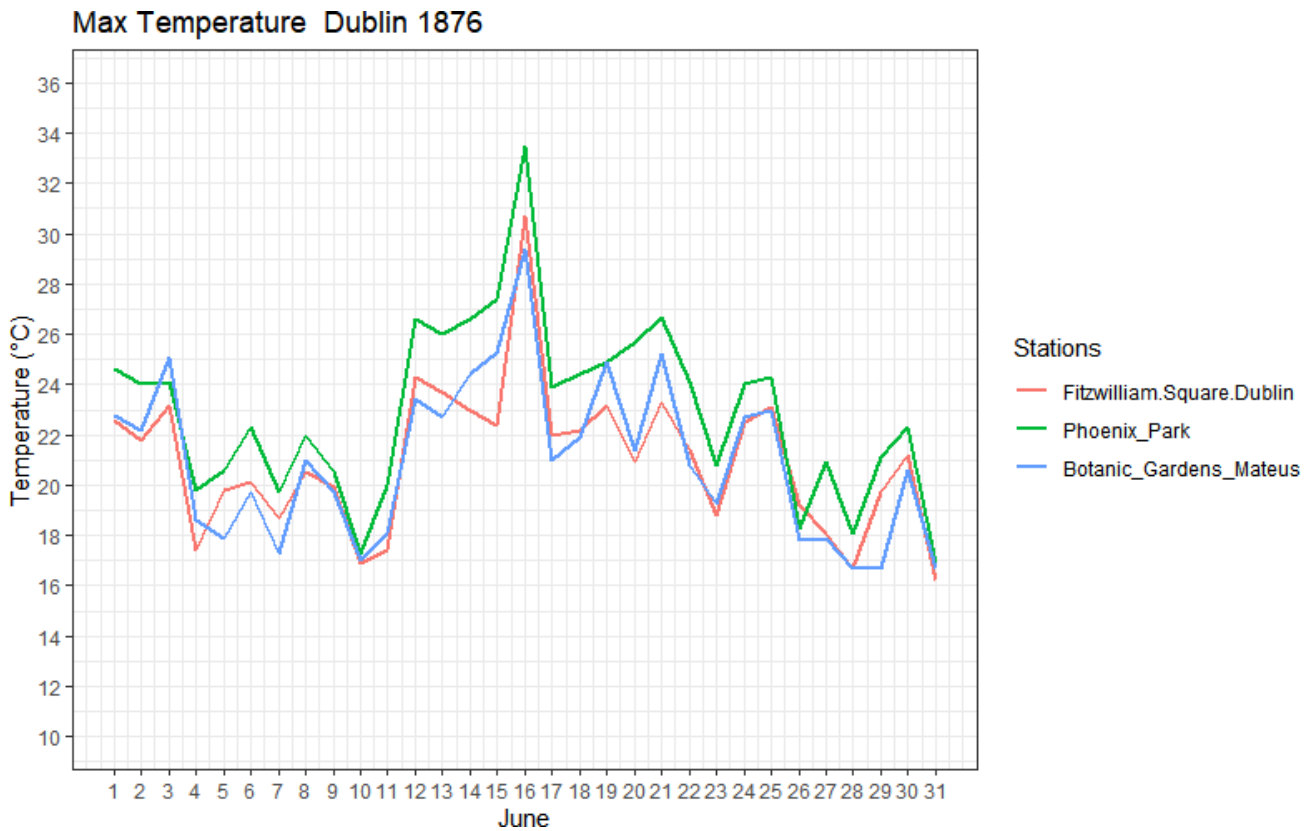
400 Figure 11: The maximum surface temperatures of all available stations in Dublin City during June 1876.
