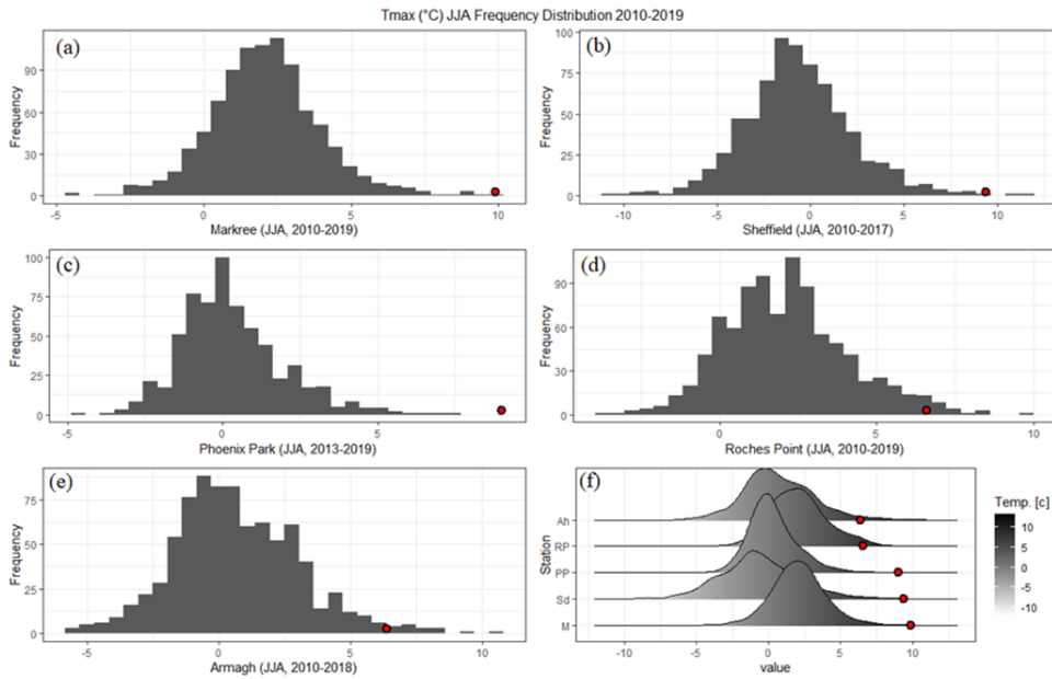
285 Figure 6f (a-e). Modern day distribution for the JJA season differences between the maximum temperature of Kilkenny Greenshill and the five stations where the data was most available and (f) and amalgamation of all of the stations for comparison purposes. Shown in red is the difference reported on June 26th 1887 between each station and Kilkenny Castle. Modern day distribution for the JJA season differences between the maximum temperature of Kilkenny Greenshill and the four stations where the data was most available. Shown in red is the difference reported on June 26th 1887 between each station and Kilkenny Castle.
