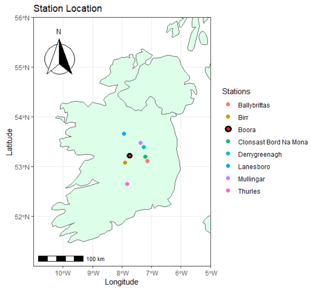
Figure 134: Map of stations closest to Boora considered in this analysis
