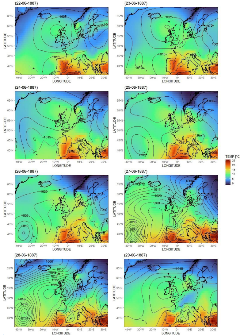
NOAA 20CRV3 MSLP & 850-hPa Temperatures
