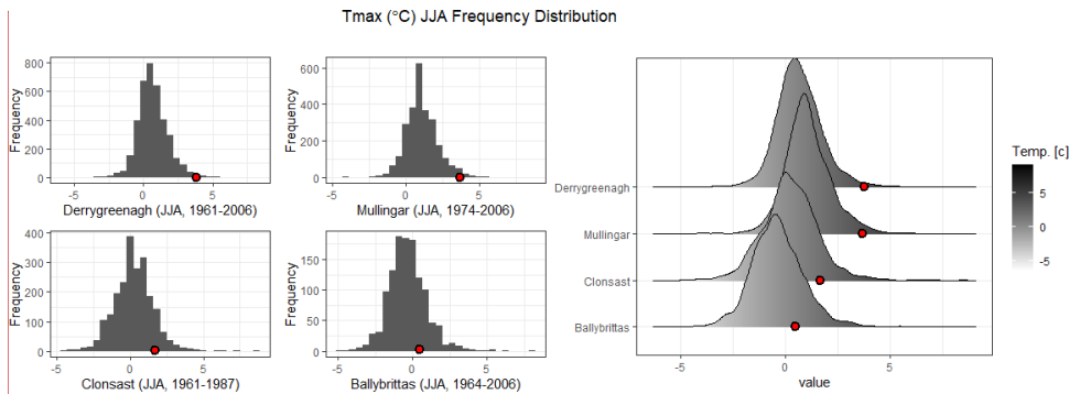
Figure 142. Modern day distribution for the JJA season differences between the maximum temperature of Boora, Offlay and the sevenfour stations where adequate the data was most available. Shown in red is the difference reported on June 29 th , 1976 between each station and Boora.
