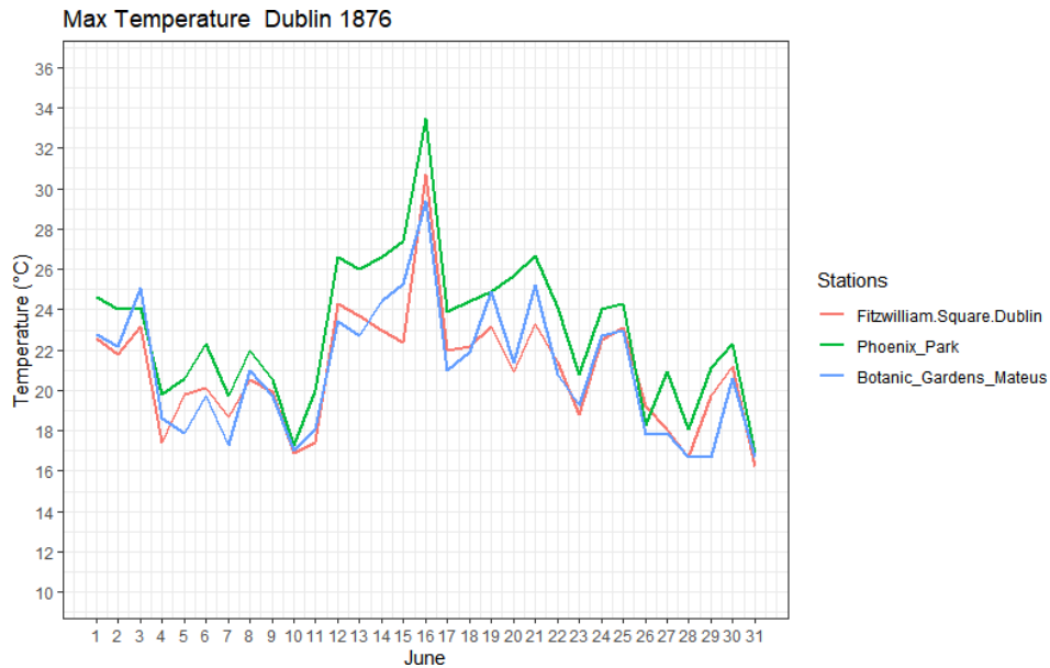
Figure 118: The maximum surface temperatures of all available stations in Dublin City during June 1876.
