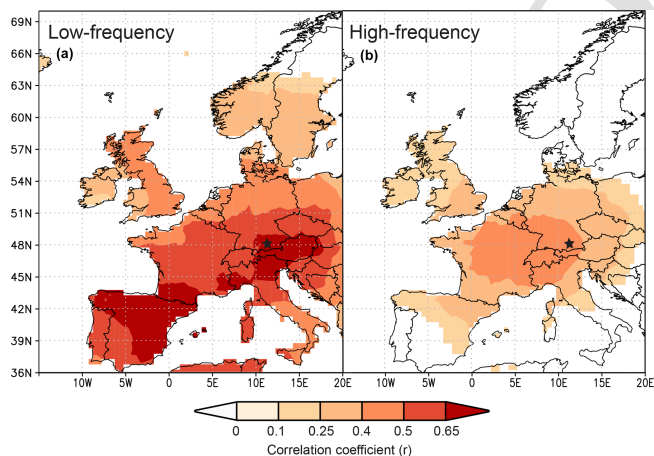
Figure 5. Spatial correlations between summer temperatures (CRU TS4.04) and \delta^{13}\text{C}_{\text{LM}_{\text{RL}}} anomalies (a) and \delta^{13}\text{C}_{\text{LM}_{\text{high-frequency}}} indices (b) from 1916–2015. Black star marks the Hohenpeißenberg in Germany.
