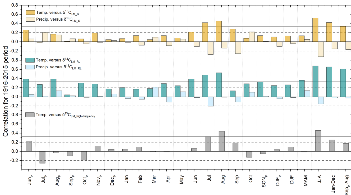
Figure 4. Correlation coefficients between corrected \delta^{13}\text{C}_{\text{LM}_S} , \delta^{13}\text{C}_{\text{LM}_{\text{RL}}} , \delta^{13}\text{C}_{\text{LM}_{\text{high-frequency}}} chronologies and local temperatures and precipitation totals from 1916 to 2015. The subscript p indicates the months of the previous year, and horizontal lines indicate the significance levels, with solid lines representing highly significant ( p < 0.001 ) and dashed lines representing significant values ( p < 0.05 ).
