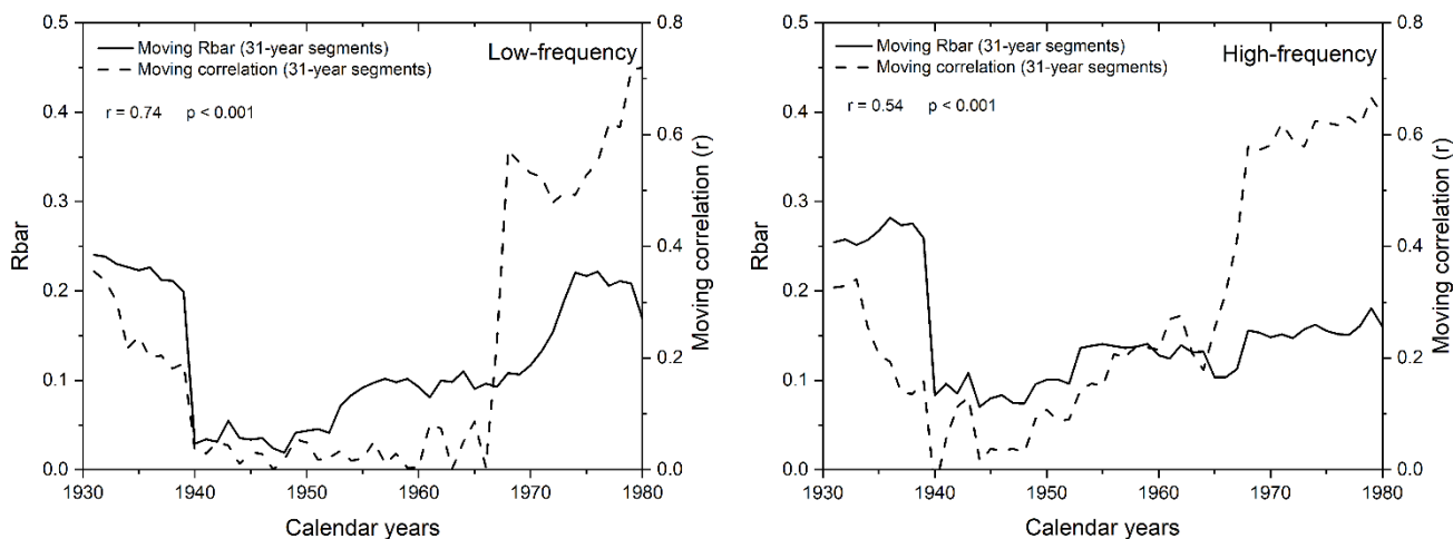
Figure 10. 31-year moving correlations between gridded instrumental and modelled summer temperatures using \delta^{13}\text{C}_{\text{LM\_RL}} values (left site) and \delta^{13}\text{C}_{\text{LM\_high-frequency}} indices (right site) (dashed lines) plotted together with the 31-year moving Rbar values of these data (solid lines).
