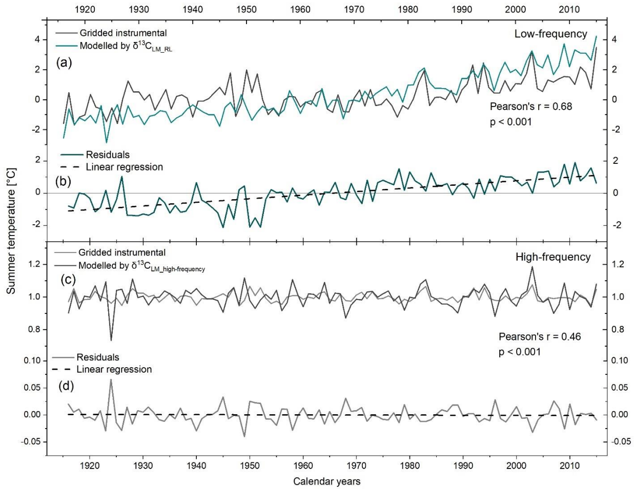
Figure 6. Gridded instrumental and modelled JJA temperatures by (a) \delta^{13}C_{LM\_RL} values and (c) \delta^{13}C_{LM\_high-frequency} indices from 1916-2015. (b) and (d) plots of residual trends through time for low- and high-frequency.
