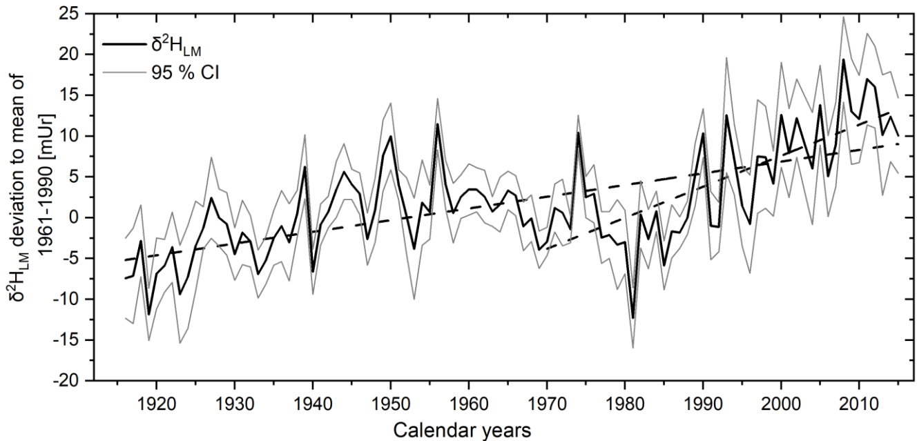
Figure 8. The corrected mean \delta^2\text{H}_{\text{LM}} anomalies as deviations from the 1961-1990 mean from 1916-2015. The 100-year record (black line) represents the mean of the eight individual tree ring series with 95 % CI (grey lines). Linear regression lines (dashed) are shown for the whole period and from 1970-2015.
