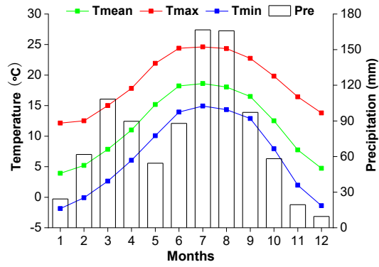
Updated ombrothermic diagram
