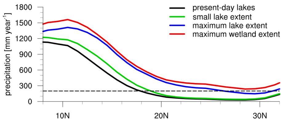
Figure 2. Mid-Holocene 30-year mean annual precipitation zonally averaged over Africa ( 10^\circ\text{E} - 30^\circ\text{W} ).
