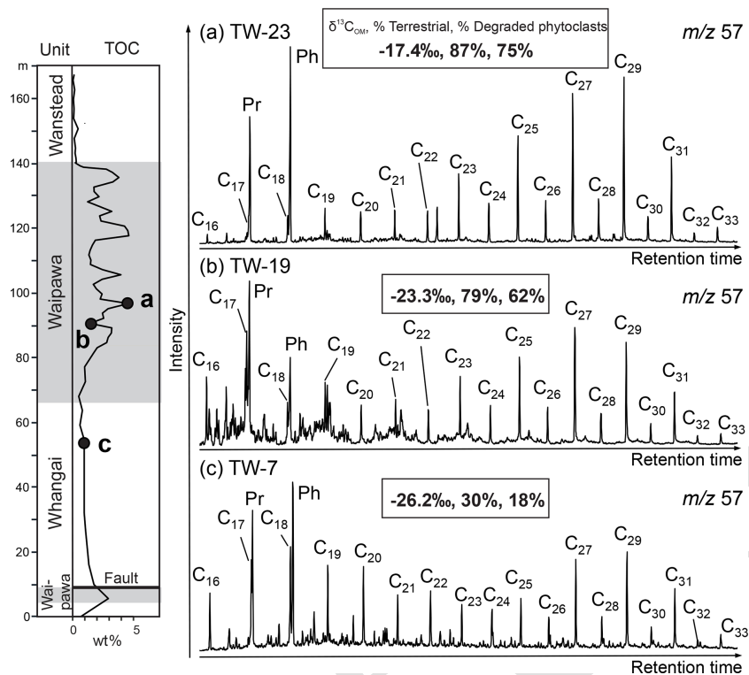
Figure 6. Representative biomarker chromatograms for (a) organic-rich Waipawa facies, (b) organic-poor Waipawa facies and (c) Whangai facies in the Taylor White section. The \delta^{13}C_{OM} value and percentages of terrestrial palynodebris and degraded phytoclasts are also shown for each sample. Identified peaks are n -alkanes, pristane (Pr) and phytane (Ph).
