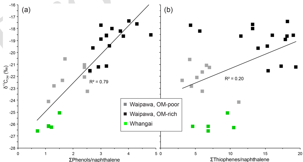
Figure 7. Correlation of \delta^{13}C_{OM} with (a) phenol and (b) thiophene abundances relative to naphthalene for the OM-rich (TOC > 2 wt %) and OM-poor (TOC < 2 wt %) Waipawa facies and Whangai facies in the Taylor White section. Naphthalene is used to normalize these compounds because it is a generic compound independent of source. Linear regressions include all samples.
