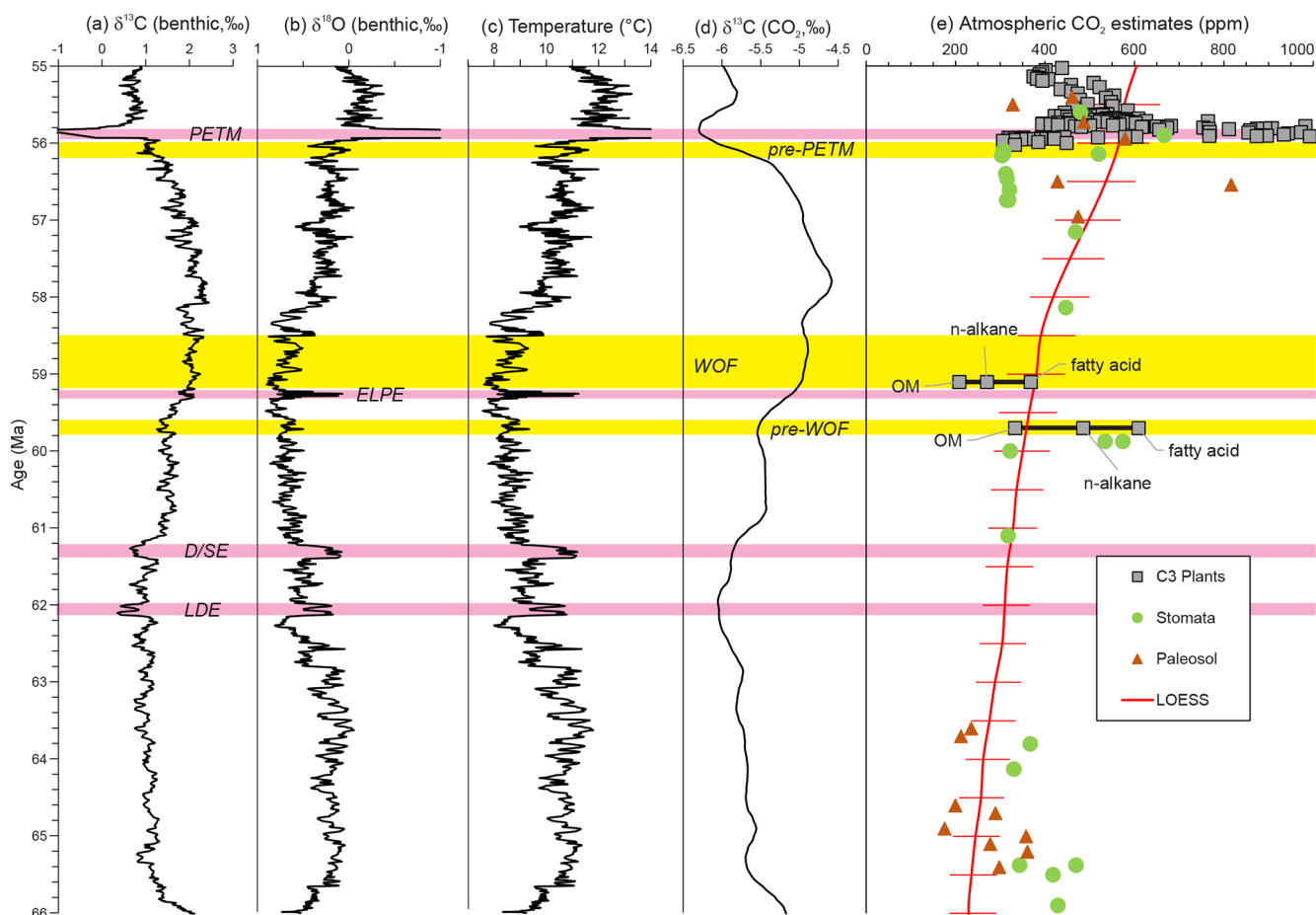
Figure 14. Compilation of early Paleogene variation in deep-sea benthic foraminiferal (a) carbon and (b) oxygen isotopes (LOESS smoothed curves from Westerhold et al., 2020), (c) oxygen isotope-based temperatures, (d) carbon isotope values for atmospheric CO 2 and (e) estimates for atmospheric CO 2 volume (after Foster et al., 2017; Hollis et al., 2019; LOESS curve from Foster et al., 2017). Horizontal pink bands – hyperthermals or carbon isotope excursion; horizontal yellow bands – reference time slices for CO 2 determinations; WOF indicates Waipawa organofacies. TSS
