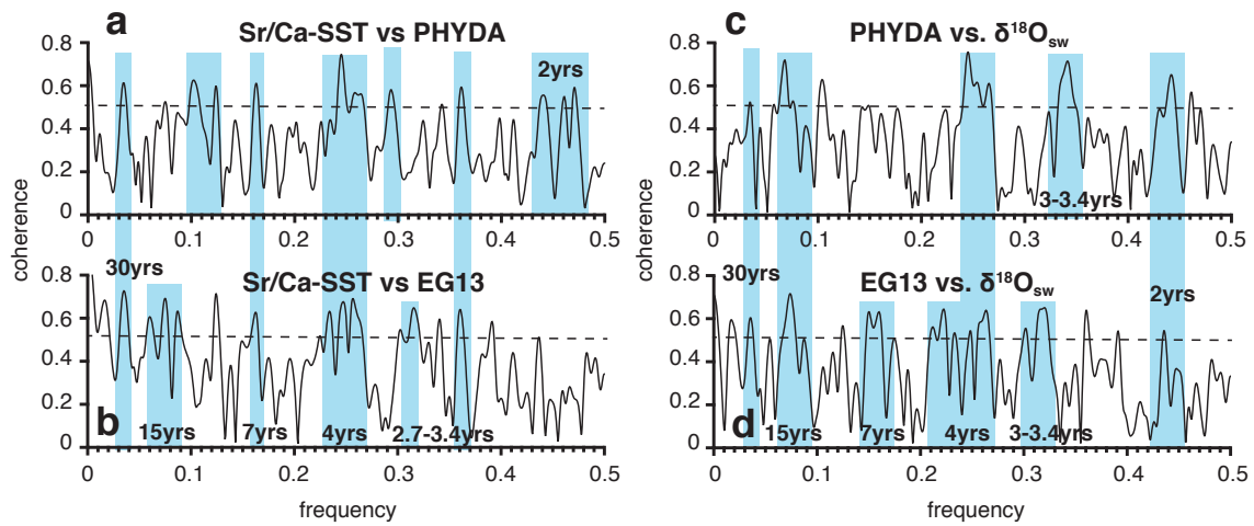
Figure S12 - Blackman-Tuckey spectral coherence between Ifaty-Tulear Sr/Ca-SST (a and b) and \delta^{18}\text{O}_{\text{seawater}} composites (c and d) with Niño3.4 reconstructions of Steiger et al. (2018; PHYDA) and Emile-Geay et al. (2013; EG13) between 1661 and 1995. Coherent frequency bands above 90% significance level (dashed line) shaded in light blue.
