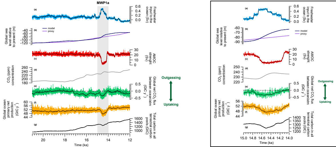
Figure 2. Time series of ocean and atmosphere variables over the last deglaciation. The presented outputs start at 21 ka, after the spin-up runs between 26-21 ka. (a) Freshwater input to the global ocean. (b) Global sea level estimate from Spratt and Lisiecki (2016) (light purple) and modelled in MPI-ESM based on the freshwater inputs (dark purple). (c) Atlantic Meridional Overturning Circulation streamfunction. (d) \text{CO}_2 concentration measured in ice cores and prescribed in the model (Bereiter et al., 2015; Köhler et al., 2017). (e) Modelled global net \text{CO}_2 flux between the ocean and the atmosphere. Positive \text{CO}_2 flux values means that the ocean is outgassing to the atmosphere and negative \text{CO}_2 flux values means that the ocean is uptaking carbon. (f) Global ocean net primary production. (g) Total carbon in all terrestrial carbon pools, i.e. vegetation, soil and litter. The thick darker curves are 500 years running mean for the panel (a) freshwater input and 50 years running mean for the other panels (c), (e) and (f). A zoom over MWP1a Meltwater Pulse 1a is presented on the right.
