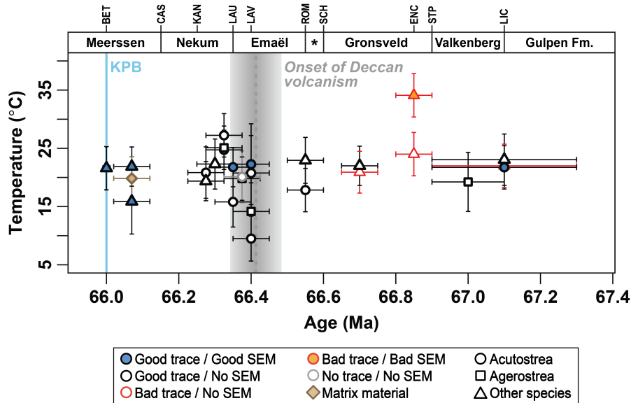
345 Figure 5: Maastrichtian \Delta_{47} -derived paleotemperatures for all samples. Samples shown in red ( n=4 ) did not pass screening thresholds and were not included in further interpretation. Error bars represent the larger of either the internal or long-term 1SE (see text). Onset of the main Deccan Traps eruptions (grey shading) at 66.413 \pm 0.067 Ma (Sprain et al., 2019). Member names and horizon abbreviations are labeled across top of figure (see Fig. 2). *Schiepersberg Member
