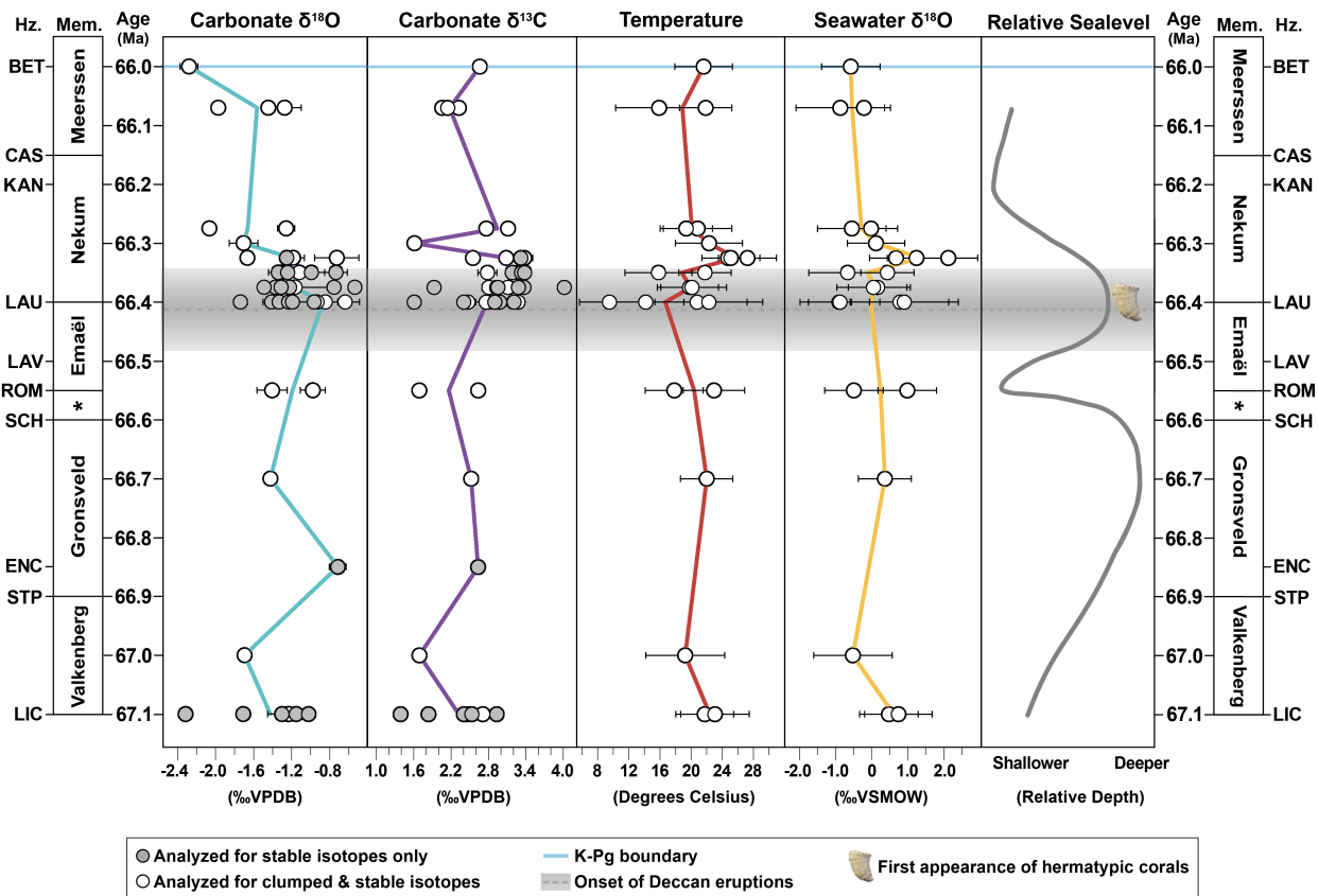
395 Figure 6: Isotopic compositions and paleotemperatures of fossil shells compared to inferred relative sea level in the Maastricht Formation. Error bars represent 1SD for \delta^{18}\text{O} (a) and \delta^{13}\text{C} (b), and external 1SE for temperature (c) and \delta^{18}\text{O}_{\text{sw}} (d) (see section 3.3). All samples failing diagenetic screening criteria have been removed. Colored lines pass through horizon means. Age model from Vellekoop et al. (2022.) (Table S3). The relative sea level curve (e) is based on Schiøler et al. (1997), adjusted to the age model used in this study. Hermatypic coral appearance data (e) is from Leloux (1999). Onset of the main 400 Deccan Traps eruptions (grey dotted line) at 66.413 \pm 0.067 Ma (Sprain et al., 2019).
