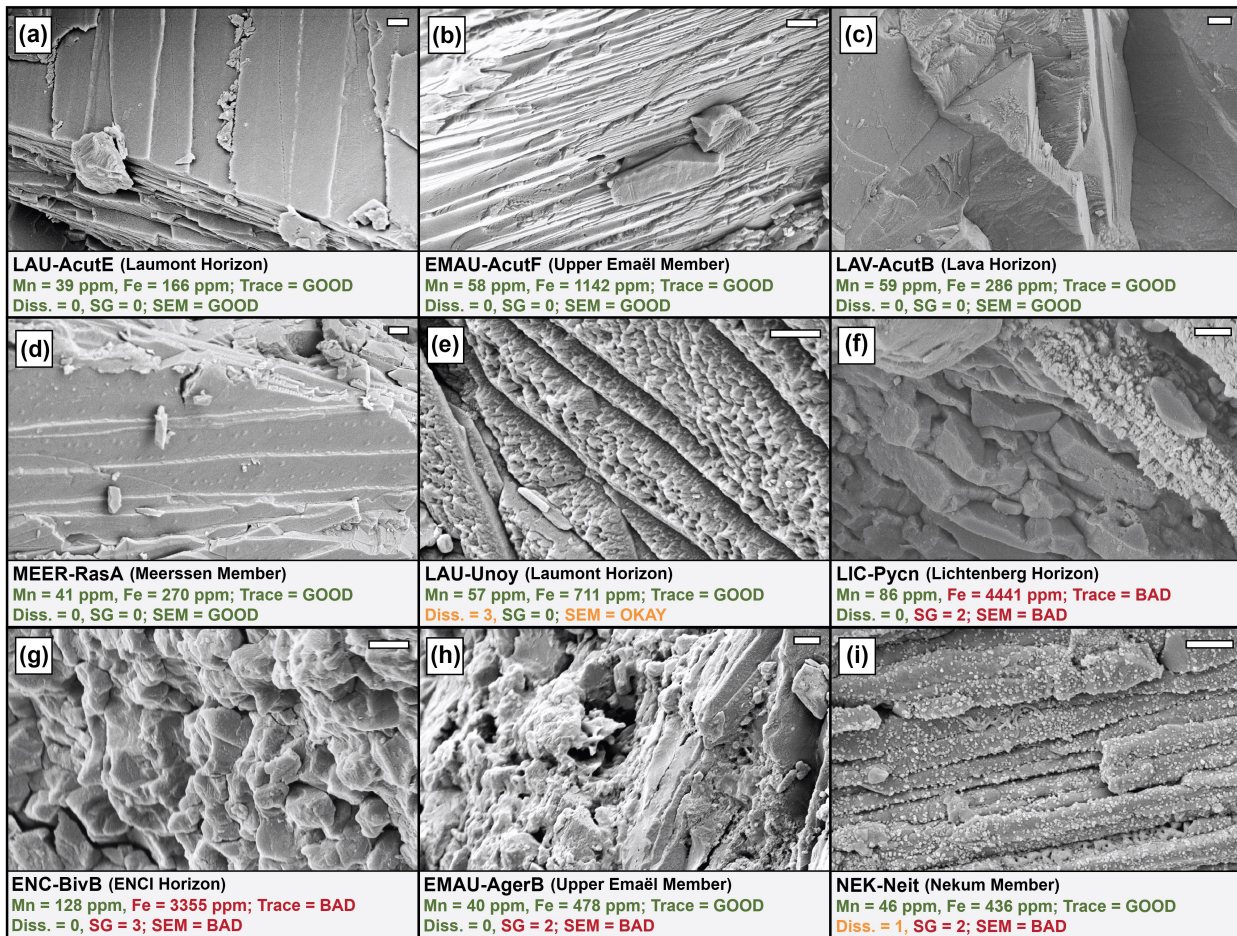
Figure 3. SEM images of nine shell specimens representing varying levels of calcite preservation. Scale bars represent 1 \mu m. Images were adjusted for brightness in Adobe Photoshop 2022. Trace element concentrations (in ppm) and SEM preservation indices quantifying the level and prevalence of dissolution and secondary growth (SG) on a scale of 0–3 are shown below each image for comparison. Samples (a) through (e) were interpreted. Samples (f) through (i) were not interpreted further, due to too much evidence of secondary growth and/or trace elements exceeding thresholds (see Fig. 4).
