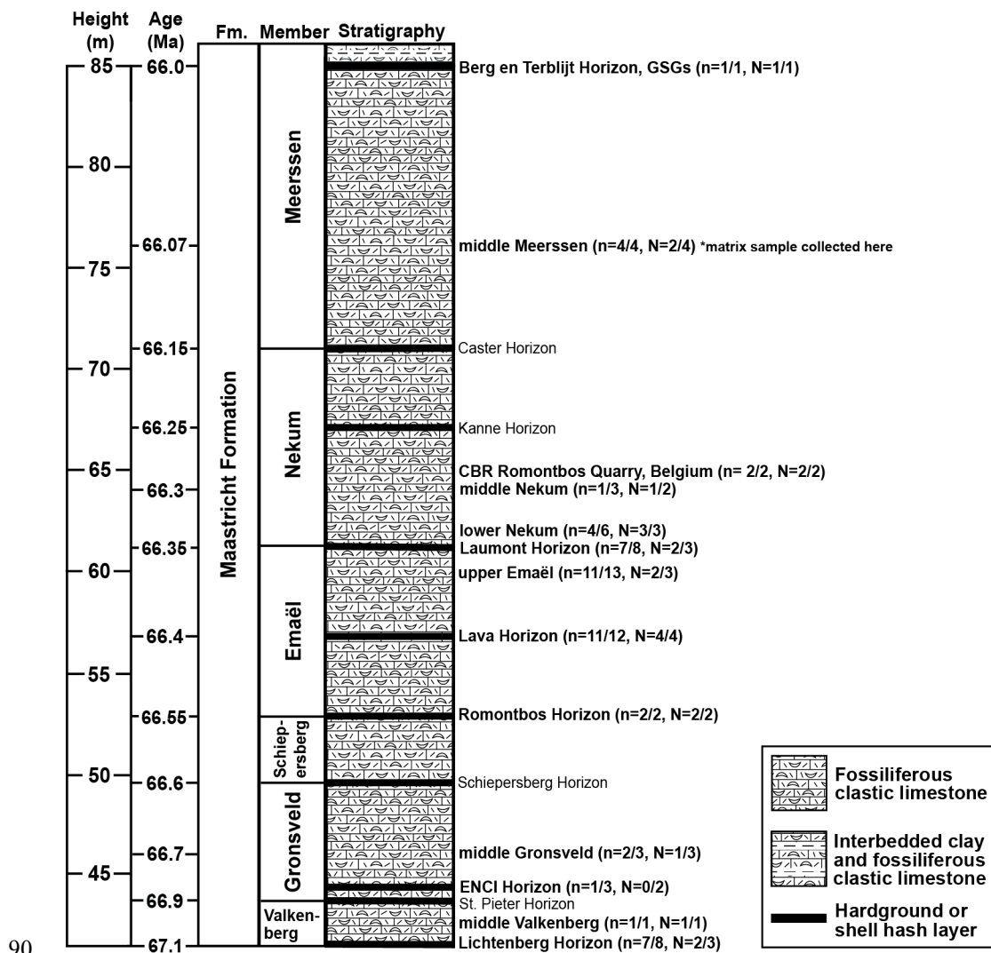
Figure 2: Composite stratigraphic section through the Maastricht Formation at ENCI quarry, Romontbos quarry, and Geulhemmerberg subterranean galleries. Samples collected in the Romontbos quarry and GSGs were placed on the ENCI quarry stratigraphic framework using the age model from Vellekoop et al. (2022) (Table S2). From each collection horizon or zone, the number of specimens collected, the number that passed diagenesis screening, the number of well-preserved specimens successfully analyzed for clumped isotopes and the total number attempted for clumped isotopes (including some
