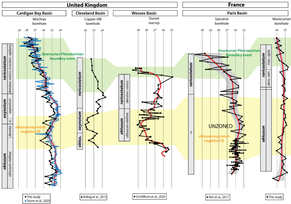
Figure 10: Correlation of negative excursion of \delta^{13}\text{C}_{\text{org}} during Upper Sinemurian in Cardigan Bay Basin (this study, Storm et al., 2020), Cleveland Basin (Riding et al., 2013), Wessex Basin (Schöllhorn et al., 2020) and Paris Basin (this study, Peti et al., 2017).
