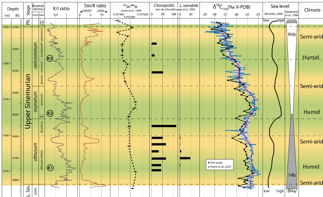
Figure 11: Palaeoclimatic interpretations inferred from clay mineral assemblages expressed by K/I and Sm/K ratios, compared with Classopollis , Liasidium variable abundance and strontium isotopes (Jones et al., 1994; van de Schootbrugge et al., 2005; Riding et al., 2013), carbon isotope variations (this study, Storm et al., 2020). Eustatic and/or regional relative sea-level variations from Hardenbol et al. (1998) and Hesselbo (2008).
