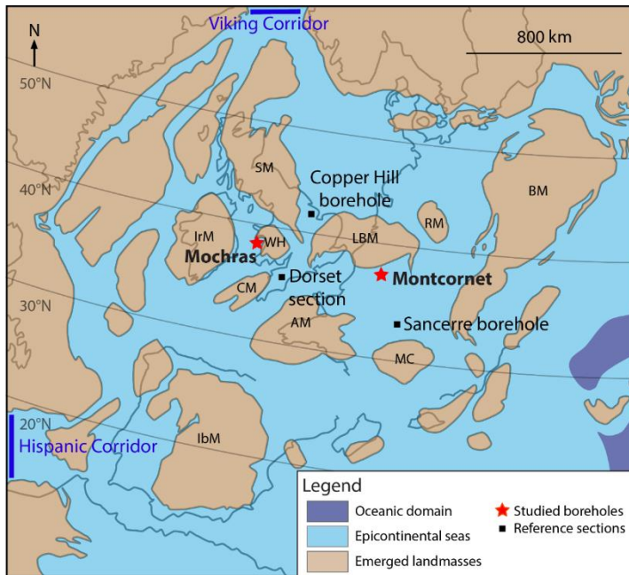
790 Figure 1: Upper Sinemurian palaeogeographical map of the northwest Tethyan domain and position of the studied boreholes (modified from Bougeault et al., 2017). Abbreviations: SM = Scottish Massif; IrM = Irish Massif; CM = Cornubian Massif; WH = Welsh High; LBM = London-Brabant Massif; RM = Rhenish Massif; BM = Bohemian Massif; MC = Massif Central; AM = Armorican Massif; IbM = Iberian Massif.
