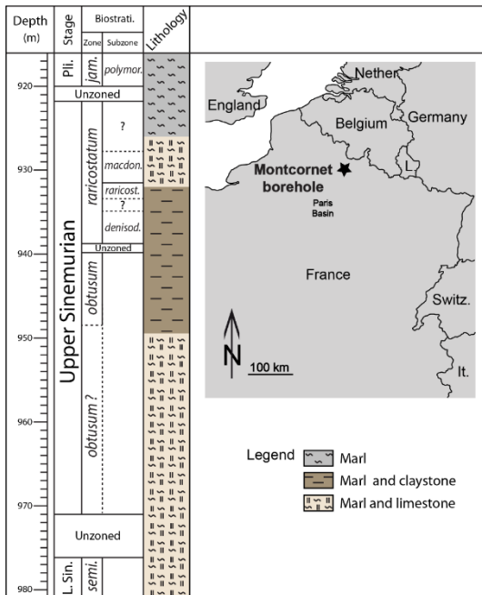
Figure 3: Location map of Montcornet borehole, simplified lithology and biostratigraphy of Upper Sinemurian (from Fauconnier, 1995; Yang et al., 1996). densinod. = densinodulum , jam. = jamesoni , L.Sin = Lower Sinemurian, macdonn. = macdonnelli , Pli. = Pliensbachian, polymor. = polymorphus , raricost. = raricostatium , semi. = semicostatium .
