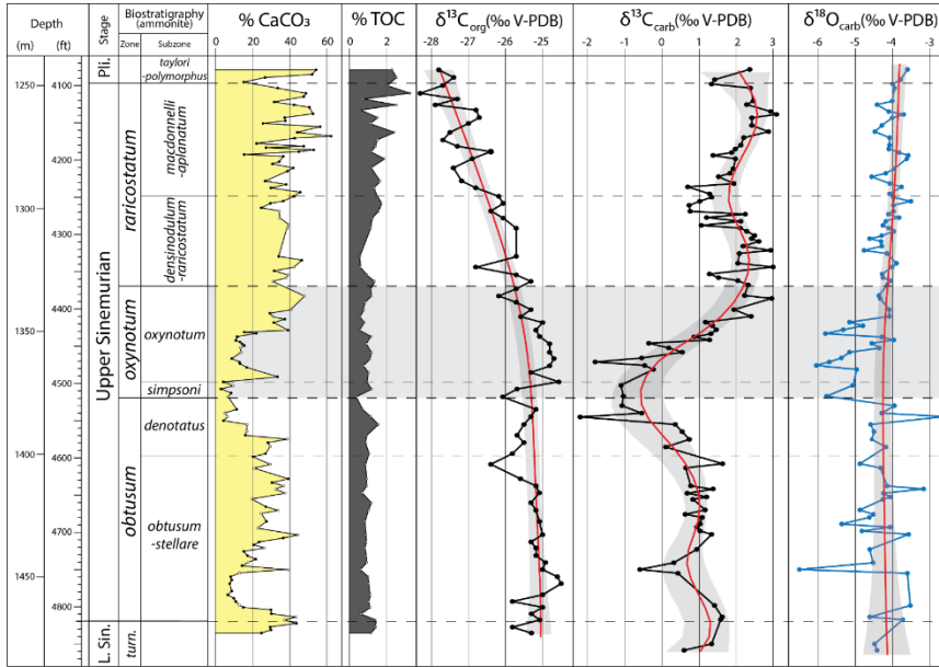
Figure 7: Carbon ( \delta^{13}\text{C}_{\text{carb}} and \delta^{13}\text{C}_{\text{org}} ) and oxygen ( \delta^{18}\text{O}_{\text{carb}} ) isotopes of the Upper Sinemurian on the Mochras borehole coupled with the proportions of \text{CaCO}_3 and TOC. Smoothing curve in red and 95% confidence interval in grey (Kernel regression). L. Sin. = Lower Sinemurian, Pli. = Pliensbachian, turn. = turneri .
