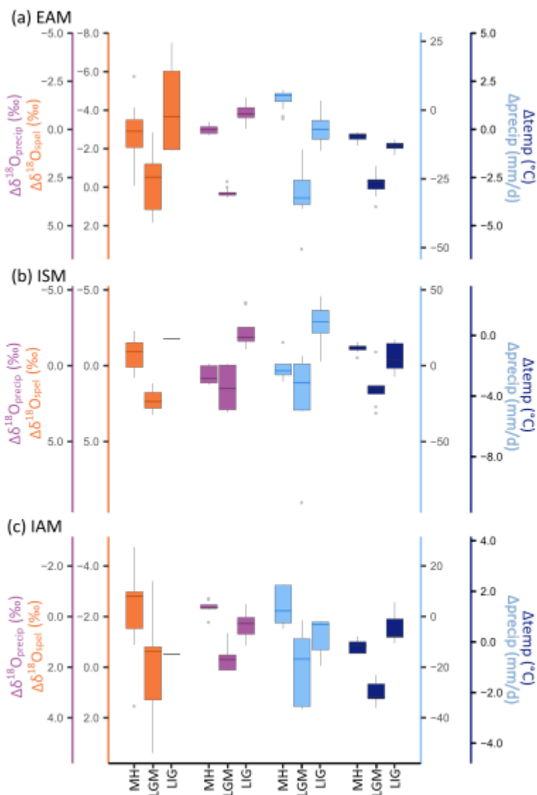
950 Figure 3: Speleothem \delta^{18}\text{O} anomalies compared to anomalies of \delta^{18}\text{O}_{\text{precip}} , precipitation and temperature from the ECHAM simulations for the (a) East Asian (EAM), (b) Indian (ISM) and (c) Indonesian-Australian (IAM) monsoons. The boxes show the median value (line) and the interquartile range, and the whiskers show the minimum and maximum values, with outliers represented by grey dots. Note that the isotope axes are reversed, so that the most negative anomalies are at the top of the plot, to be consistent with the assumed relationship with the direction of change in precipitation and temperature.
