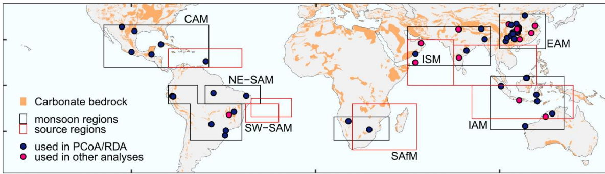
870 Figure 1: Spatial distribution of speleothem records used in this study. Colours indicate the sites used in Principal Coordinates Analysis and Redundancy Analysis (PCoA, RDA) to separate monsoon regions, and sites not used in PCoA and RDA but used in subsequent analyses. The individual regional monsoons are shown by boxes: CAM = Central American Monsoon latitude: 10 to 33°; longitude: -115 to -58°, SW-SAM = southwestern South American Monsoon latitude: -10° to 0°; longitude: -80° to -64° and latitude: -30° to -10°; longitude: -68° to -40°), NE-SAM = northeastern South American Monsoon (latitude: -10° to 0°; longitude: - 875 60° to -30°), SAFm = southern African Monsoon (latitude: -30° to -17°; longitude: 10° to 40°), ISM = Indian Summer Monsoon (latitude: 11° to 32°; longitude: 50° to 95°), EAM = East Asian Monsoon (latitude: 20° to 39°; longitude: 100° to 125°), IAM = Indonesian-Australian Monsoon (latitude: -24° to 5°; longitude: 95° to 135°). Source region limits used in the multiple linear regression analysis are also shown. The background carbonate lithology is from the World Karst Aquifer Mapping (WOKAM) project (Goldschneider et al., 2020).
