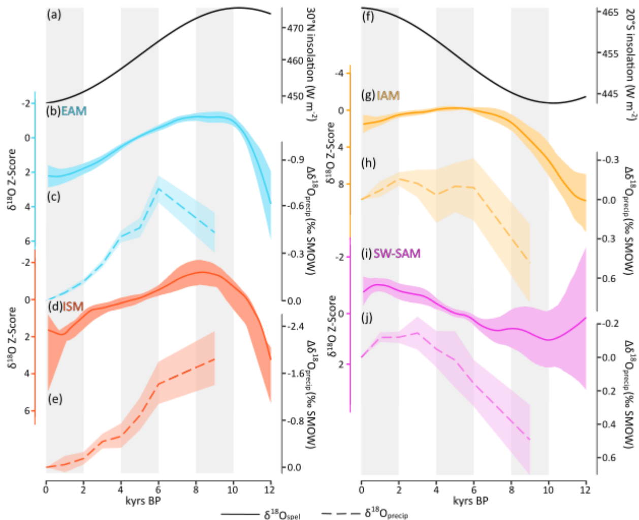
900 Figure 4: Evolution of regional speleothem \delta^{18}\text{O} signals through the Holocene compared to \delta^{18}\text{O}_{\text{precip}} simulated by the GISS model. The left panel shows northern hemisphere monsoons (EAM = East Asian Monsoon; ISM = Indian Summer Monsoon) and summer (May through September) insolation at 30^\circ\text{N} (Berger, 1978). The right panel shows southern hemisphere monsoons (SW-SAM = southwest South American Monsoon; IAM = Indonesian-Australian Monsoon) and summer (November through March) 905 insolation for 20^\circ\text{S} (Berger, 1978). The speleothem \delta^{18}\text{O} changes are expressed as z-scores, with a smoothed loess fit (3,000 year window), and confidence intervals obtained by bootstrapping by site. \delta^{18}\text{O}_{\text{precip}} values are expressed as anomalies from the pre-industrial control simulation. Note that the isotope axes are reversed, so that the most negative anomalies are at the top of the plot, to be consistent with the assumed relationship with the changes in insolation.
