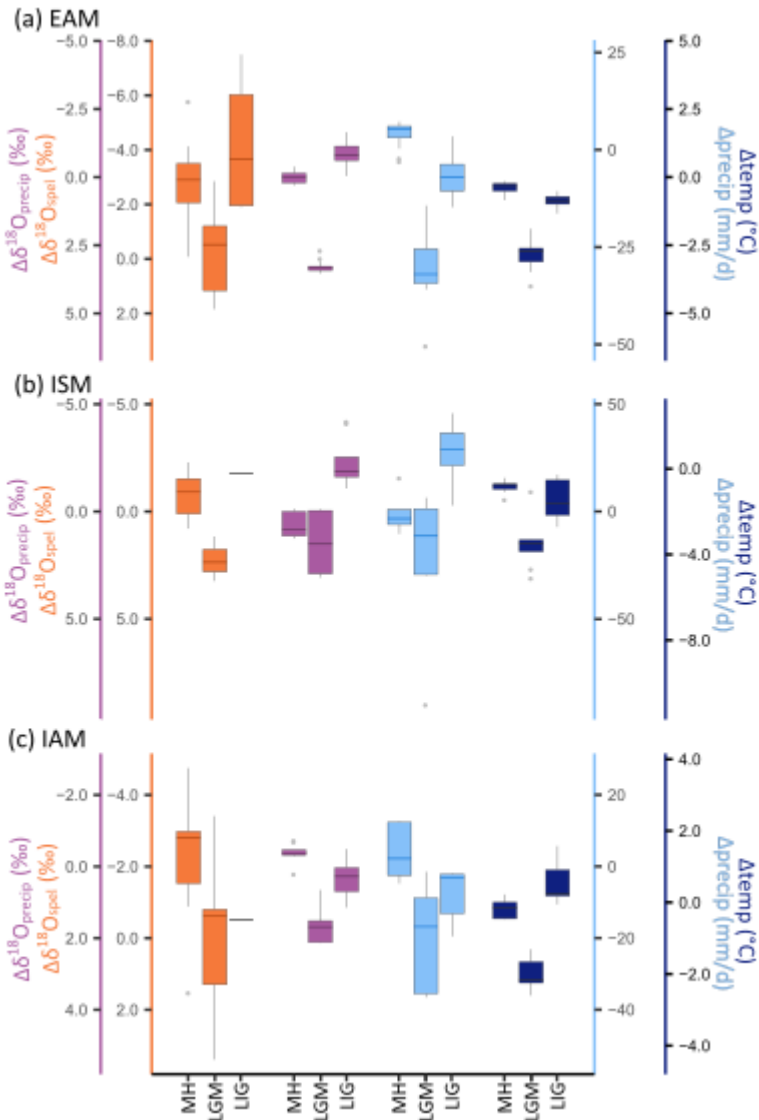
890 Figure 3: Speleothem \delta^{18}\text{O} anomalies compared to anomalies of \delta^{18}\text{O}_{\text{precip}} , precipitation and temperature from the ECHAM simulations for the (a) East Asian (EAM), (b) Indian (ISM) and (c) Indonesian-Australian (IAM) monsoons. The boxes show the median value (line) and the interquartile range, and the whiskers shown the minimum and maximum values, with outliers represented by grey dots. Note that the isotope axes are reversed, so that the most negative anomalies are at the top of the plot, to be consistent with the assumed relationship with the direction of change in precipitation and temperature.
