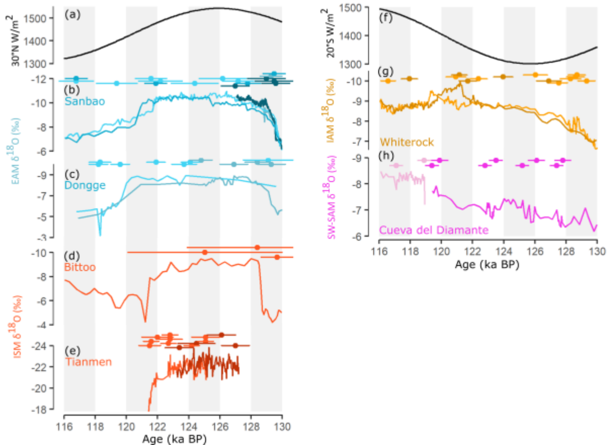
910 Figure 5: Comparison of changes in summer insolation and Last Interglacial \delta^{18}\text{O}_{\text{spe}} records from the (b,c) East Asian Monsoon (EAM), (d,e) Indian Summer Monsoon (ISM), (g) southwest South American Monsoon (SW-SAM) and (h) Indonesian-Australian Monsoon (IAM) regions. The U/Th dates and uncertainties are shown for each record. The summer insolation curves (Berger, 1978) are for May through September at 30^\circ\text{N} in the northern hemisphere (a) and for November through March for 20^\circ\text{S} in the southern hemisphere (f). Note that the isotope axes are reversed, so that the most negative anomalies are at the top of the plot, to be consistent with the assumed relationship with the changes in insolation.
