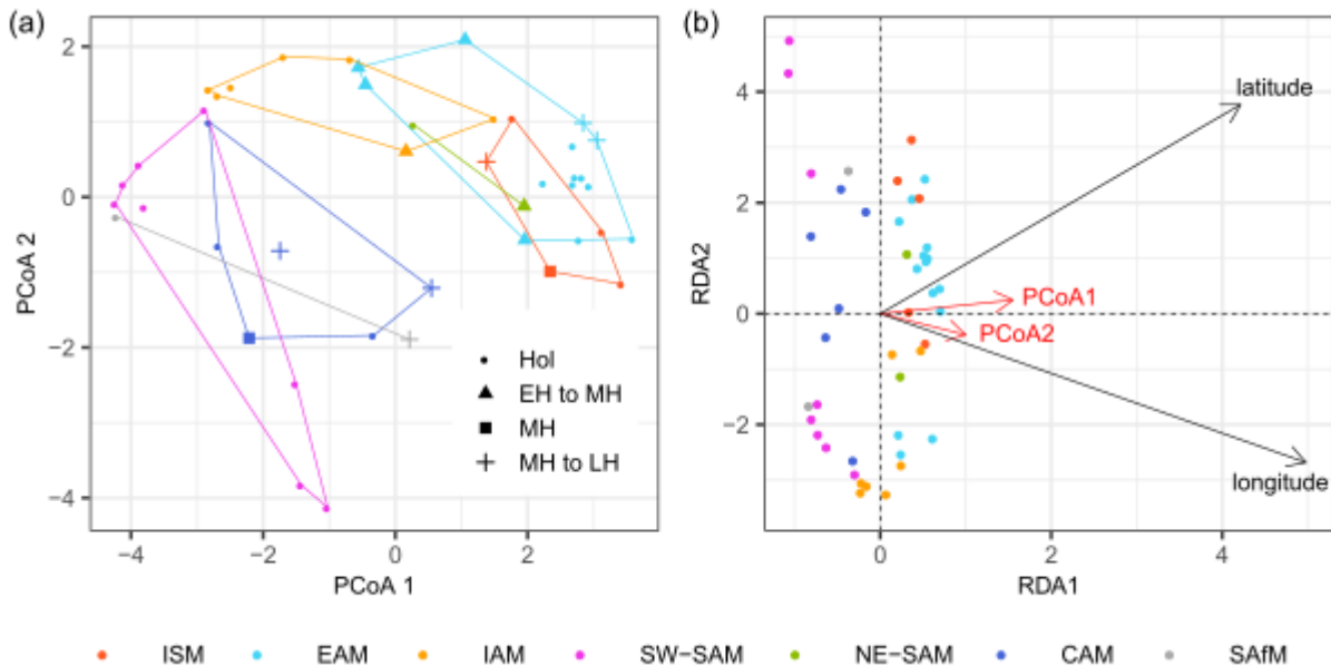
880 (a) PCoA biplot showing the loadings of each site on the first 2 axes, which represent 85% of the total variance. Shapes indicate the Holocene coverage of each site, where sites with a coverage \geq 8000 years represent most or all of the Holocene (Hol). Sites with a temporal coverage of < 8000 years are 885 coded to show whether they represent the early to mid-Holocene (EH to MH, record midpoint > 8,000 years BP), the mid Holocene (MH, record midpoint between 8,000 and 5,000 years BP), or the mid to late-Holocene (LH to MH, midpoint < 5,000 years BP). (b)
