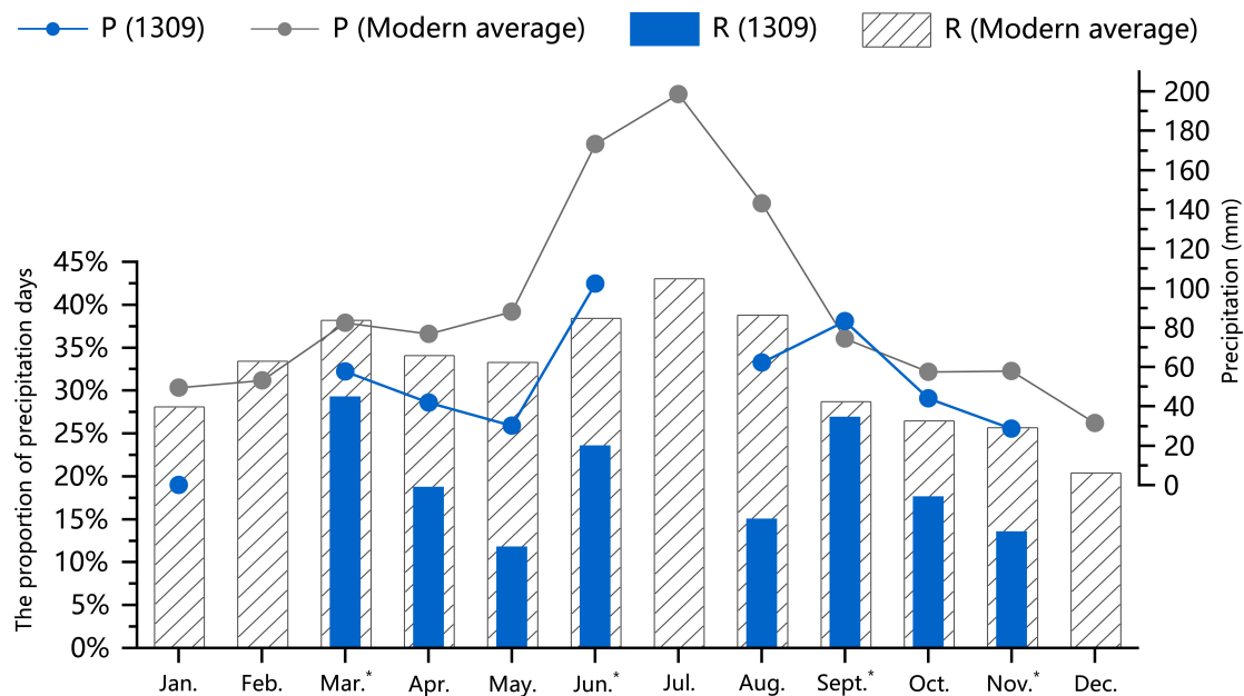
Fig. 1. Precipitation and the proportion of precipitation days in Zhenjiang for each month of 1309 and their comparison with the modern averages
