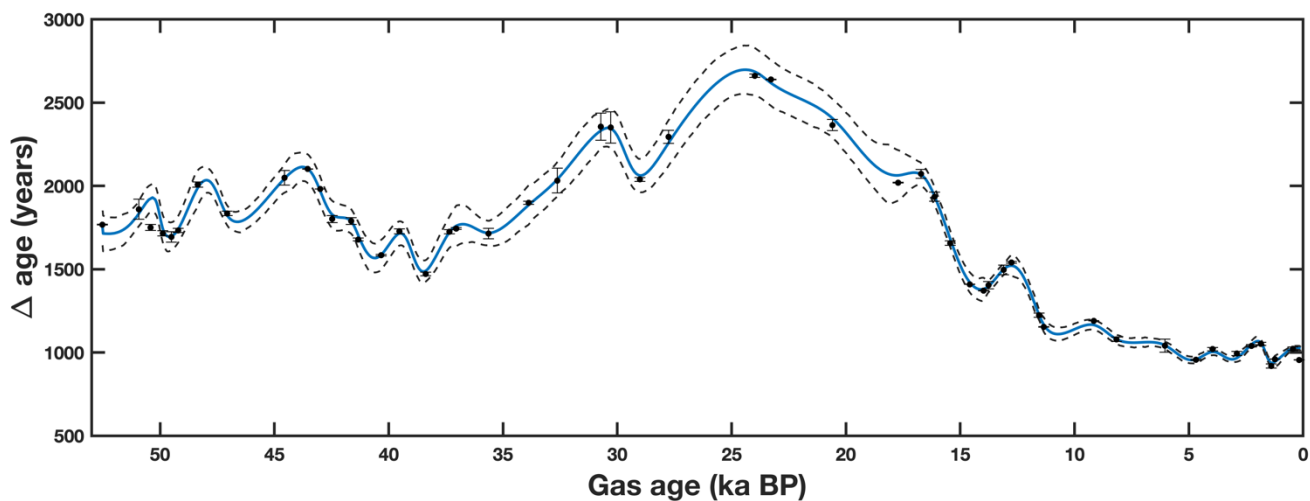
20 Figure 3. Empirically derived \Delta age history for the SPC14 ice core, derived as described in the text. Blue line is a spline fit to the \Delta age points. \Delta age error bounds ( 2\sigma ), dashed lines, reflect uncertainties with \Delta age based on WD \Delta age uncertainty, and relative SP19 uncertainties, black dots indicate individual \Delta age constraints (see text).
