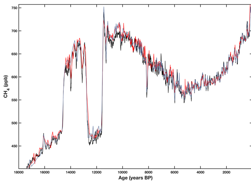
Figure 7. a) SPC14 (blue), WD (black), and RICE (red) all exhibit resolved centennial scale variation in \text{CH}_4 in the Holocene and during the deglaciation. RICE data from (Lee et al., 2020), WD data from (Rhodes et al., 2015).
