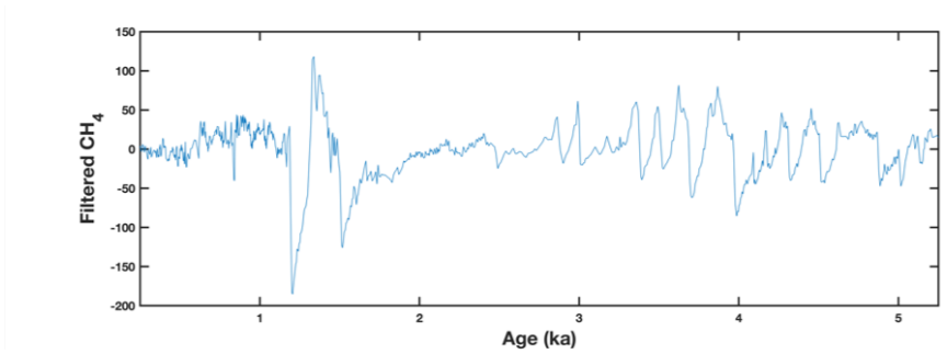
Fig. 1. Filtered CH4 record
