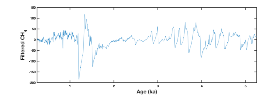
Fig. 1. Filtered CH4 record
