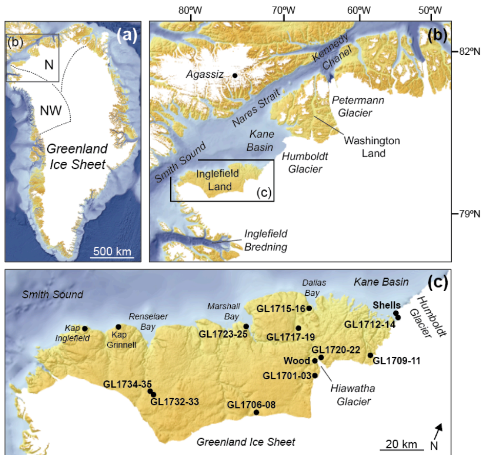
590 Figure 1: Location of the study area in Greenland (a), with marked northwest (NW) and north (N) Greenland extent and places mentioned in the text (b). (c) shows Inglefield Land with places discussed in the text. Black dots denote sample locations for wood fragments in front of the Hiawatha Glacier, molluscs at the margin of the Humboldt Glacier and boulder samples (GL17XX) collected throughout the study area.
