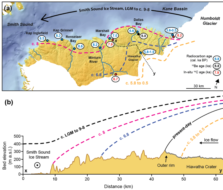
645 Figure 7: Deglaciation in Inglefield Land. (a) shows ages believed to constrain the deglaciation in the area. In-situ ^{14}\text{C} ages and radiocarbon ages at Humboldt Glacier and Hiawatha Glacier are from this study. Radiocarbon ages at the coast are from Nichols (1969), Blake et al. (1992) and Mason (2010). (b) shows the Holocene deglaciation pattern in Inglefield Land inferred from this study across the transect (x-y) seen in (a).
