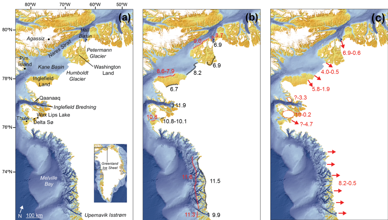
650 Figure 8: Age constraints (in ka) of the Holocene ice extent at the outer coast, present-day ice margin and for the period when the GrIS was smaller than present. (a) shows localities in northwest and north Greenland. (b) shows the initial Holocene deglaciation of the GrIS towards the outer coast (red) (Corbett et al., 2013, Corbett et al., 2015, Jakobsson et al., 2018, Ceperley et al., 2020, Søndergaard et al., 2020) and following retreat towards the present-day ice margin (black) (Briner et al., 2013, McFarlin et al., 2018, Reusche et al., 2018, Axford et al., 2019, Reilly et al., 2019, Søndergaard et al., 2019, Ceperley et al., 2020, Søndergaard et al., 2020). (c) shows the period when the GrIS and 655 its outlets (arrows) and local ice caps (circles) were smaller than the present-day extent (Bennike, 2002, 2008, Briner et al., 2014, Farnsworth et al., 2018, Axford et al., 2019, Reilly et al., 2019, Søndergaard et al., 2019, Søndergaard et al., 2020). A question mark means that the upper limit of restricted ice extent has not been constrained.
