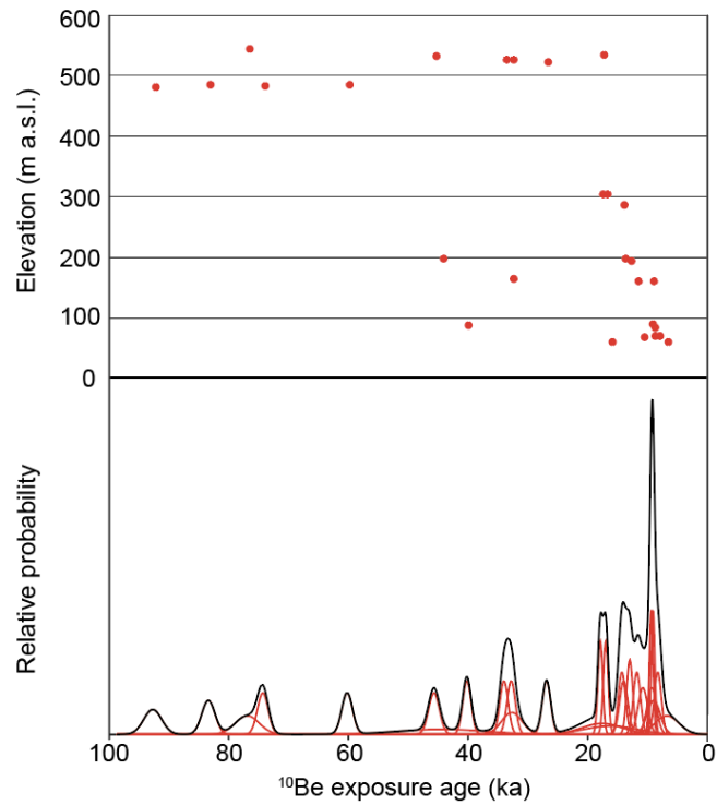
640 Figure 6: ^{10}\text{Be} ages from boulders sampled at various elevations in Inglefield Land, north Greenland. The top panel shows ^{10}\text{Be} ages plotted against elevation of the sample sites. Each red dot represents the ^{10}\text{Be} age of an individual boulder and its associated elevation. The bottom panel shows the relative probability distribution of the boulder ages with their 1\sigma analytical uncertainty (red lines) and the cumulated probability plot of all ^{10}\text{Be} ages (black line).
