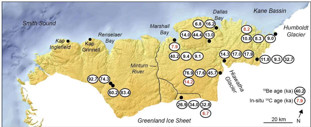
615 Figure 3: Map of Inglefield Land, north Greenland. Black dots denote sample locations for boulder samples and their resulting ^{10}\text{Be} and in-situ ^{14}\text{C} exposure ages given in ka. ^{10}\text{Be} age uncertainties range between 0.3 ka and 7.3 ka with an average of 1.4 ka and ^{14}\text{C} age uncertainties range between 0.3 ka and 0.5 ka with an average of 0.4 ka.
