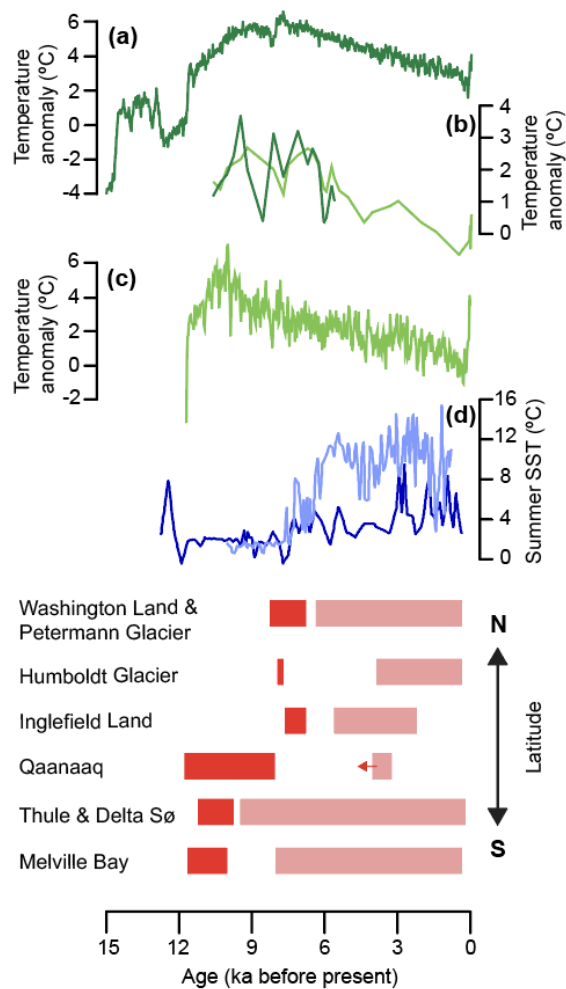
660 Figure 9: Ice extent and climate fluctuations for north and northwest Greenland during the last 15 ka. (a) mean annual temperature anomalies, northwest Greenland (Buizert et al., 2018). (b) July air temperature anomalies at Delta Sø, northwest Greenland, using two different training sets and transfer functions, FOR15 (light green) and FRA06 (dark green) (Axford et al., 2019). (c) Agassiz \delta^{18}\text{O} temperature reconstruction (Lecavalier et al., 2017). (d) Reconstructed west Greenland sea surface temperatures from Gibb et al. (2015) (dark blue) and Ouellet-Bernier et al. (2014) (light blue). The lower panel shows the inferred ice extent in north and northwest Greenland from Melville Bay in the south to Washington Land in the north (for references, see text). Dark red bars denote known periods of deglaciation from the outer coast towards the present-day ice margin and bright red bars denote periods of smaller than present-day extent. Arrows indicate the lack of an upper or lower constraint. 665
