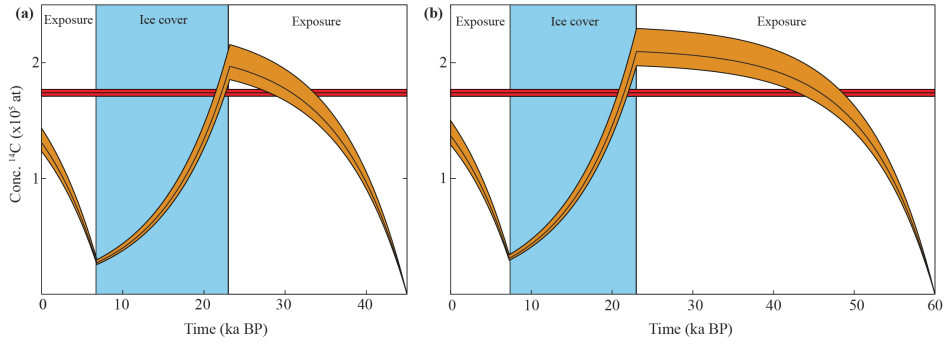
675 Figure 5: Modelled exposure scenario for boulder sample GL1701. The red line shows the measured in-situ ^{14}\text{C} concentration in the sample and the orange line is the nuclide concentration build up and decay during periods of exposure and ice cover. (a) shows exposure from 45 to 23 ka and again from 6.7 ka until present and ice cover in between. (b) shows exposure from 60 to 23 ka and again from 6.7 ka until present and ice cover in between.
