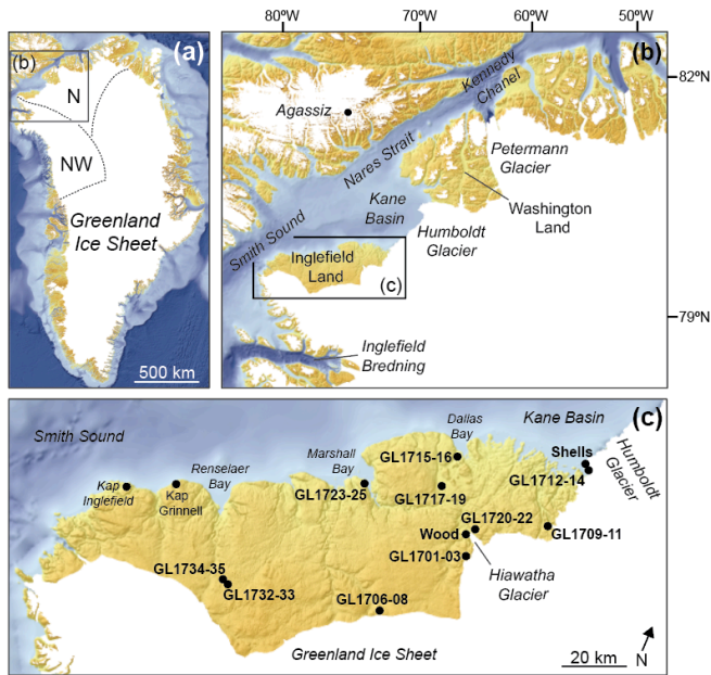
640 Figure 1: Location of the study area in Greenland (a), with marked northwest (NW) and north (N) Greenland extent and places mentioned in the text (b). (c) shows Ingfield Land with places discussed in the text. Black dots denote sample locations for wood fragments in front of the Hiawatha Glacier, molluscs at the margin of the Humboldt Glacier and boulder samples (GL17XX) collected throughout the study area.
