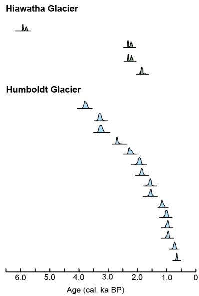
670 Figure 4: Radiocarbon age probability plots of wood fragments collected in front of the Hiawatha Glacier (green) and reworked marine molluscs collected at the margin of Humboldt Glacier (blue). Each plot represents the age of a single wood fragment or mollusc shell and its calibrated age probability distribution.
