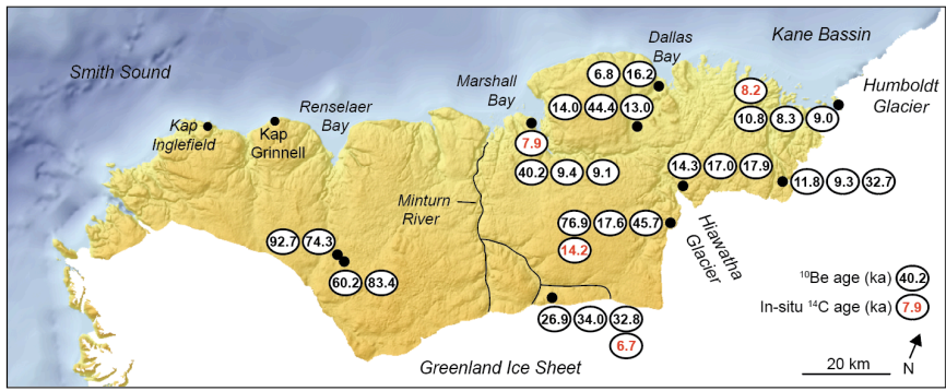
665 Figure 3: Map of Inglefield Land, north Greenland. Black dots denote sample locations for boulder samples and their resulting ^{10}\text{Be} and in-situ ^{14}\text{C} exposure ages given in ka. ^{10}\text{Be} age uncertainties range between 0.3 ka and 7.3 ka with an average of 1.4 ka and ^{14}\text{C} age uncertainties range between 0.3 ka and 0.5 ka with an average of 0.4 ka.
