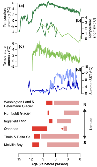
710 Figure 9: Ice extent and climate fluctuations for north and northwest Greenland during the last 15 ka. (a) mean annual temperature anomalies, northwest Greenland (Buizert et al., 2018). (b) July air temperature anomalies at Delta Sø, northwest Greenland, using two different training sets and transfer functions, FOR15 (light green) and FRA06 (dark green) (Axford et al., 2019). (c) Agassiz \delta^{18}\text{O} temperature reconstruction (Lecavalier et al., 2017). (d) Reconstructed west Greenland sea surface temperatures from Gibb et al. (2015) (dark blue) and Ouellet-Bernier et al. (2014) (light blue). The lower panel shows the inferred ice extent in north and northwest Greenland from Melville Bay in the south to Washington Land in the north (for references, see text). Dark red bars denote known periods of deglaciation from the outer coast towards the present-day ice margin and bright red bars denote periods of smaller than present-day extent. Arrows indicate the lack of an upper or lower constraint. 715
