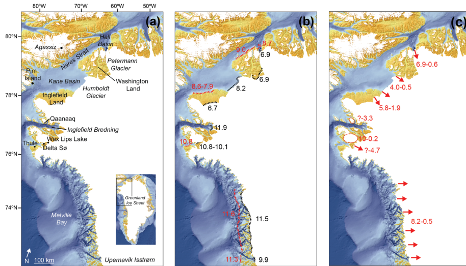
700 Figure 8: Age constraints (in ka) of the Holocene ice extent at the outer coast, present-day ice margin and for the period when the GrIS was smaller than present. (a) shows localities in northwest and north Greenland. (b) shows the initial Holocene deglaciation of the GrIS towards the outer coast (red) (Corbett et al., 2013, Corbett et al., 2015, Jakobsson et al., 2018, Ceperley et al., 2020, Søndergaard et al., 2020) and following retreat towards the present-day ice margin (black) (Briner et al., 2013, McFarlin et al., 2018, Reusche et al., 2018, Axford et al., 2019, Reilly et al., 2019, Søndergaard et al., 2019, Ceperley et al., 2020, Søndergaard et al., 2020). (c) shows the period when the GrIS and 705 its outlets (arrows) and local ice caps (circles) were smaller than the present-day extent (Bennike, 2002, 2008, Briner et al., 2014, Farnsworth et al., 2018, Axford et al., 2019, Reilly et al., 2019, Søndergaard et al., 2019, Søndergaard et al., 2020). A question mark means that the upper limit of restricted ice extent has not been constrained.
