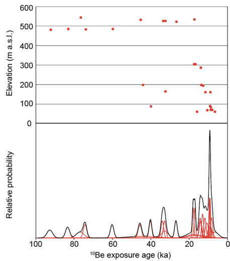
690 Figure 6: ^{10}\text{Be} ages from boulders sampled at various elevations in Ingfield Land, north Greenland. The top panel shows ^{10}\text{Be} ages plotted against elevation of the sample sites. Each red dot represents the ^{10}\text{Be} age of an individual boulder and its associated elevation. The bottom panel shows the relative probability distribution of the boulder ages with their 1\sigma analytical uncertainty (red lines) and the cumulated probability plot of all ^{10}\text{Be} ages (black line).
