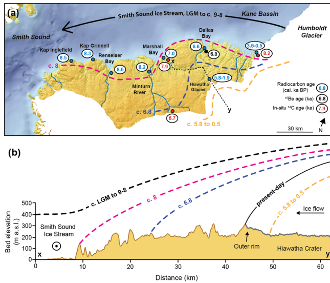
695 Figure 7: Deglaciation in Inglefield Land. (a) shows ages believed to constrain the deglaciation in the area. In-situ 14 C ages and radiocarbon ages at Humboldt Glacier and Hiawatha Glacier are from this study. Radiocarbon ages at the coast are from Nichols (1969), Blake et al. (1992) and Mason (2010). (b) shows the Holocene deglaciation pattern in Inglefield Land inferred from this study across the transect (x-y) seen in (a).
