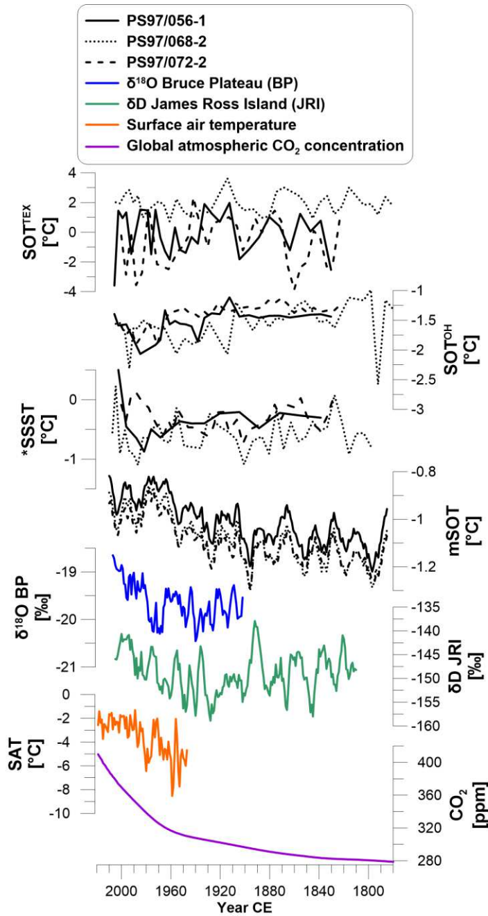
Figure 6: Biomarker derived subsurface ocean temperatures based on \text{TEX}_{86}^L ( \text{SOT}^{\text{TEX}} ), and hydroxylated GDGTs ( \text{SOT}^{\text{OH}} ), and summer sea surface temperatures (SSST) derived from diatom assemblages compared to modelled subsurface ocean temperature (mSOT), stable isotope ice core records from the Bruce Plateau (BP, \delta^{18}\text{O} , 5 year running mean; Goodwin et al., 2016) and from James Ross Island (JRI, \delta\text{D} , 5 year running mean; Abram et al., 2013). Annual means surface air temperature (SAT) is derived from four meteorological stations (annual mean from stations O'Higgins, Faraday/Vernadsky, Bellingshausen and Jubaney, British Antarctic Survey, 2013) and global annual atmospheric carbon dioxide concentrations are combined from Meinshausen et al. (2017) and Tans and Keeling (2020).
