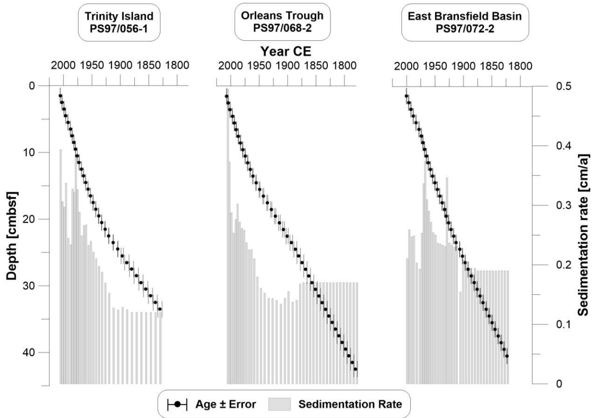
Figure 2: Age-depth models with error bars of all three cores . The sedimentation rate is displayed in grey bars. Ages were extrapolated prior to 1880 CE for all cores based on their average respective sedimentation rate of the three lowermost, reliable dated intervals . All plots were done with Grapher™ 13.
