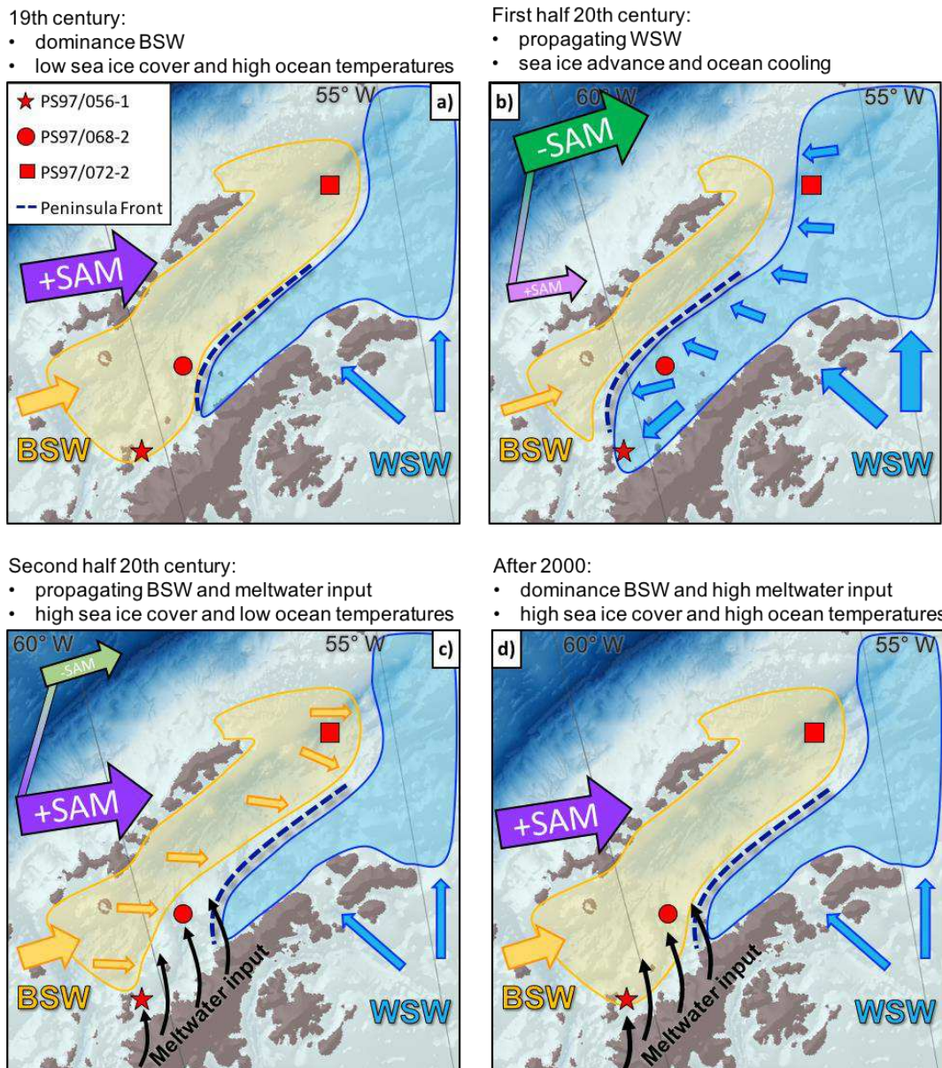
Figure 1 (Figure 8 in the manuscript): The illustration of the four environmental units and their dominant drivers of a) low sea ice cover and high ocean temperatures from dominating BSW described in Unit A, b) moderate winter and spring sea ice cover with decreasing temperatures that propagate from the Weddell Sea to the southern WAP in Unit B, c) high but variable sea ice cover and ocean temperature lows under advancing BSW and +SAM and additional meltwater pulses of Unit C, and d) high sea ice cover under a warm ocean temperature reversal as a result of BSW dominance and meltwater input from the AP in Unit D.
