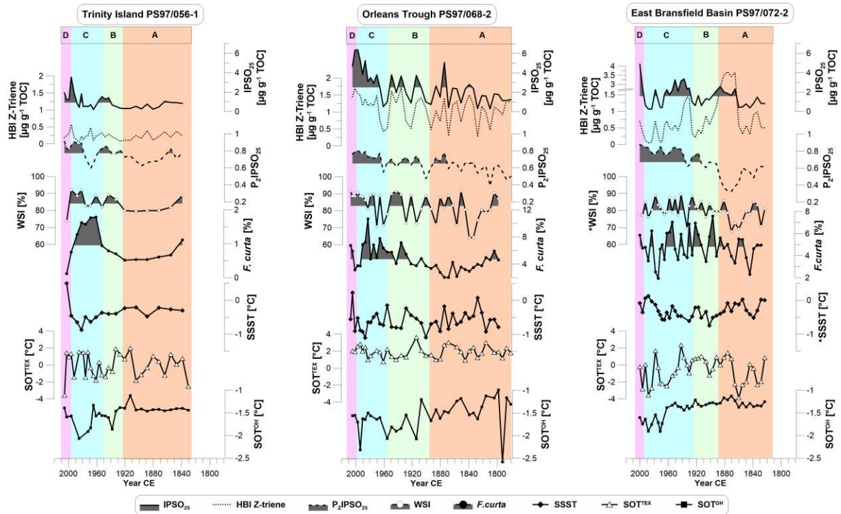
Figure 3: Biomarker composition of the three sediment cores showing concentrations of (from top to bottom) IP SO 25 and HBI Z-trienes, the sea ice index P 2 IP SO 25 , diatom-derived winter sea ice (WSI) concentrations and temperatures of summer sea surface temperatures (SSST), subsurface ocean temperature derived from TEX L 86 (SOT TEX ), and OH-GDGs (SOT OH ). Data marked with * are from the trigger core PS97/072-1. Vertical colored bars denote the environmental units A to D described in section 4.5 . The shadings mark values above the mean of each biomarker in the respective core.
