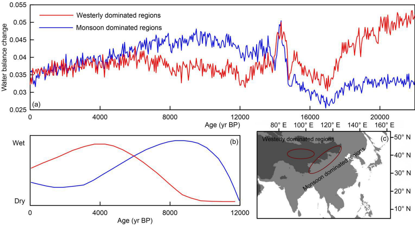
Figure 6. (a) Simulated water balance change between westerly dominated regions and monsoon dominated regions in the Asian closed basins since the LGM, (b) General climate changing patterns during the Holocene in monsoon Asia and westerly Central Asia come from Chen et al. (2006), and (c) Extracted westerly dominated regions and monsoon dominated regions in the Asian closed basins.
