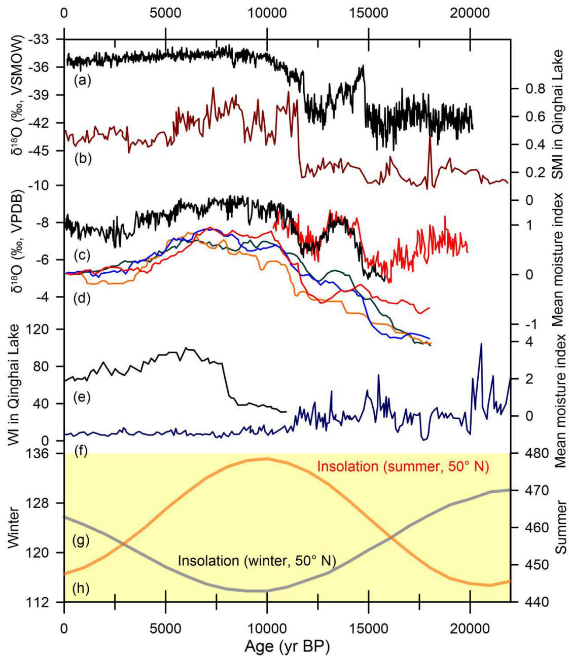
300 Figure 7. Comparison of records between the westerly and monsoon regions of the Northern Hemisphere. (a) NGRIP \delta^{18}\text{O} (Rasmussen et al., 2006); (b) Lake Qinghai Westerlies climate index (An et al., 2012); (c) Dongge and Hulu cave speleothem \delta^{18}\text{O} records (Dykoski et al., 2005; Wang et al., 2008); (d) moisture indexes in East Asian Monsoon (red line), East African Monsoon (green line), Indian Monsoon (blue line) and Australian Monsoon (orange line) regions (Wang et al., 2017); (e) The average moisture index for arid central Asian region as a whole during the Holocene (An and Chen, 2009); (f) Lake Qinghai
