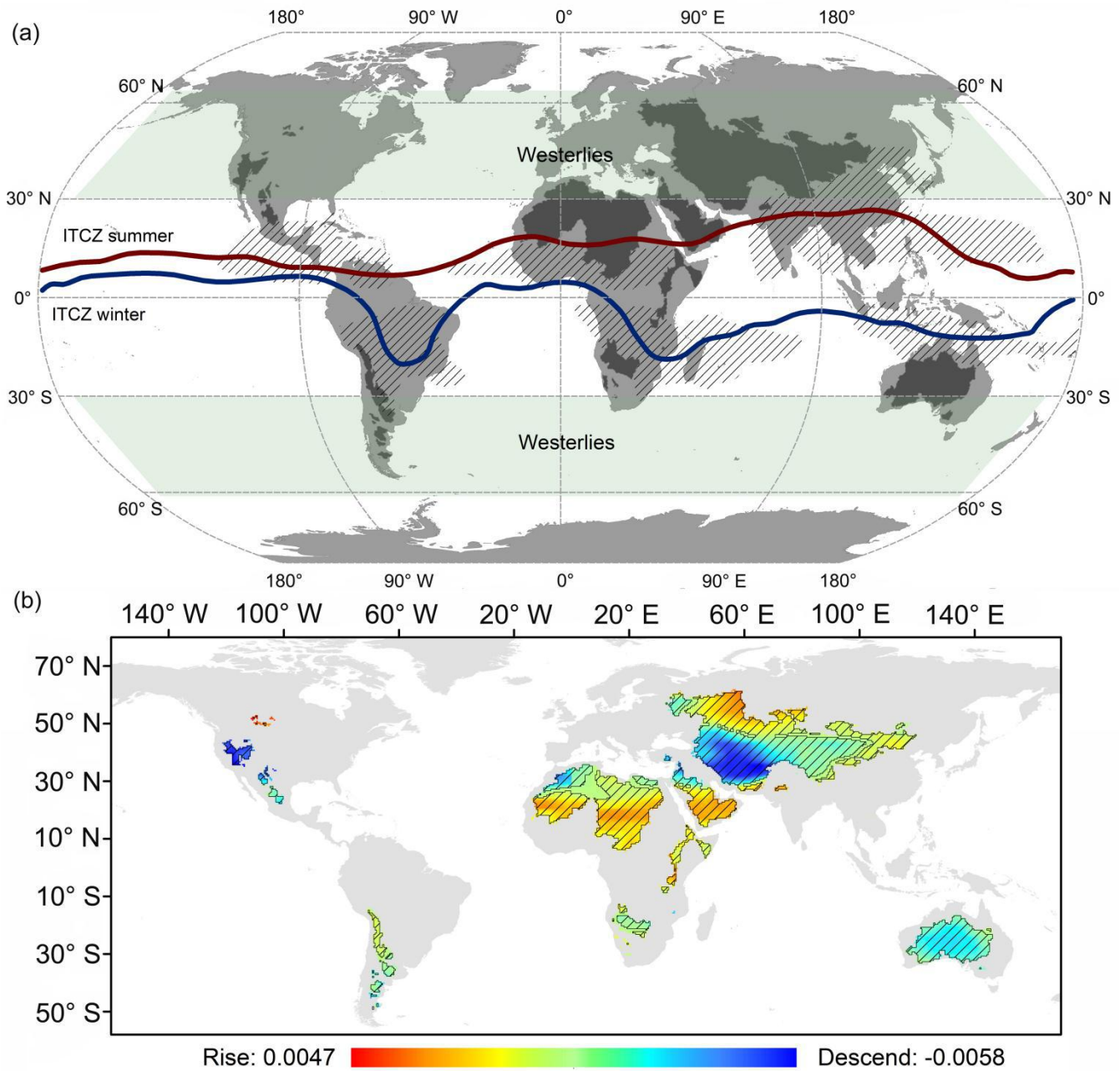
Figure 2. (a) Distribution of global closed basins and circulation system: The dark areas are global closed basins; summer
