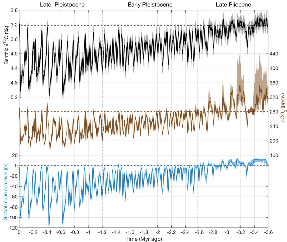
Figure 4: Observed benthic \delta^{18}\text{O} (black; Lisiecki and Raymo, 2005) and reconstructed CO 2 (brown) and global mean sea level (blue) for the entire 3.6 Myr simulation period. The present-day values for the three variables (pre-industrial value of 280 ppmv for CO 2 ) are shown by horizontal dashed lines. Shaded areas indicates the uncertainty in the LR04 benthic \delta^{18}\text{O} stack, and the resulting uncertainty in the reconstructed CO 2 and sea level.
