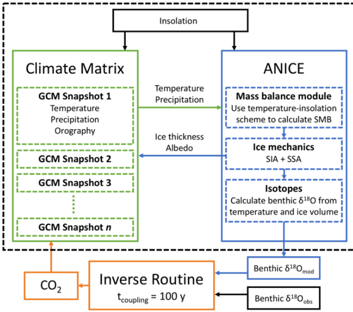
Figure 2: A conceptual visualization of the inverse forward modelling approach. The model is forced externally by an insolation reconstruction and a benthic \delta^{18}\text{O} record (black boxes). p\text{CO}_2 is changed over time based on the difference between observed and modelled \delta^{18}\text{O} . The climate matrix interpolates between the pre-calculated GCM snapshots, based on the prescribed p\text{CO}_2 value and the modelled state of the cryosphere (ice thickness and albedo), to determine the climate that is used to calculate the surface mass balance over the ice sheets. The modelled ice sheets and climate are then used to calculate a modelled benthic \delta^{18}\text{O} value, which is used to update modelled \text{CO}_2 in the next time step. Figure adapted from Berends et al. (2019).
