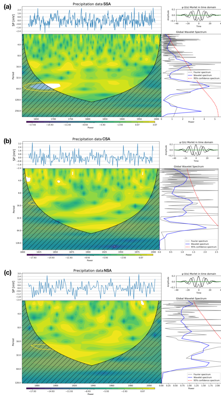
245 Figure 7: The wavelet power spectrum of the reconstructed precipitation at the SSA (a), CSA (b) and NSA (c); powers are given in \log_2 -scale. Significant are the periods that in the graph on the right intersect the dashed red region of significance (blue curve), constructed for a significance level of 0.05. At the top of the graph is a time series and to the right is the view of the used mother wavelet. By hatching on the wavelet transform graph (this graph is filled), the influence cone is indicated. Values falling into the
