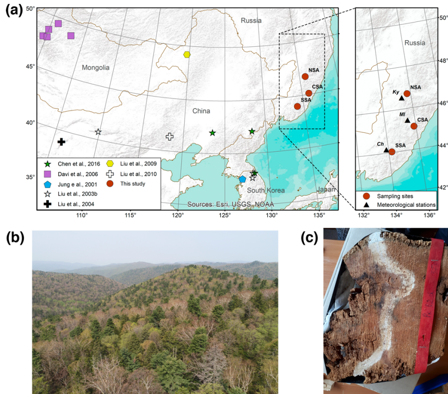
80 Figure 1: Location of the study area. (a) Location of the sample sites of this study and nearest study areas with precipitation reconstructions in continental Northeast Asia. SSA, CSA and NSA are the southern, central and north-western Sikhote-Alin Mountains, respectively; Ch, MI and KY are the Chuguevka, Melnichnoe and Krasniy Yar meteorological stations, respectively. Basemap: Esri. "Topographic" [basemap]. Scale Not Given. "World Topographic Map". June 14, 2013. http://www.arcgis.com/home/item.html?id=30e5fe3149c34df1ba922e6f5bbf808f . (April 07, 2020). (b) Korean pine-broadleaved forest at the SSA site in late spring; tallest conifer trees are Korean pine. (c) Wood sample obtained from dead Korean pine tree.
