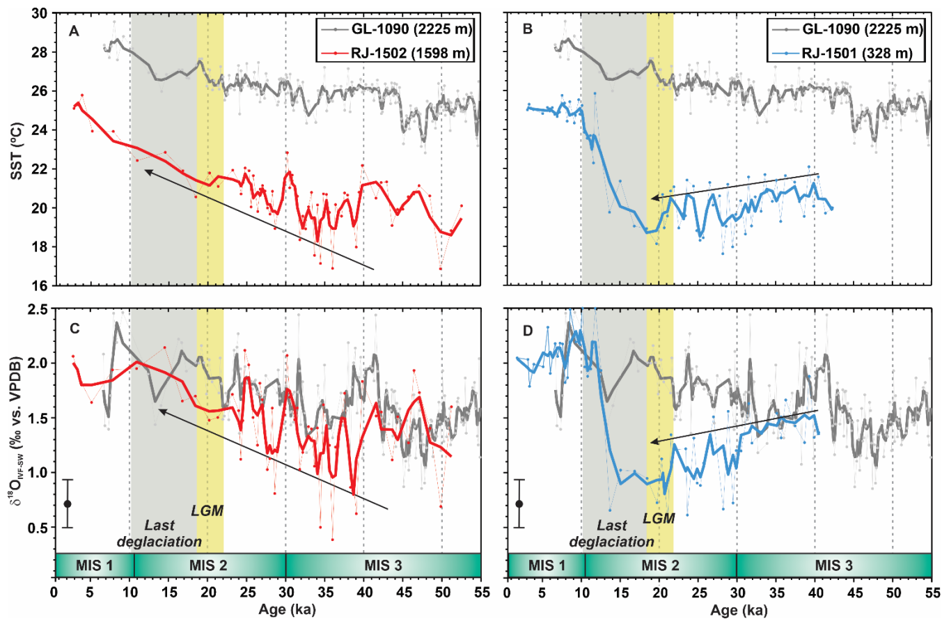
85 Figure 4 – Comparison of the records from marine sediment cores RJ-1501 (blue), RJ-1502 (red) (this study) and GL-1090 (grey) (Santos et al., 2017a). A and B: Alkenone ( U_{37}^K )-derived sea surface temperature (SST) from cores RJ-1502 and RJ- 1501 and Mg/Ca-derived SST from core GL-1090. C and D: Ice-volume free seawater oxygen isotope ( \delta^{18}\text{O}_{\text{IVF-SW}} ) from cores RJ-1502, RJ-1501 and GL-1090. Records are depicted by the original data (dots and thin line) and the respective three-point running average (thick line). Yellow and grey bars denote the Last Glacial Maximum (LGM) and last deglaciation, 80 respectively. The vertical bars at the left of panel C and D indicate the total uncertainty associated with the \delta^{18}\text{O}_{\text{IVF-SW}} . Marine Isotope Stages (MIS) are indicated at the bottom of the panel.
