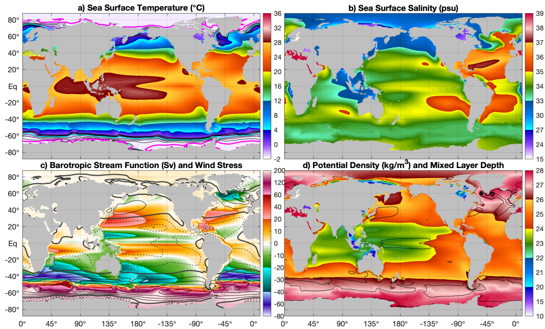
Figure S3. Annual mean for the pre-industrial reference simulation with sea surface a) temperature and b) salinity, c) barotropic stream function (shading, positive for clockwise flow) and zonal wind stress (contours every 5 \cdot 10^{-2} Pa, solid positive and dashed negative, thick line at 0 Pa), and d) upper 200m average potential density (shading) and mixed layer depth (contour lines at 100m and 200m, thick line at 500m). Note the different colour scales in a), c) compared to Figures 3 and S4). Contours in a) show annual mean sea ice fraction at 10% intervals, thick cyan line at 50% and magenta at 90%.
