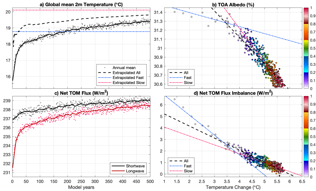
Figure S15. Modelled response after an instant quadrupling of atmospheric CO 2 , starting from the equilibrated state of the pre-industrial reference. a) Annual mean globally averaged near surface air temperature (dots; thick line: using a 25-year smoothing window) with the dashed black line showing the extrapolated response to that point (similarly in blue: extrapolation using years 1–20 and red: using years 101–500). b) Top of the atmosphere albedo: annual (markers; coloured to normalised model time) and linear interpolation (black: all, blue: years 1–20 and red: years 101–500). c) Top of model net shortwave (black) and longwave flux (red): yearly (dots) and smoothed (lines). d) Top of model flux imbalance (shortwave - longwave, see c) ) versus globally averaged temperature change (from the pre-industrial reference): annual (markers) and interpolated (lines; as in b) ).
