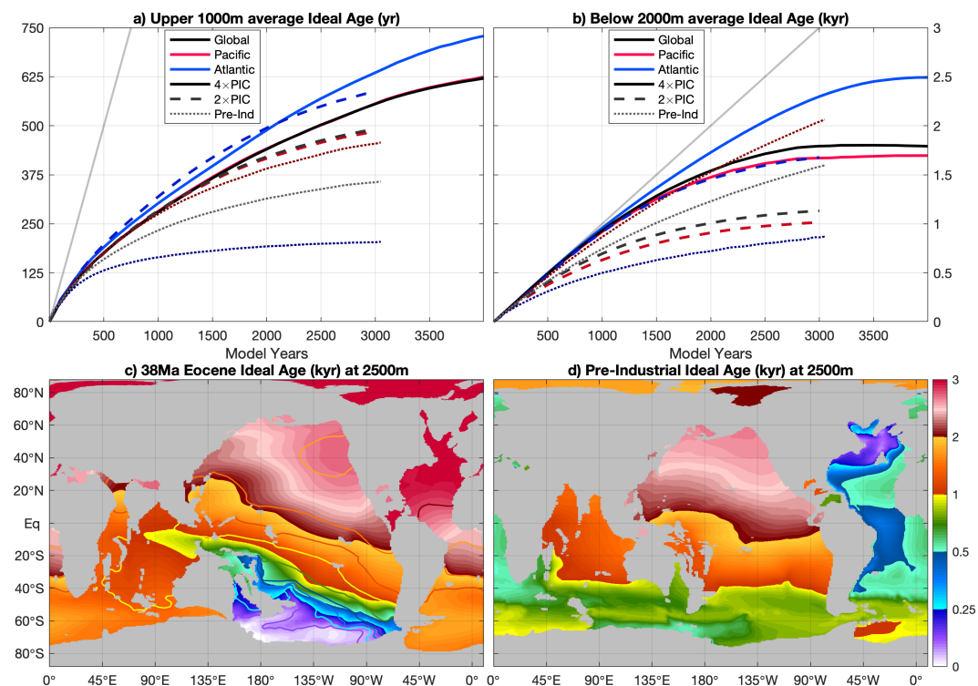
Figure S1. Time series of a) upper 1km and b) below 2km volume-weighted average ideal age tracers for Pre-Industrial (dotted), 38Ma 2× PIC (dashed) and 4× PIC (solid) spin-up simulations. Averages are shown globally (black) and for both the Pacific (red) and Atlantic (blue) ocean basins separately. c) 38Ma and d) pre-industrial horizontal distributions of ideal age tracers at 2500m depth for the end of each model simulation. Colour shading in c) shows the ideal age of 4× PIC, while contours do so for the 2× PIC case (using the same colourmap shown to the right).
