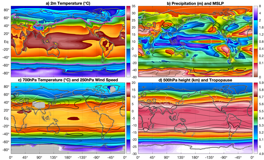
Figure S5. Annual mean for the pre-industrial reference simulation with a) near surface (2m) air temperature (shading) and average min/max temperature (contours; magenta: T_{min} < 0^{\circ}\text{C} , cyan: T_{min} < -10^{\circ}\text{C} , blue: T_{min} < -20^{\circ}\text{C} ), b) precipitation (shading) and mean sea level pressure (contours every 5hPa, thick black lines every 20hPa, \leq 1000\text{hPa} in black and > 1000\text{hPa} in white), c) 700hPa temperature (shading) and 200hPa wind speed (contours every 5m/s starting at 10m/s; white for < 20\text{m/s} and black for > 20\text{m/s} , thick black lines every 20m/s), and d) 500hPa geopotential height (shading) and tropopause height (contours every 1km starting at 12km; white for < 15\text{km} and black for > 15\text{km} , thick black line at 15km). Note the different colour scales in a), c), d) compared to Figures 4 and S6).
