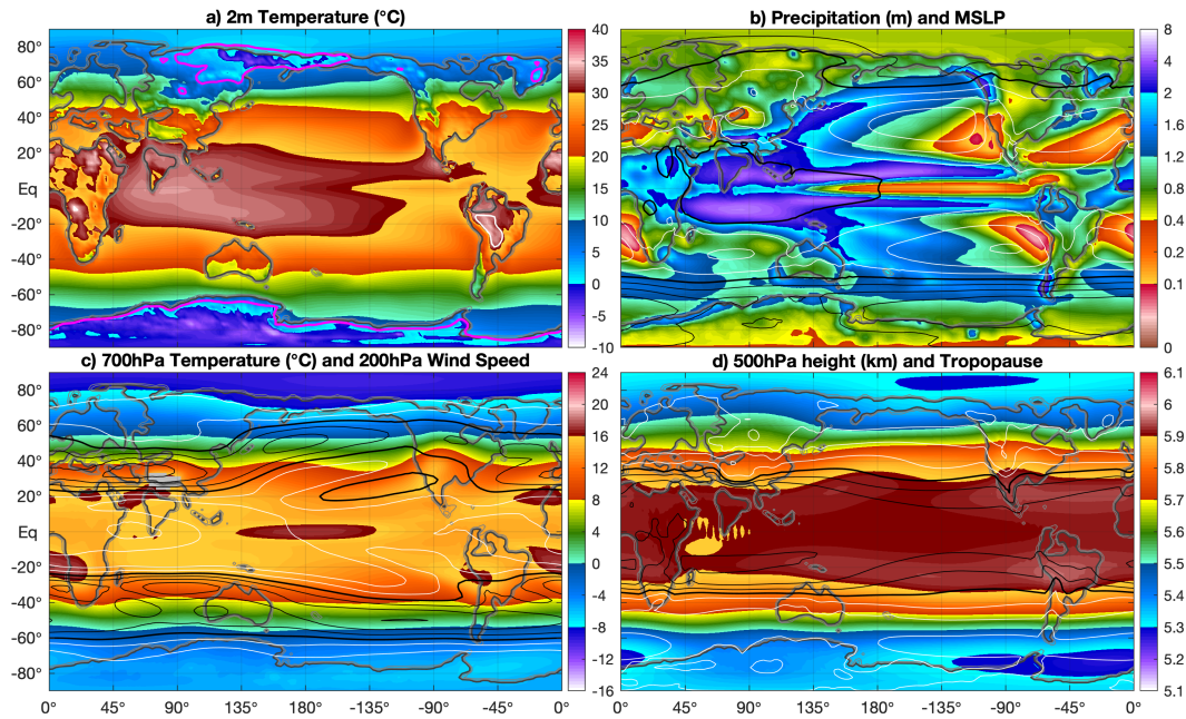
Figure S6. Annual mean for the 38Ma 2\times PIC simulation with a) 2m above ground level air temperature (shading) and average min/max temperature (contours; magenta: T_{min} < 0^\circ\text{C} and white: T_{max} > 40^\circ\text{C} ), b) precipitation (shading) and mean sea level pressure (contours every 5hPa, thick black lines every 20hPa, \leq 1000\text{hPa} in black and > 1000\text{hPa} in white), c) 700hPa temperature (shading) and 200hPa wind speed (contours every 5m/s starting at 10m/s; white for < 20\text{m/s} and black for > 20\text{m/s} , thick black lines every 20m/s), and d) 500hPa geopotential height (shading) and tropopause height (contours every 1km starting at 12km; white for < 15\text{km} and black for > 15\text{km} , thick black line at 15km).
