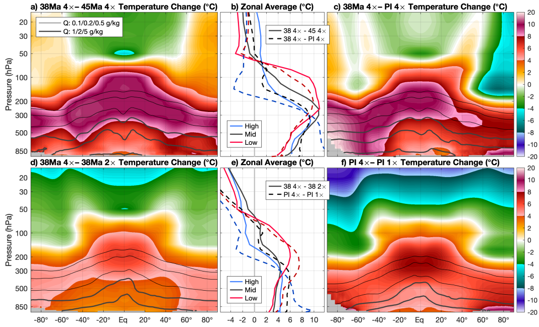
Figure S14. Zonally averaged temperature (shading) and humidity (contours) difference for a) 38Ma 4× PIC versus 45Ma 4× CO 2 (GH14), c) 38Ma 4× PIC versus the pre-industrial reference, d) 38Ma 4× PIC versus 38Ma 2× PIC, and f) pre-industrial 4× CO 2 versus the pre-industrial reference. Meridionally averaged temperature changes are shown in the b) and e) for low (0–30°; red), middle (30–60°; black) and high (60–90°; blue) latitudes, respectively (both hemispheres). Solid lines correspond to the pattern shown to the left, dashed lines to the one to the right.
