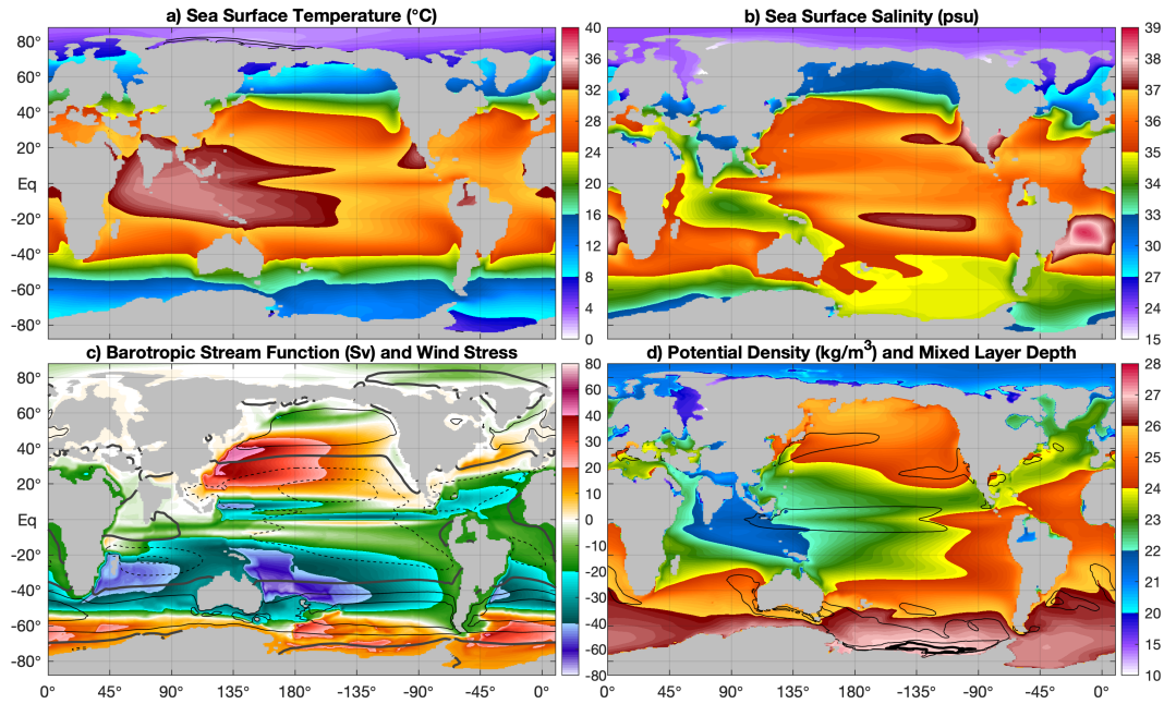
Figure S4. Annual mean for the 38Ma 2× PIC simulation with a) temperature and b) salinity, c) barotropic stream function (shading, positive for clockwise flow) and zonal wind stress (contours every 5 \cdot 10^{-2} Pa, solid positive and dashed negative, thick line at 0 Pa), and d) upper 200m average potential density (shading) and mixed layer depth (contour lines at 100m and 200m, thick line at 500m). Contours in a) show annual mean sea ice fraction at 10% intervals.
