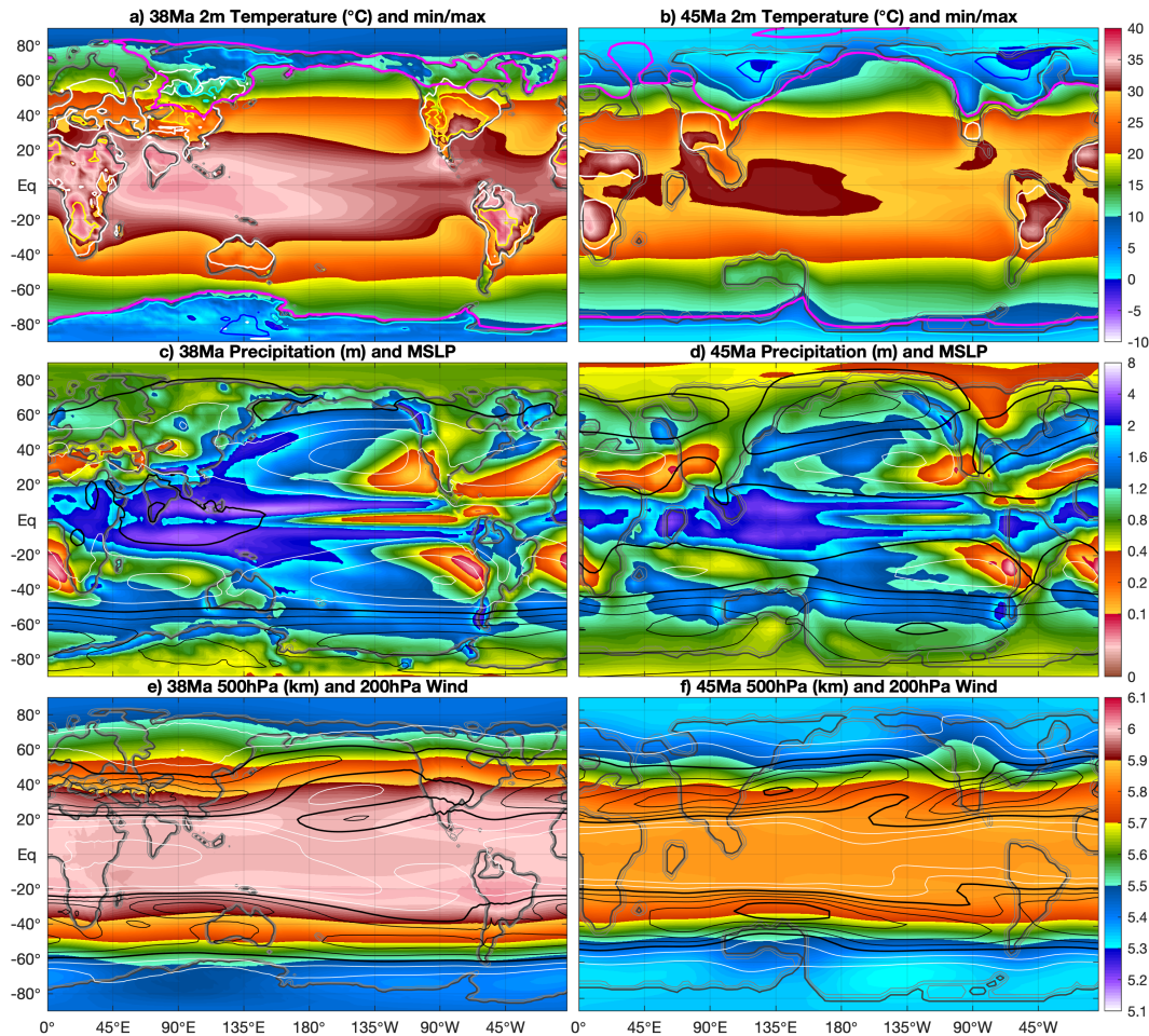
Figure S13. Annual mean (shading), warmest monthly maximum (white: 40°C and yellow: 50°C) and coldest monthly minimum (magenta: 0°C, cyan: -10°C, blue: -20°C) near surface air temperature for the a) 38Ma 4\times PIC simulation (this study) and b) from Goldner et al. (2014) (GH14) using a 45Ma geography and 4\times pre-industrial CO 2 . A similar comparison is made in c) and d) for precipitation (shading) and mean sea level pressure (contours every 5hPa, thick black lines every 20hPa, \leq 1000 hPa in black and >1000 hPa in white), as well as in e) and f) for 500hPa geopotential height (shading) and 200hPa wind speed (contours every 5m/s starting at 10m/s; white for <20 m/s and black for >20 m/s, thick black lines every 20m/s). All colour scales and contour intervals meet the same conventions as those used in Figures 4 and S6.
