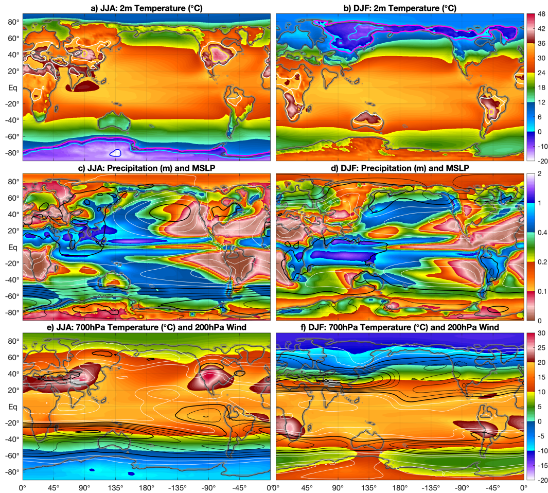
Figure S8. 38Ma 4 × PIC a) June-July-August and b) December-January-February mean 2m air temperature (shading) and average min/max temperature (contours; magenta: T_{min} < 0^{\circ}\text{C} , cyan: T_{min} < -10^{\circ}\text{C} , blue: T_{min} < -20^{\circ}\text{C} , white: T_{max} > 40^{\circ}\text{C} and yellow: T_{max} > 50^{\circ}\text{C} ), c) and d) similar to a) and b) for total precipitation (shading) and mean sea level pressure (contours every 5hPa, thick black lines every 20hPa, \leq 1000\text{hPa} in black and > 1000\text{hPa} in white), and e) and f) for 700hPa temperature (shading) and 200hPa wind speed (contours every 5m/s starting at 10m/s; white for < 20\text{m/s} and black for > 20\text{m/s} , thick black lines every 20m/s).
