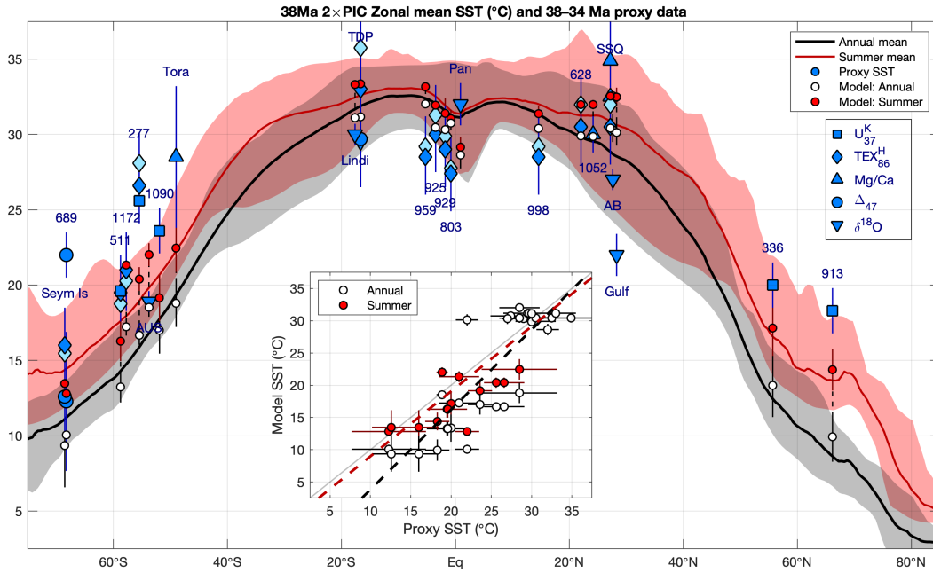
Figure S9. Zonally averaged annual mean (black) and summer mean (red) SST, shaded regions showing zonal spread for the 38Ma 2× PIC case. Blue markers indicate SST proxy estimates, whereas white (annual) and red (summer) circles depict model values at the corresponding 38Ma locations. Error bars represent proxy calibration errors and the model spatial variation within a 4^\circ \times 4^\circ box. The inset shows a scatter plot of model versus proxy SST, with a linear fit using annual mean (black) or summer mean (red; only outside of the tropics) model values.
