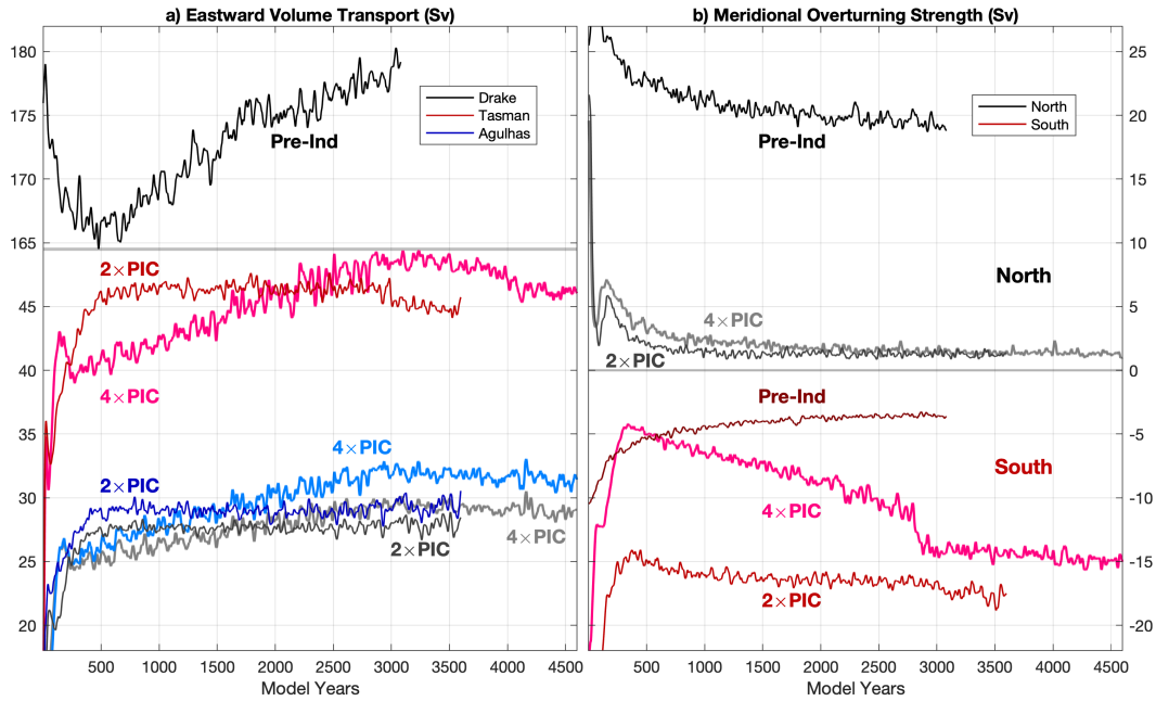
Figure S2. Time series of a) Southern Ocean Gateway volume transports and b) maximum global meridional overturning for both 2\times PIC (dashed), 4\times PIC (solid) Eocene and pre-industrial (dotted) spin-up simulations. Transports through three (one for pre-industrial) north-south transects in the Southern Ocean are considered: Drake Passage (black, 65^\circ W), Tasmanian Gateway (red, 150^\circ E) and Agulhas (blue, 25^\circ E), with positive values indicating eastward flow.
