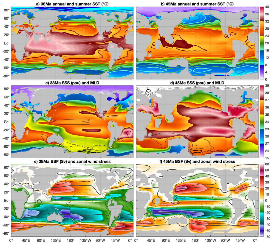
Figure S12. Annual mean (shading) and summer (contours every 2°C) sea surface temperatures for the a) 38Ma 4× PIC simulation (this study) and b) from Goldner et al. (2014) (GH14) using a 45Ma geography and 4× pre-industrial CO 2 . A similar comparison is made in c) and d) for sea surface salinity (shading) and mixed layer depth (contour lines at 100m and 200m, thick line at 500m), as well as in e) and f) for barotropic stream function (shading) and zonal wind stress (contours every 5·10 -2 Pa; solid positive and dashed negative, thick line at 0Pa). All colour scales and contour intervals meet the same conventions as those used in Figures 3 and S4.
