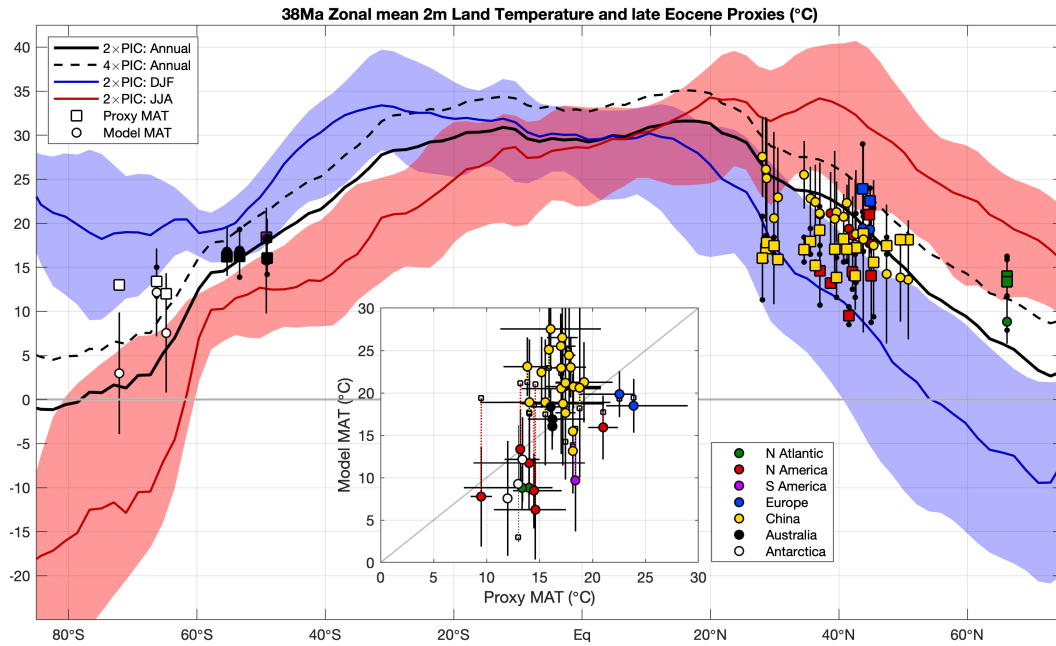
Figure S11. Zonally averaged annual mean (black), December–February (blue) and June–August (red) near surface air temperature (land-only) for the 38Ma 2× PIC case (solid line; dashed: 4× PIC). Red and blue shading indicates zonal variability of the according seasonal averages. Markers show late Eocene proxy estimates (squares) and corresponding model annual mean (circles), colour coded for their respective region. Error bars (black dots) are indicative of the spread at each site (proxies) or spatial variation in a 5^{\circ} \times 4^{\circ} box (model). The inset shows a scatter plot of model versus proxy air temperatures, the former being corrected for differences in model and reconstructed topography (uncorrected: small squares).
