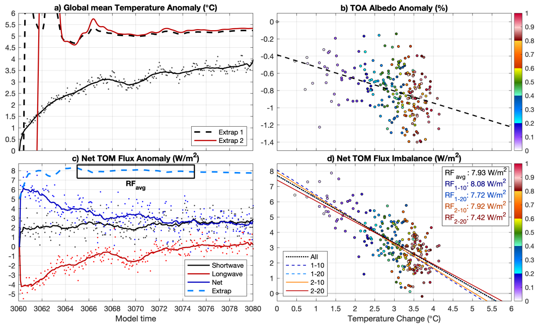
Figure S16. First 20 years of the response after an instant quadrupling of atmospheric CO 2 , starting from the equilibrated state of the pre-industrial reference. Model years 3060–3080 for both the reference and 4\times CO 2 simulations are considered, of which the monthly mean output fields are compared 1 on 1. The respective differences are shown for monthly mean, globally average a) near surface air temperature, b) top of the atmosphere albedo, c) top of model net shortwave (black), longwave (red) and net (blue), and d) top of model net flux imbalance versus temperature. In addition to monthly means (dots in a), c); markers in b), d) coloured to normalised model time), smoothing averages are shown using a 2-year sliding window. A simple linear regression is added using a dashed black line in b), d) with the latter including the results of different time intervals and the corresponding estimated radiative forcing. The progression of the estimated temperature response using a linear regression starting from year 1 (black dashed) and year 2 (red) is shown as well in a), the same is done for the radiative forcing in c) (dashed blue; from year one only). The radiative forcing experienced by the model in this perturbation experiment is estimated by taking the average extrapolation using years 1–6 to 1–15 (i.e. 3066 to 3075) and shown as RF avg in d).
