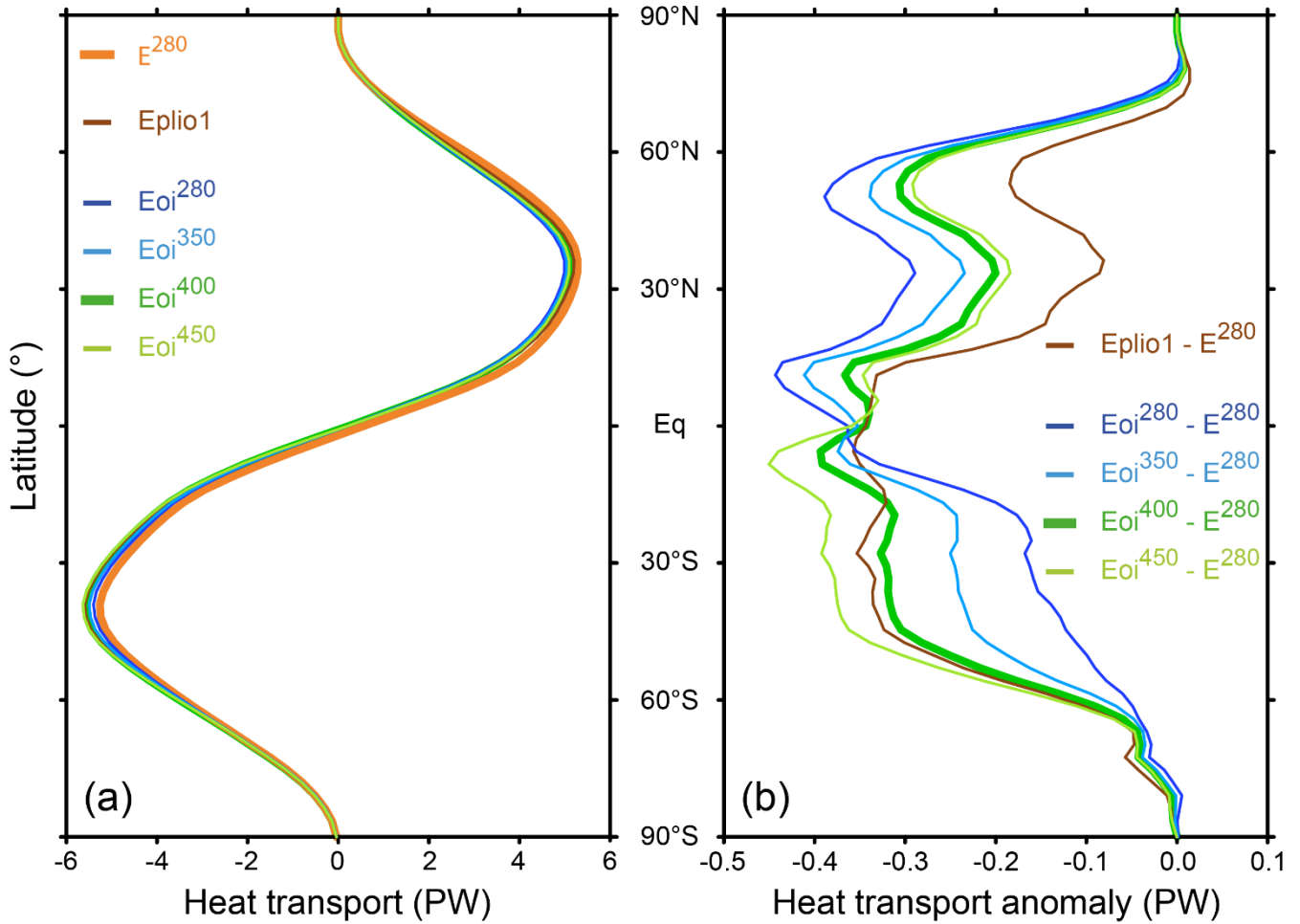
740 Figure 13: (a) The total meridional heat transport in the Pliocene experiments and in E 280 , as calculated from the top-of-atmosphere radiative transport, and (b) the anomaly between the Pliocene experiments and E 280 . The core experiment, Eoi 400 , is shown in bold green.
