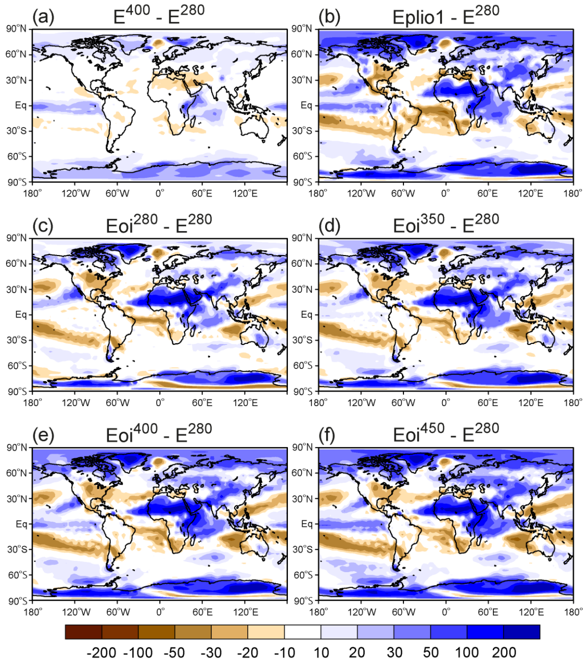
Figure 7: Annual mean precipitation anomaly between six experiments and E^{280} , the Pre-Industrial, as a percentage of E^{280} , eg. 100 \times (E_{oi}^{400} - E^{280}) / E^{280} . For a comparison of PlioMIP1 and PlioMIP2, see (b) and (e). For the individual effects of CO_2 and Pliocene boundary conditions, see (a) and (c), respectively.
