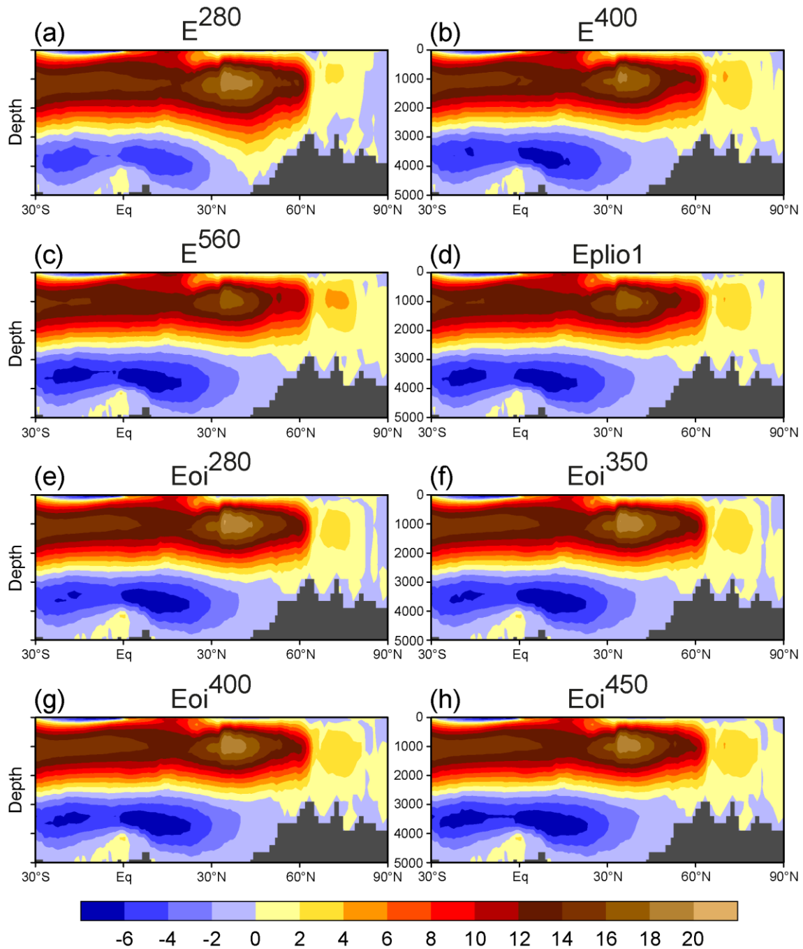
Figure 11: Streamfunction of the Atlantic meridional overturning circulation, averaged over the last 500 years. For a comparison of PlioMIP1 and PlioMIP2, see (d) and (g). For the individual effects of CO 2 and Pliocene boundary conditions, see (b) and (e), respectively.
