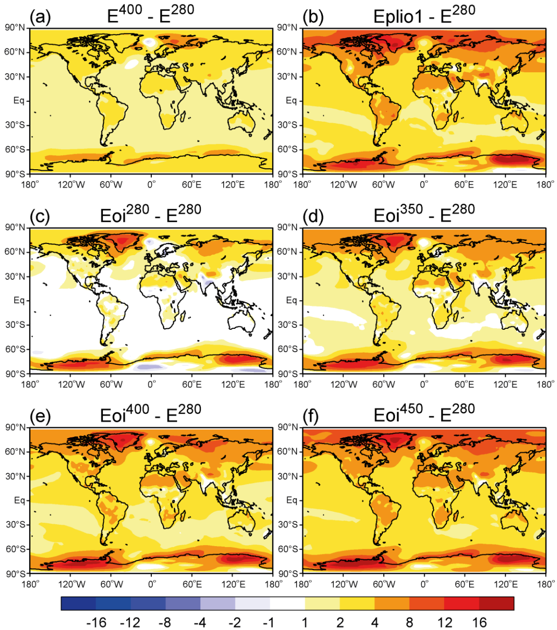
Figure 3: Annual mean surface air temperature anomaly between six experiments and E^{280} , the Pre-Industrial. For a comparison of PlioMIP1 and PlioMIP2, see (b) and (e). For the individual effects of \text{CO}_2 and Pliocene boundary conditions, see (a) and (c), respectively.
