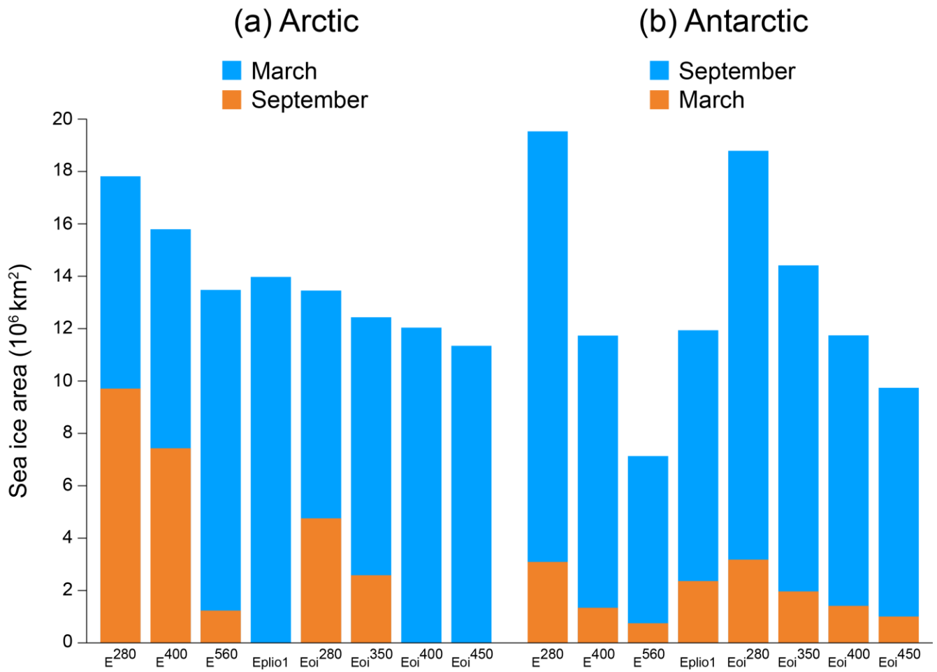
720 Figure 8: Total surface area of sea ice in each polar region during March and September.
