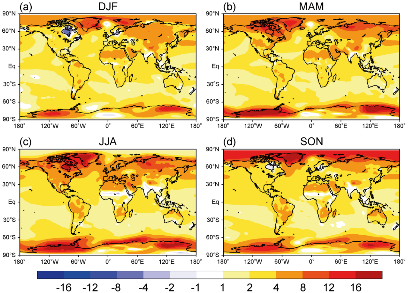
710 Figure 5: Seasonal surface air temperature anomaly between E_{oi}^{400} and E^{280} for December-February (DJF), March-May (MAM), June-August (JJA) and September-November (SON).
