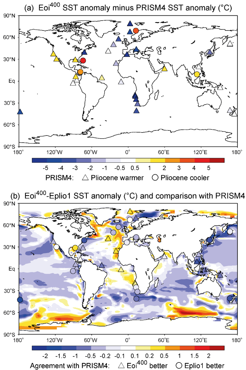
765 Figure 17: (a) Comparison of annual mean model SST anomalies and PRISM4 proxy data SST anomalies. Blue (red) indicates that model SST anomalies are smaller (greater) than those of proxy data. The shape of the symbols indicates whether proxy data suggests higher (triangle) SST in the Pliocene or lower (circle). (b) The difference between PlioMIP1 and PlioMIP2 SST. The shape of the symbols at PRISM4 locations indicates whether PlioMIP2 agrees better with proxy data (triangle) or whether PlioMIP1 agrees better (circle).
