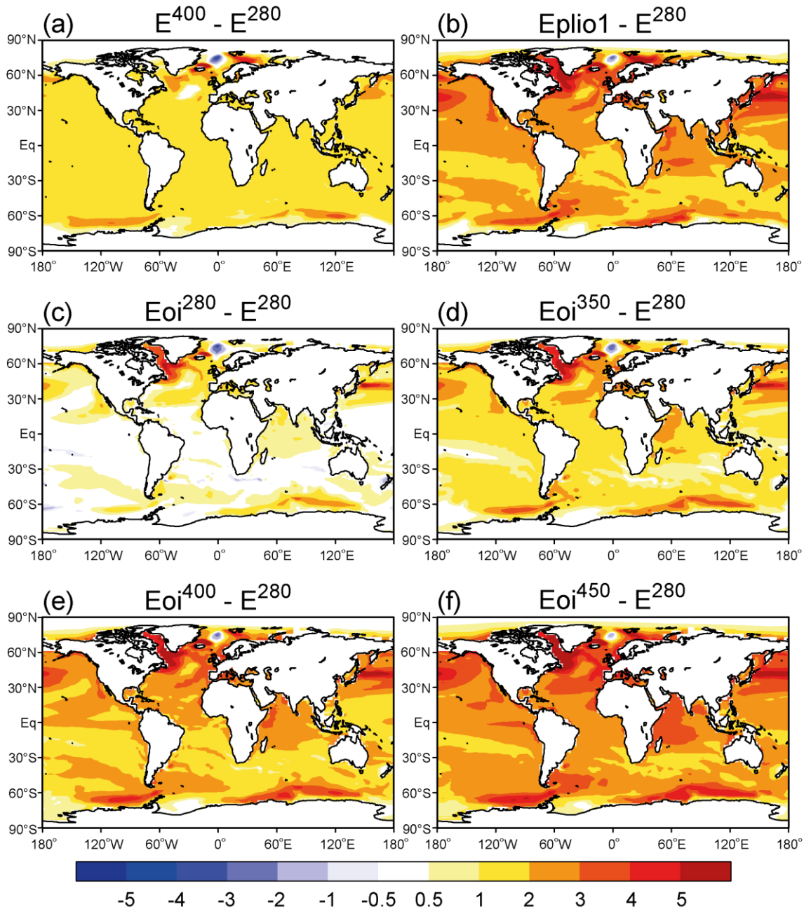
Figure 6: Annual mean sea surface temperature anomaly between six experiments and E^{280} , the Pre-Industrial. For a comparison of PlioMIP1 and PlioMIP2, see (b) and (e). For the individual effects of \text{CO}_2 and Pliocene boundary conditions, see (a) and (c), respectively.
