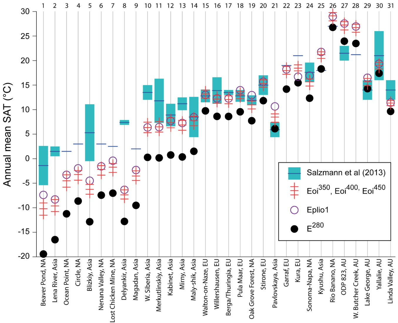
750 Figure 15: Comparison of annual mean surface air temperatures derived from terrestrial proxy data (Table S3a of Salzmman et al., 2013) and those from model experiments. Proxy data are indicated by the dark blue line and the uncertainty range by light blue. The three red marks represent, from top to bottom, E^{450} , E^{400} and E^{350} . Abbreviations used at the bottom of the figure: NA (North America), EU (Europe), AU (Australia).
