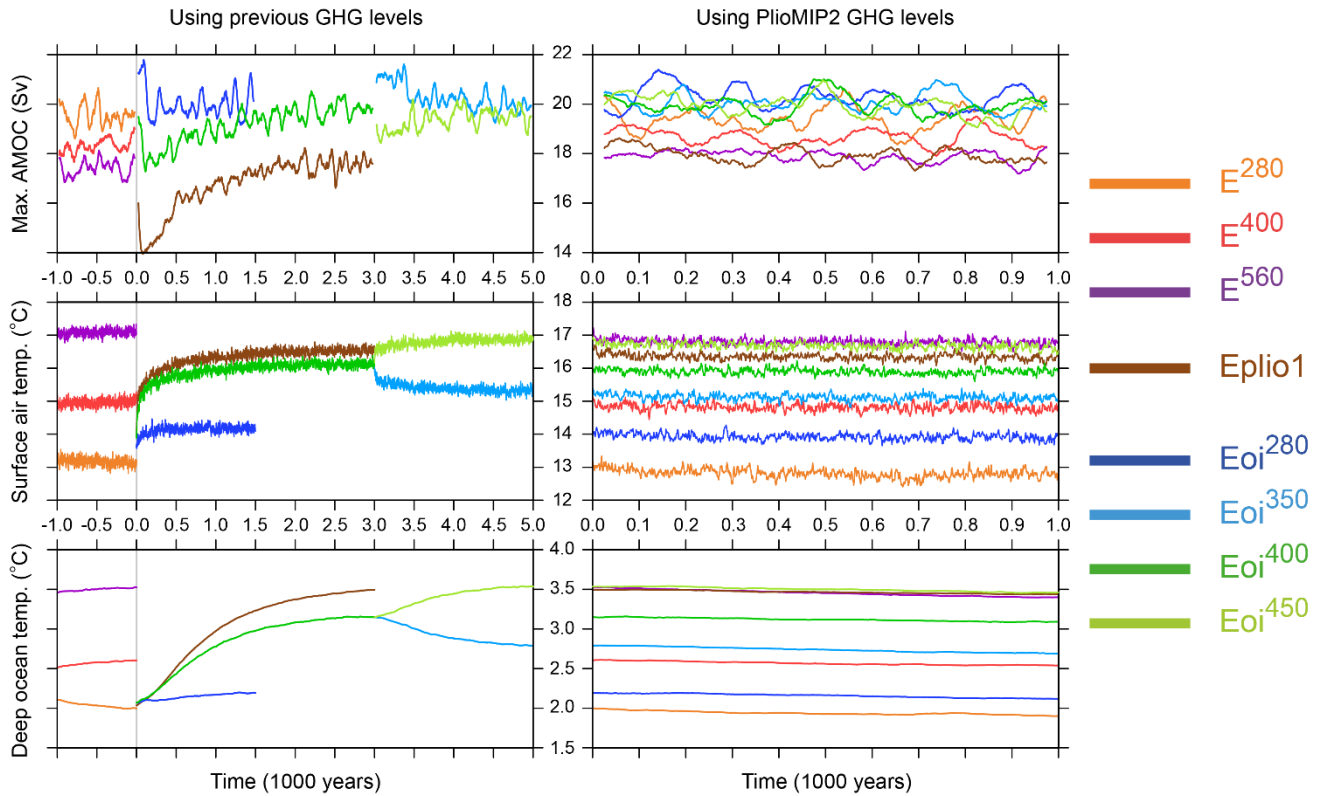
700 Figure 2: Time series of the AMOC index (top), globally averaged surface air temperature (middle) and global ocean temperature below depths of 1900m (bottom). A 51-year moving average has been applied to the AMOC index time series. The subfigures on the left depict the initial stages of the experiments during which greenhouse gas levels are set to previous, PlioMIP1 values, while the subfigures on the right depict the final 1000 years of the integration during which greenhouse gas levels are consistent with those specified in PlioMIP2.
