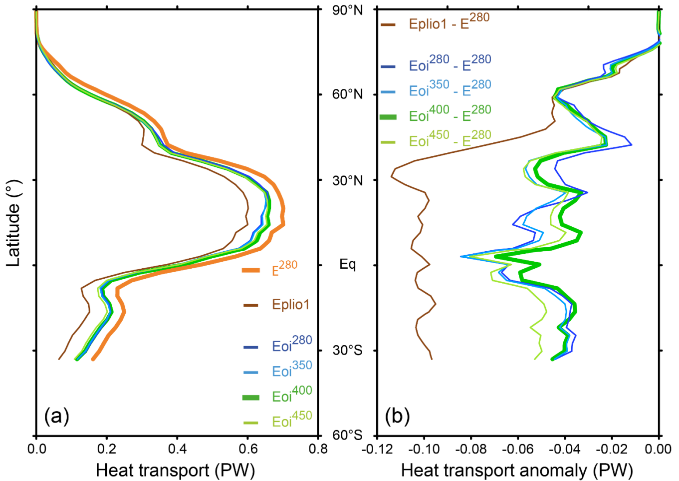
Figure 12: (a) The Atlantic Ocean meridional heat transport in the Pliocene experiments and in E^{280} and (b) the anomaly between the Pliocene experiments and E^{280} . The core experiment, Eoi^{400} , is shown in bold green.
