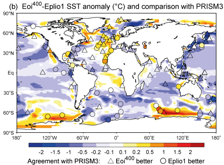
Figure 16: (a) Comparison of annual mean model SST anomalies and PRISM3 proxy data SST anomalies. Blue (red) indicates that model SST anomalies are smaller (greater) than those of proxy data. The shape of the symbols indicates whether proxy data suggests higher (triangle) SST in the Pliocene or lower (circle). (b) The difference between PlioMIP1 and PlioMIP2 SST. The shape of the symbols at PRISM3 locations indicates whether PlioMIP2 agrees better with proxy data (triangle) or whether PlioMIP1 agrees better (circle).
